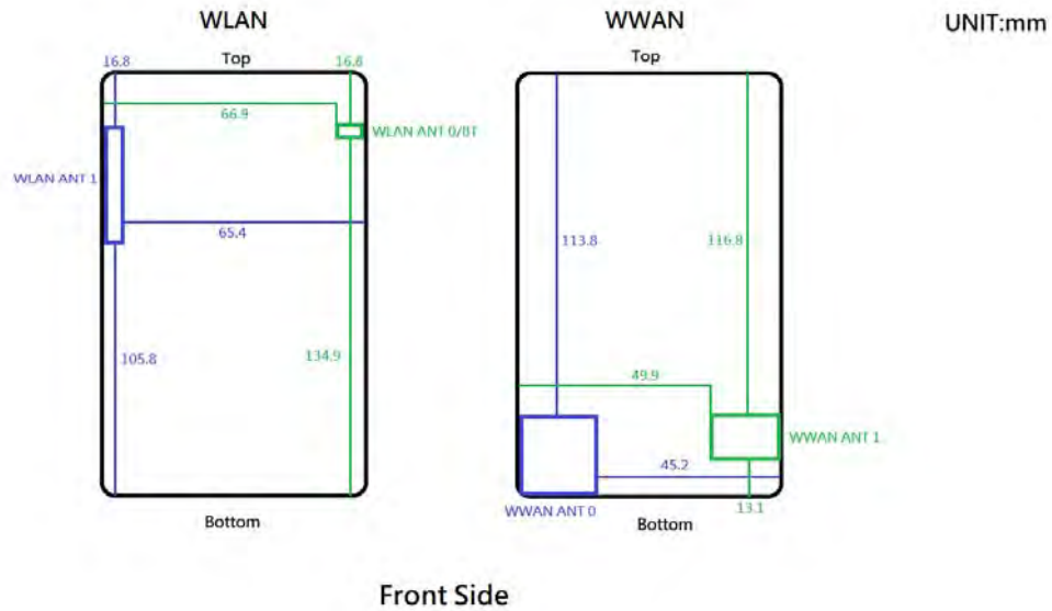
Fig.23 Antenna position of EUT
