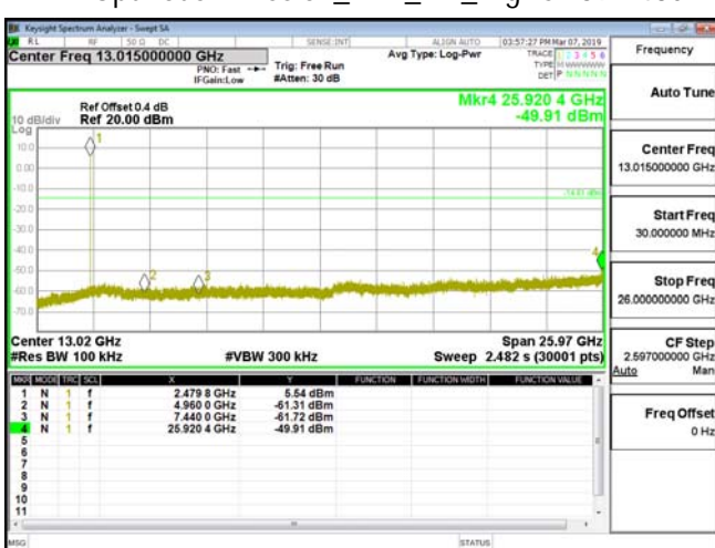
Spurious Emission_BLE_1M_HighCH39-2480
