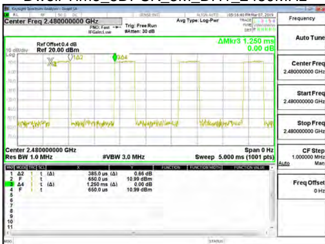
Dwell Time_8DPSK_3M_DH1_2480MHz
