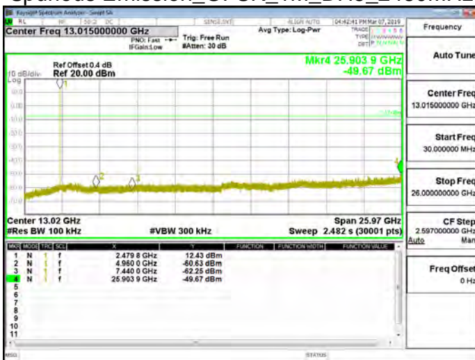
Spurious Emission_GFSK_1M_DH5_2480MHz
