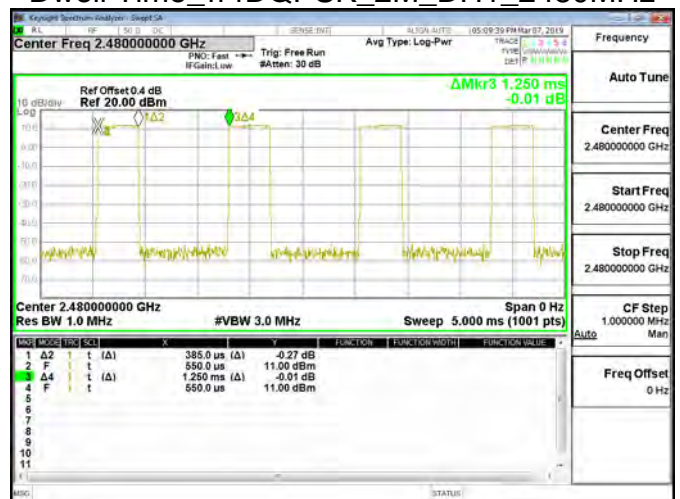
Dwell Time_π4DQPSK_2M_DH1_2480MHz
