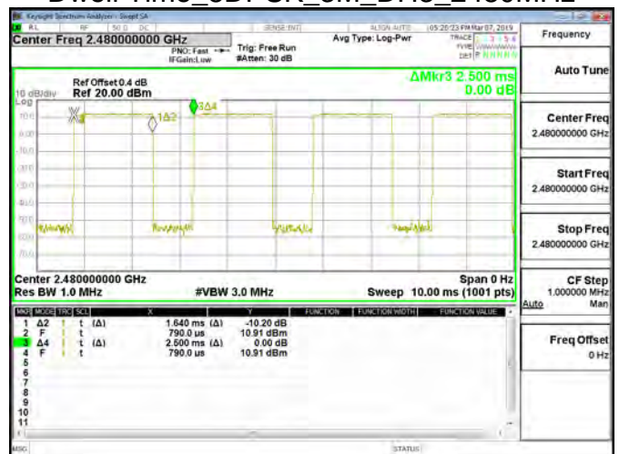
Dwell Time_8DPSK_3M_DH3_2480MHz
