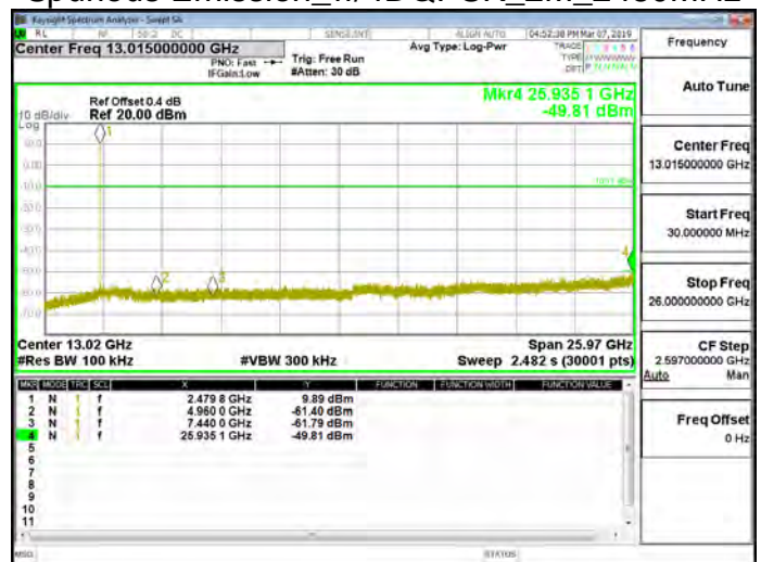
Spurious Emission_π/4DQPSK_2M_2480MHz
