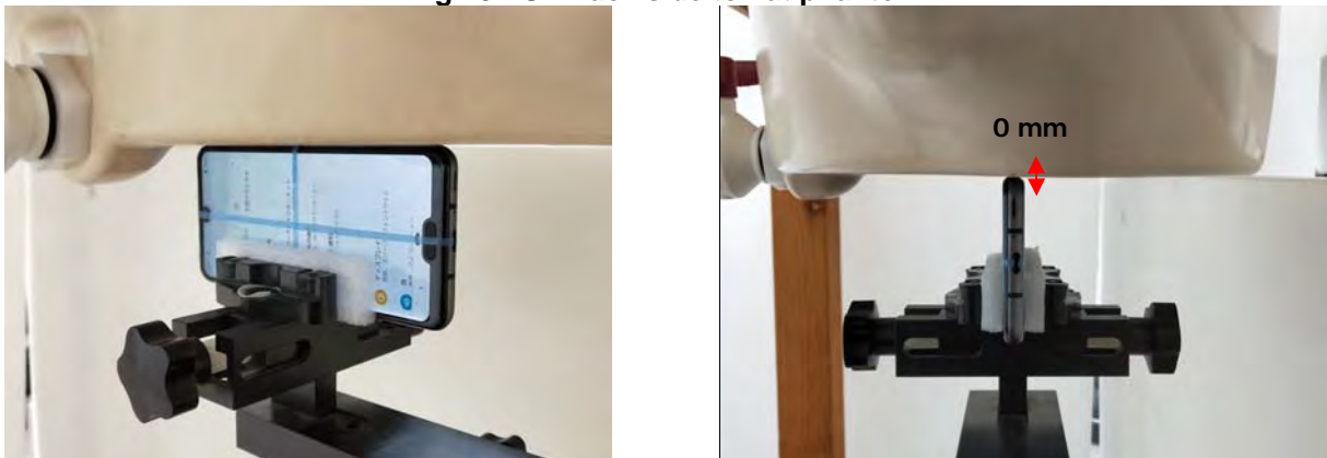
Fig.17 EUT Right side to flat phantom
