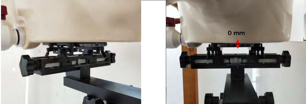
Fig.15 EUT Front side to flat phantom
