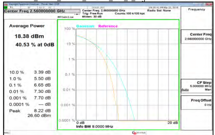
LTE_Band7_20MHz_64QAM_100_0_HighCH21350-2560
