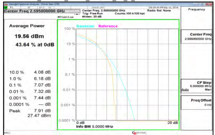
LTE_Band38_5MHz_64QAM_25_0_MidCH38000-2595
