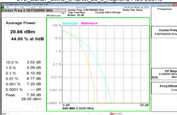
LTE_Band7_5MHz_64QAM_25_0_HighCH21425-2567.5
