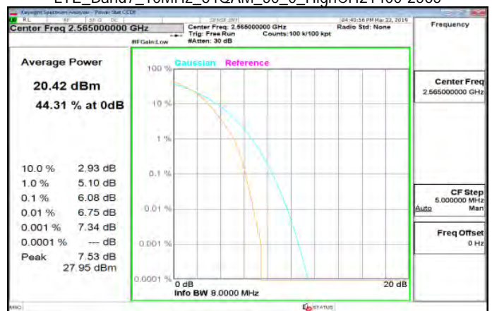
LTE_Band7_10MHz_64QAM_50_0_HighCH21400-2565
