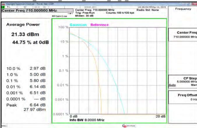
LTE_Band17_10MHz_64QAM_50_0_MidCH23790-710
