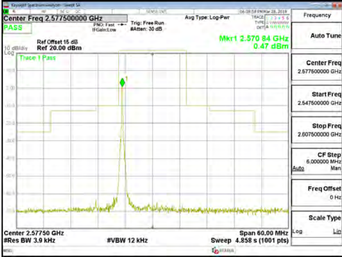
Band38_15MHz_64QAM_1_0_CH38000
