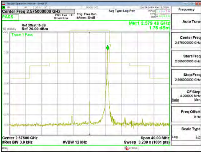
Band38_10MHz_64QAM_1_49_CH38000
