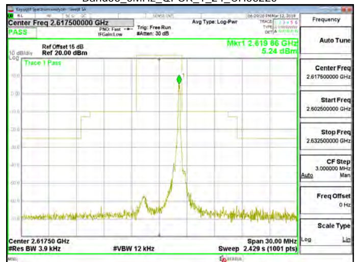
Band38_5MHz_QPSK_1_24_CH38225
