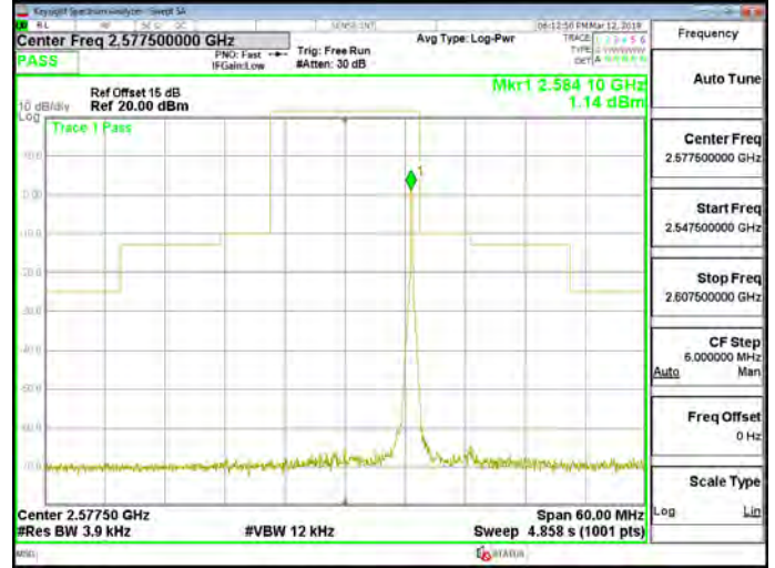
Band38_15MHz_64QAM_1_74_CH38000
