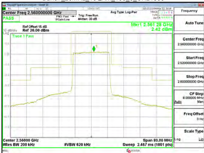
Band7_20MHz_16QAM_100_0_CH21350
