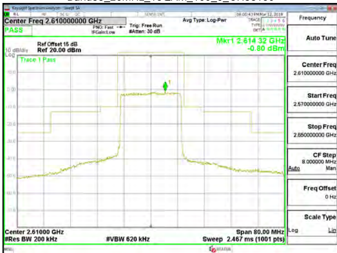
Band38_20MHz_16QAM_100_0_CH38150
