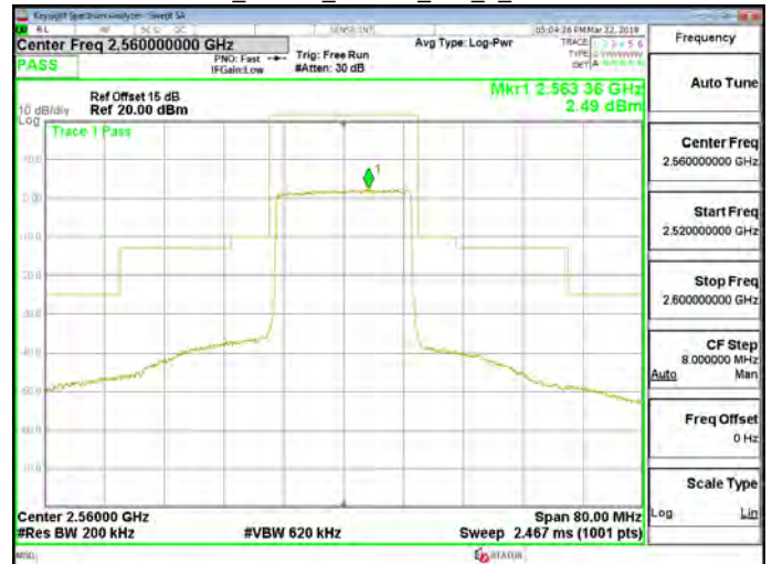
Band7_20MHz_64QAM_100_0_CH21350
