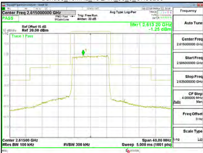
Band38_10MHz_16QAM_50_0_CH38200
