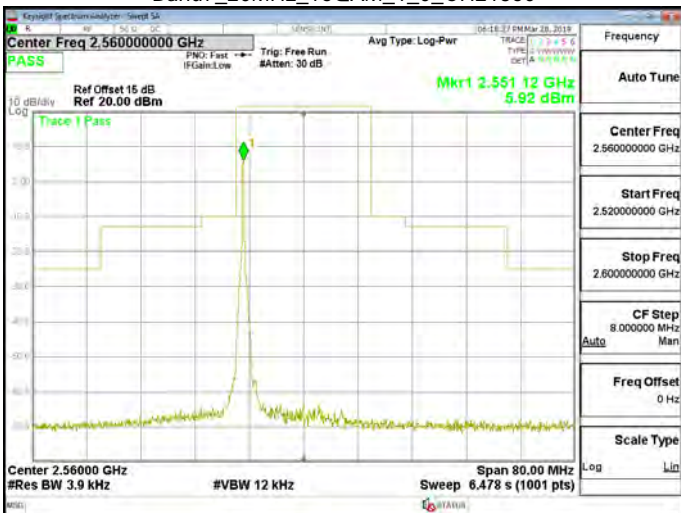
Band7_20MHz_16QAM_1_0_CH21350
