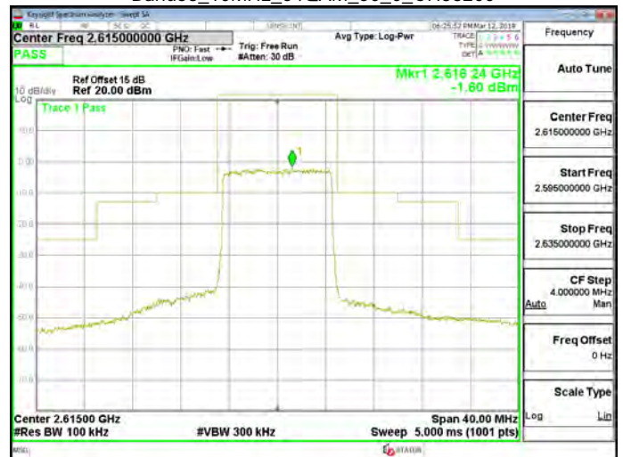
Band38_10MHz_64QAM_50_0_CH38200
