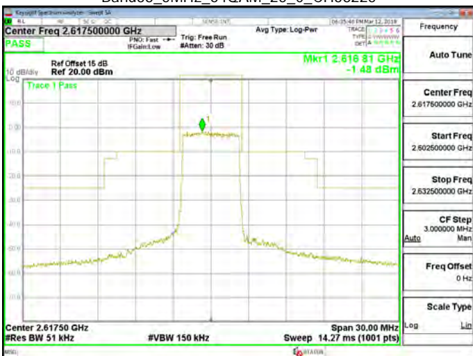
Band38_5MHz_64QAM_25_0_CH38225
