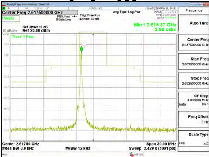
Band38_5MHz_64QAM_1_0_CH38225
