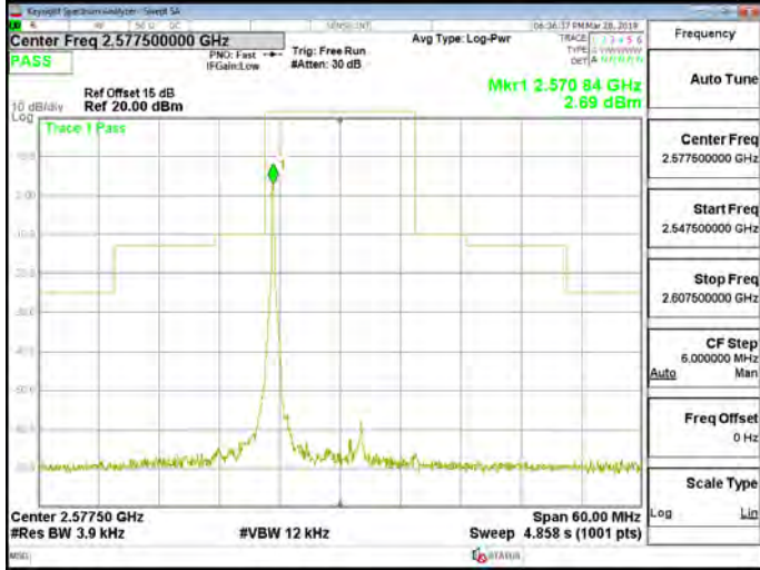
Band38_15MHz_QPSK_1_0_CH38000
