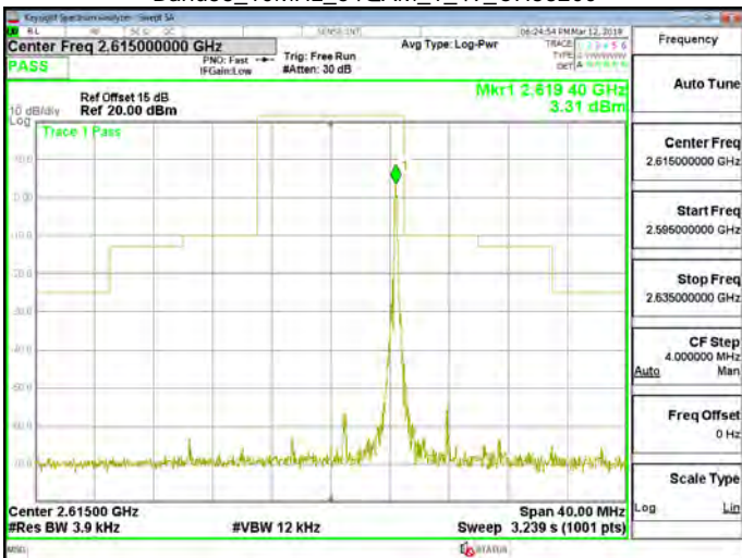
Band38_10MHz_64QAM_1_49_CH38200
