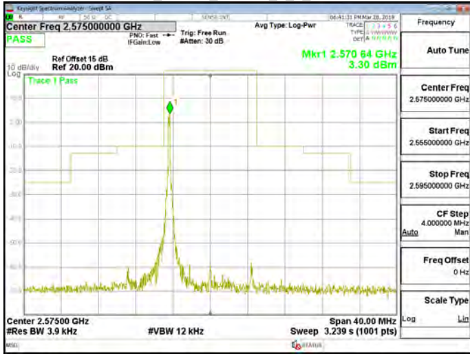
Band38_10MHz_16QAM_1_0_CH38000
