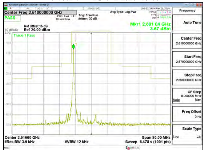
Band38_20MHz_QPSK_1_0_CH38150
