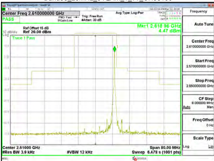
Band38_20MHz_64QAM_1_99_CH38150
