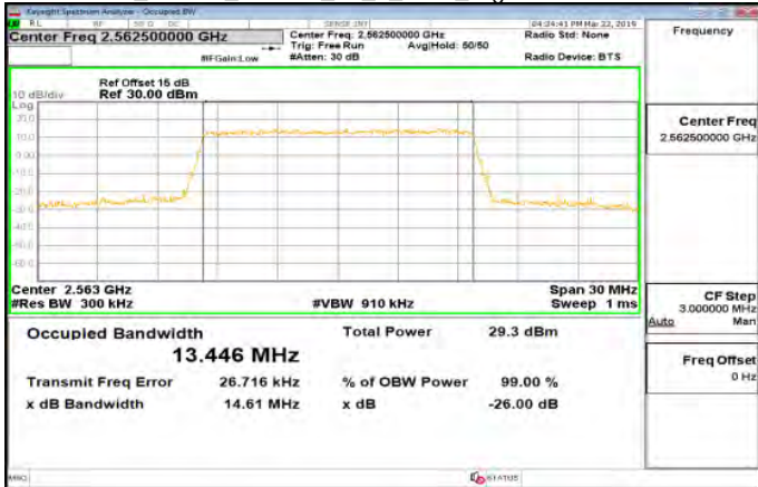
Band7_15MHz_16QAM_75_0_Main_HighCH21375-2562.5
