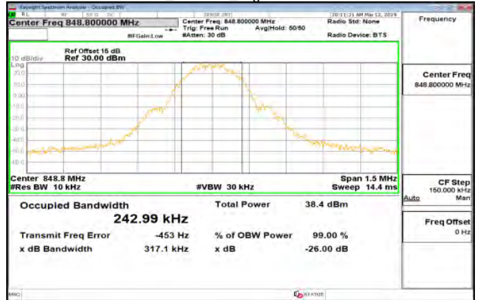
GPRS_850MHz_HighCH251-848.8
