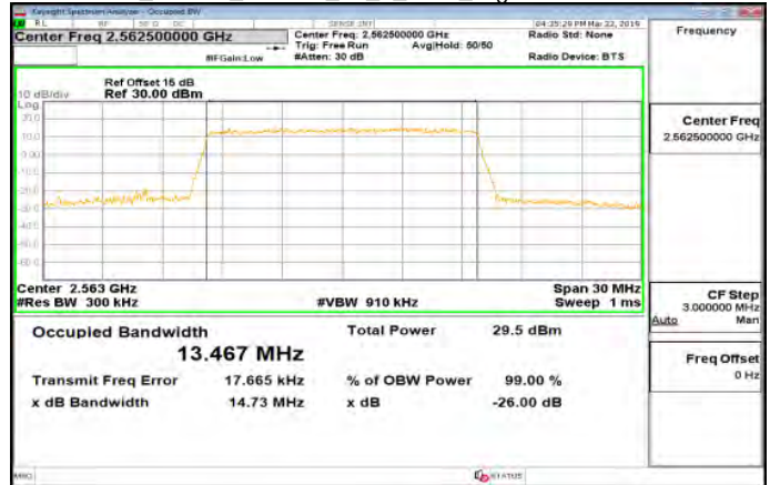
Band7_15MHz_64QAM_75_0_Main_HighCH21375-2562.5
