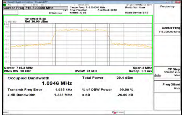
Band12_1_4MHz_64QAM_6_0_Main_HighCH23173-715.3
