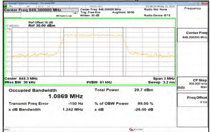
Band5_1_4MHz_QPSK_6_0_Main_HighCH20643-848.3
