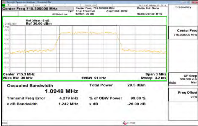
Band12_1_4MHz_16QAM_6_0_Main_HighCH23173-715.3
