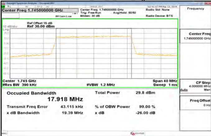
Band4_20MHz_64QAM_100_0_Main_HighCH20300-1745
