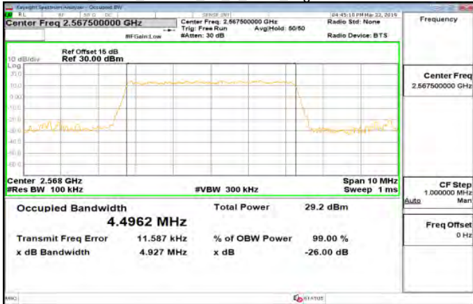
Band7_5MHz_16QAM_25_0_Main_HighCH21425-2567.5
