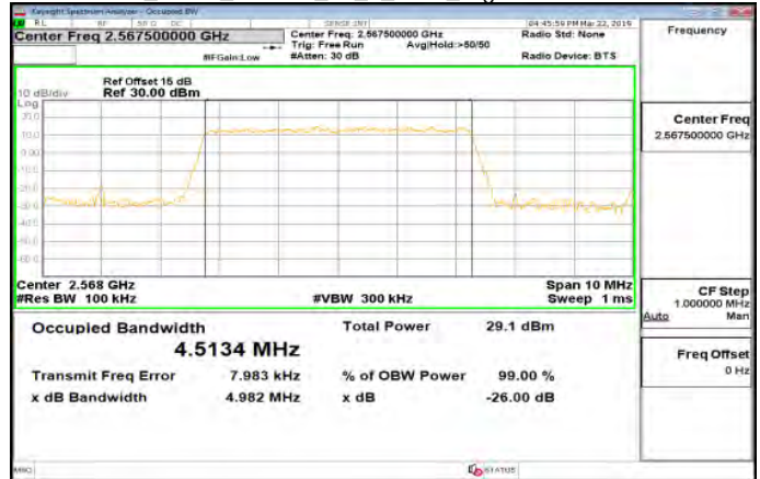
Band7_5MHz_64QAM_25_0_Main_HighCH21425-2567.5
