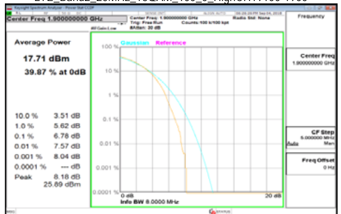
LTE_Band2_20MHz_16QAM_100_0_HighCH19100-1900
