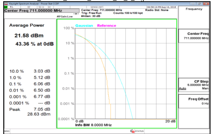
LTE_Band17_10MHz_16QAM_50_0_HighCH23800-711
