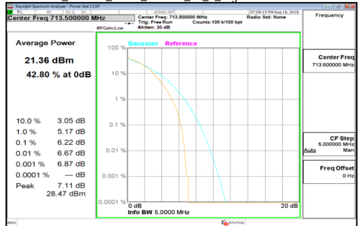
LTE_Band17_5MHz_16QAM_25_0_HighCH23825-713.5
