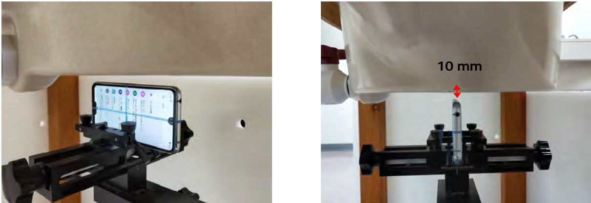
Fig.14 EUT Left side to flat phantom
