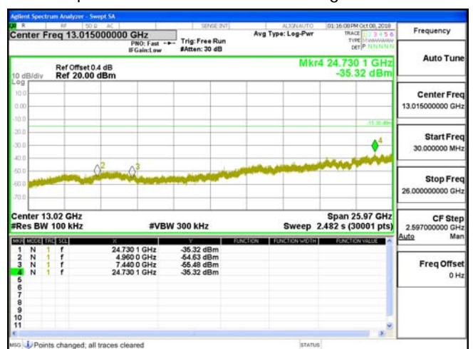
Spurious Emission_BLE_2M_HighCH39-2480
