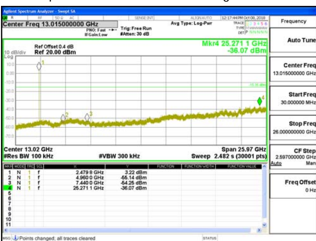
Spurious Emission_BLE_1M_HighCH39-2480
