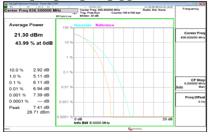
LTE_Band5_10MHz_64QAM_50_0_MidCH20525-836.5
