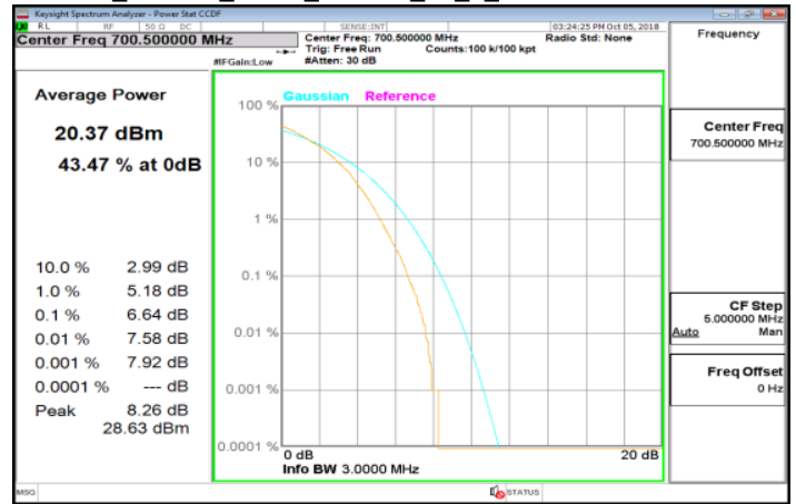
LTE_Band12_3MHz_64QAM_15_0_LowCH23025-700.5
