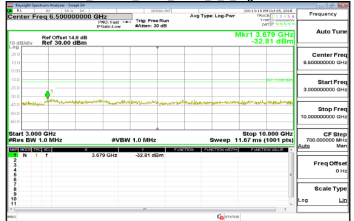
3GHz~10GHz_Band17_5MHz_QPSK_1_0_HighCH23825-713.5
