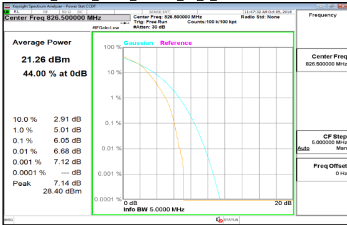
LTE_Band5_5MHz_64QAM_25_0_LowCH20425-826.5
