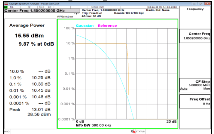
GPRS_1900MHz_LowCH512-1850.2
