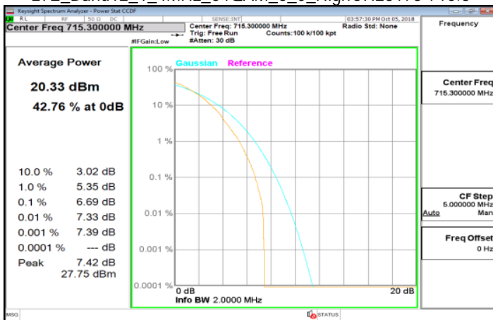
LTE_Band12_1_4MHz_64QAM_6_0_HighCH23173-715.3
