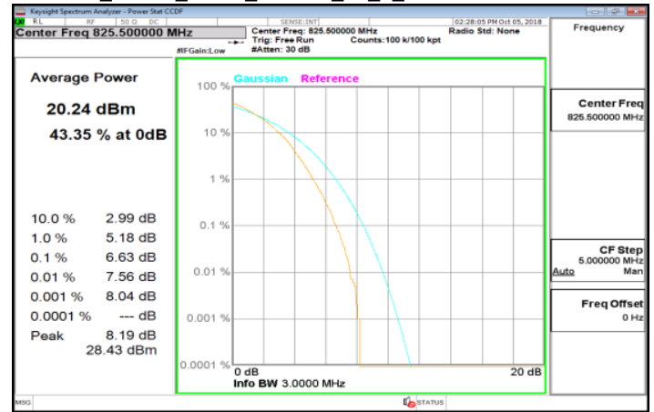
LTE_Band5_3MHz_64QAM_15_0_LowCH20415-825.5
