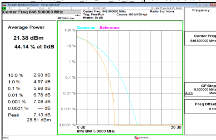
LTE_Band5_5MHz_64QAM_25_0_HighCH20625-846.5
