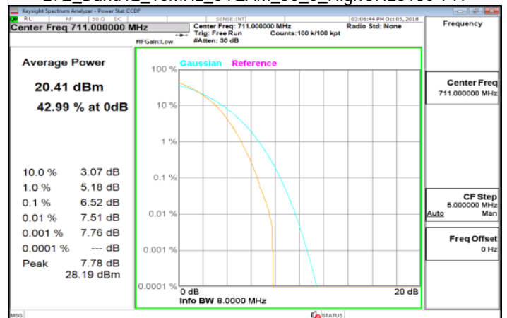
LTE_Band12_10MHz_64QAM_50_0_HighCH23130-711
