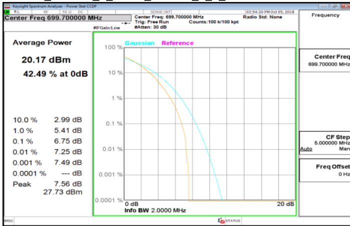
LTE_Band12_1_4MHz_64QAM_6_0_LowCH23017-699.7
