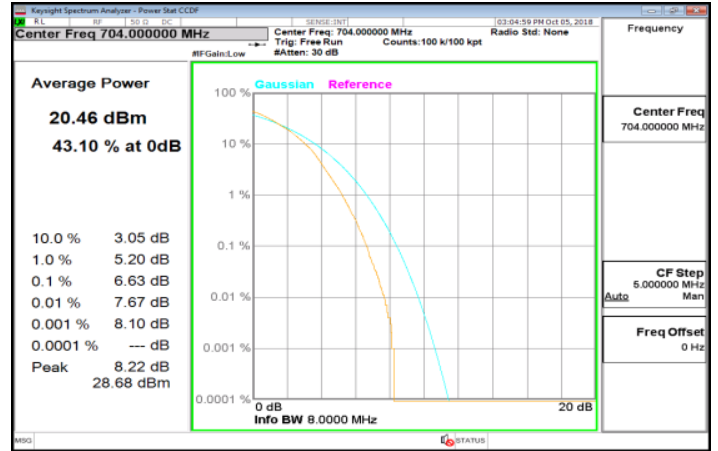
LTE_Band12_10MHz_64QAM_50_0_LowCH23060-704
