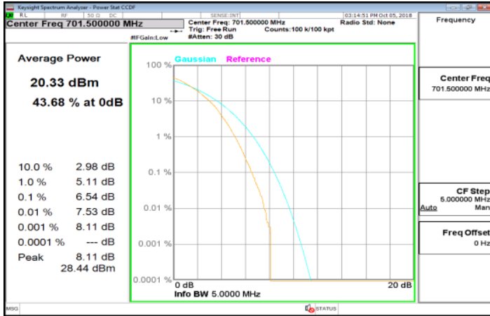
LTE_Band12_5MHz_64QAM_25_0_LowCH23035-701.5
