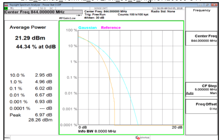
LTE_Band5_10MHz_64QAM_50_0_HighCH20600-844
