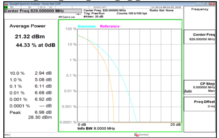
LTE_Band5_10MHz_64QAM_50_0_LowCH20450-829
