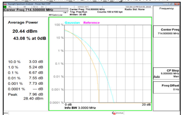
LTE_Band12_3MHz_64QAM_15_0_HighCH23165-714.5
