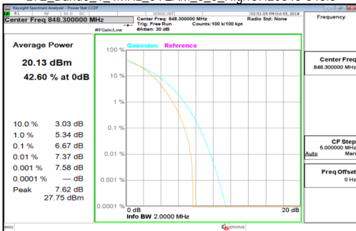
LTE_Band5_1_4MHz_64QAM_6_0_HighCH20643-848.3
