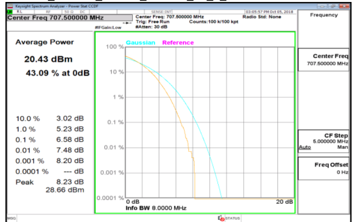
LTE_Band12_10MHz_64QAM_50_0_MidCH23095-707.5
