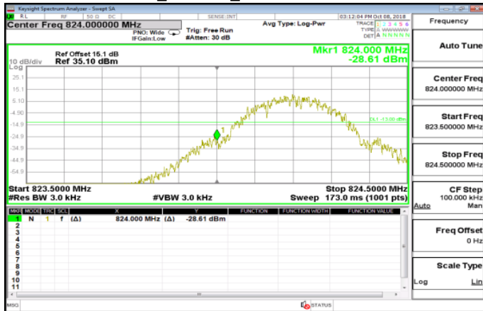
GSM_850MHz_LowCH128-824.2
