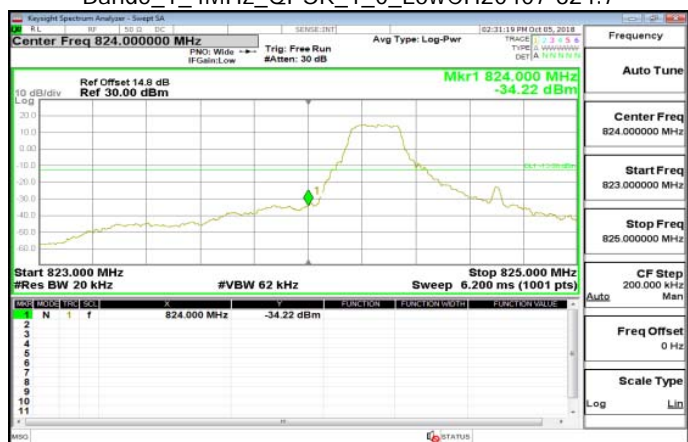
Band5_1_4MHz_QPSK_1_0_LowCH20407-824.7
