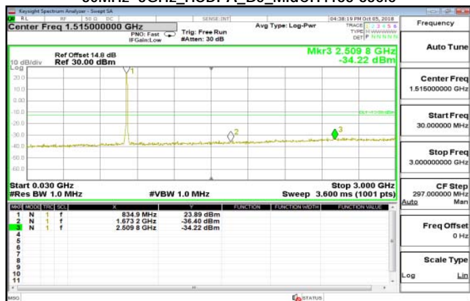
30MHz~3GHz_HSDPA_B5_MidCH4183-836.6
