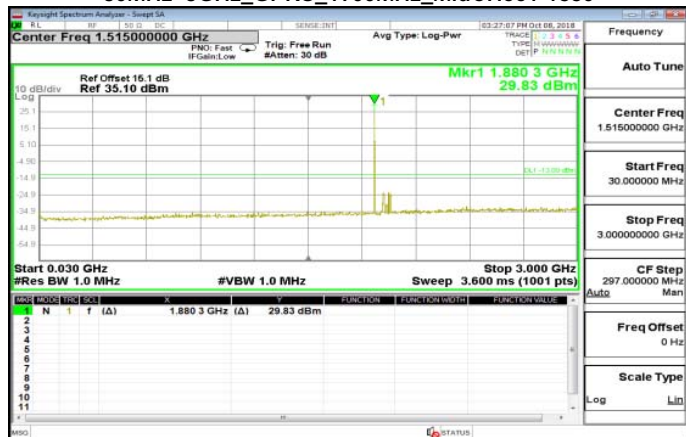
30MHz~3GHz_GPRS_1900MHz_MidCH661-1880
