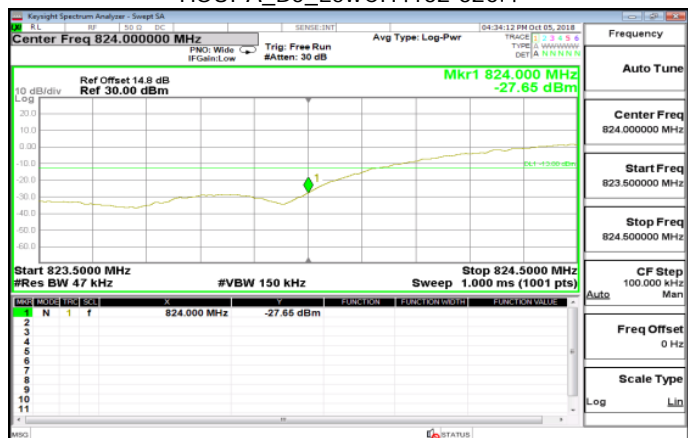
HSUPA_B5_LowCH4132-826.4
