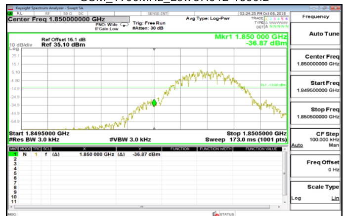
GSM_1900MHz_LowCH512-1850.2
