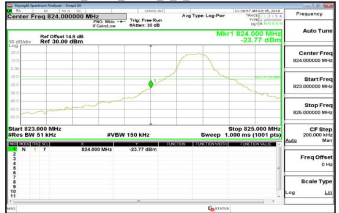
Band5_5MHz_QPSK_1_0_LowCH20425-826.5
