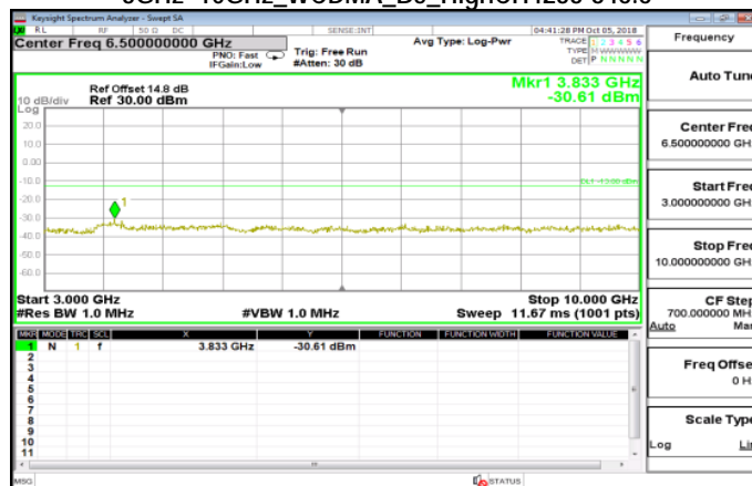
3GHz~10GHz_WCDMA_B5_HighCH4233-846.6
