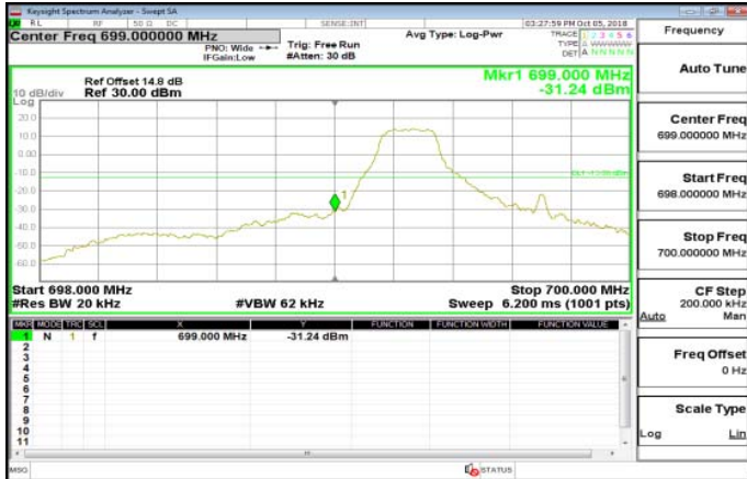
Band12_1_4MHz_QPSK_1_0_LowCH23017-699.7
