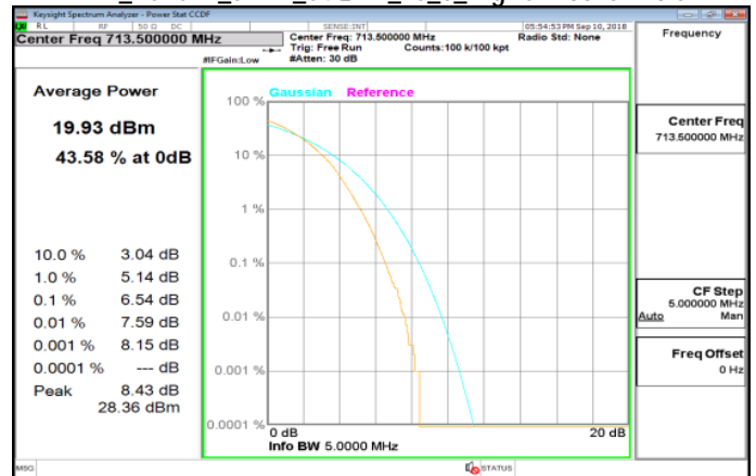
LTE_Band17_5MHz_64QAM_25_0_HighCH23825-713.5
