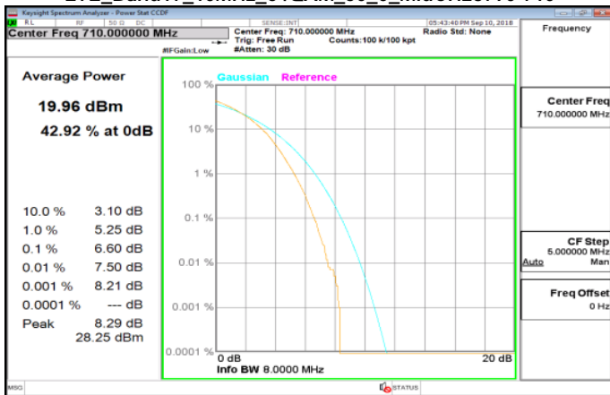
LTE_Band17_10MHz_64QAM_50_0_MidCH23790-710
