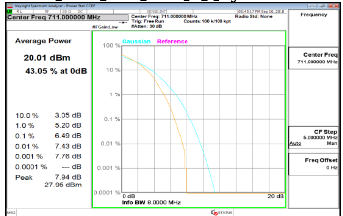
LTE_Band17_10MHz_64QAM_50_0_HighCH23800-711
