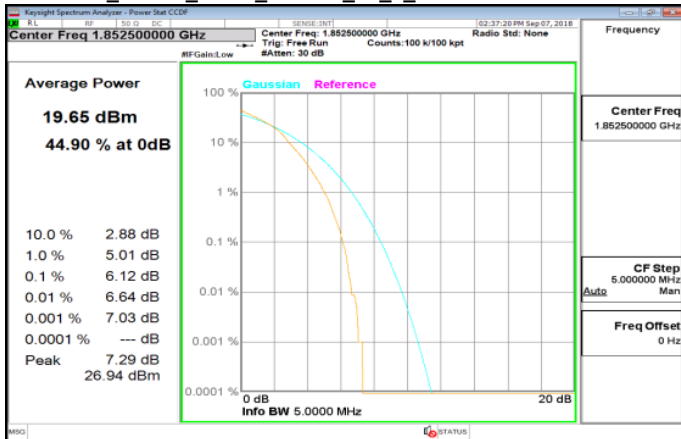
LTE_Band2_5MHz_64QAM_25_0_LowCH18625-1852.5
