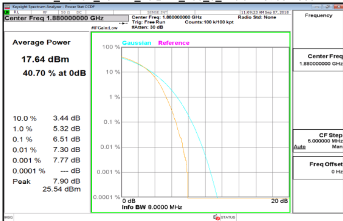
LTE_Band2_20MHz_16QAM_100_0_MidCH18900-1880
