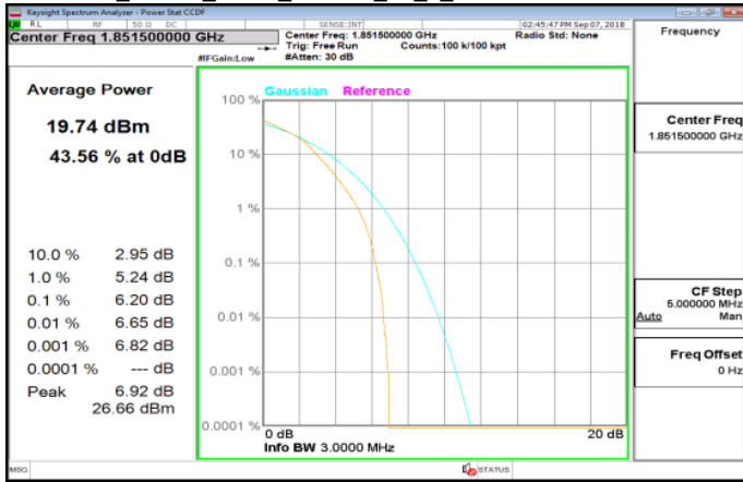
LTE_Band2_3MHz_64QAM_15_0_LowCH18615-1851.5
