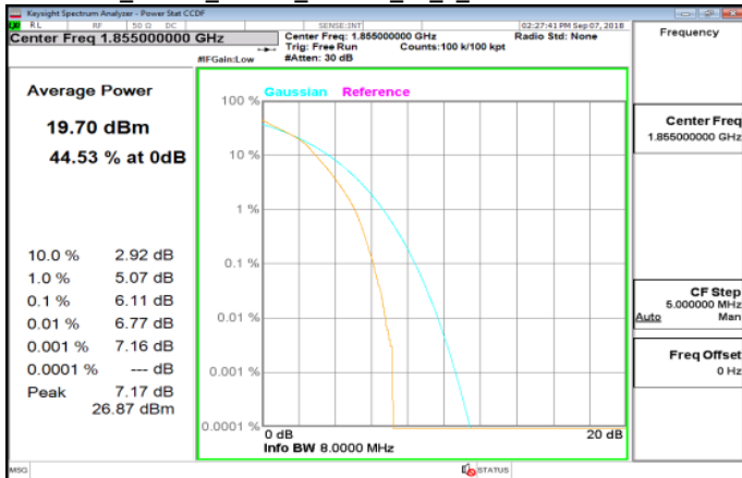
LTE_Band2_10MHz_64QAM_50_0_LowCH18650-1855
