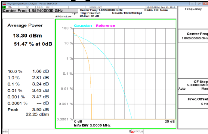
HSUPA_B2_LowCH9262-1852.4
