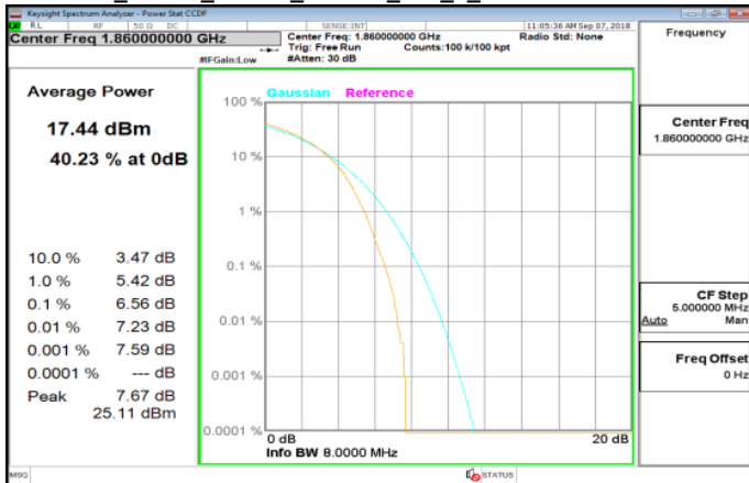
LTE_Band2_20MHz_64QAM_100_0_LowCH18700-1860
