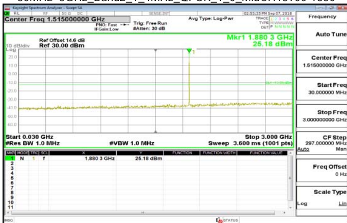
30MHz-3GHz_Band2_1_4MHz_QPSK_1_0_MidCH1890-1880
