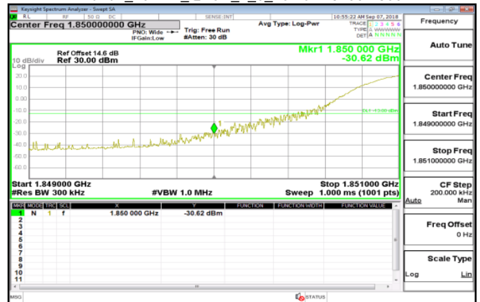
Band2_20MHz_QPSK_1_0_LowCH18700-1860
