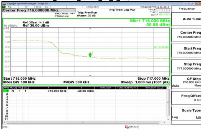
Band17_10MHz_QPSK_1_49\High CH23800-711
