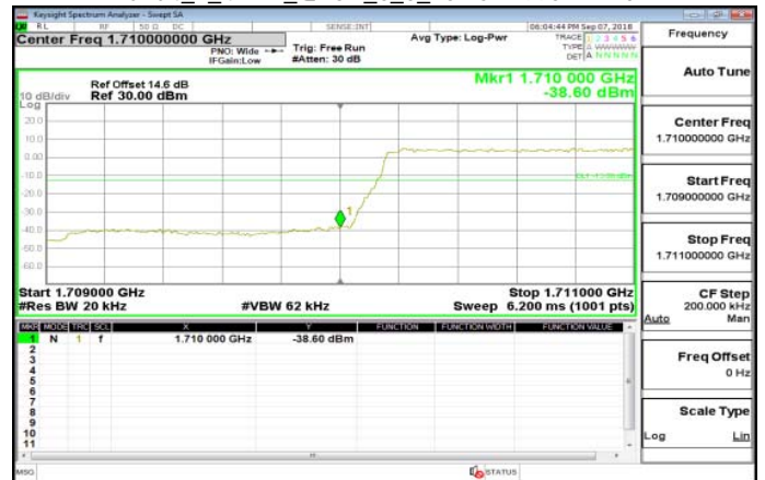
Band4_1_4MHz_QPSK_6_0_LowCH19957-1710.7
