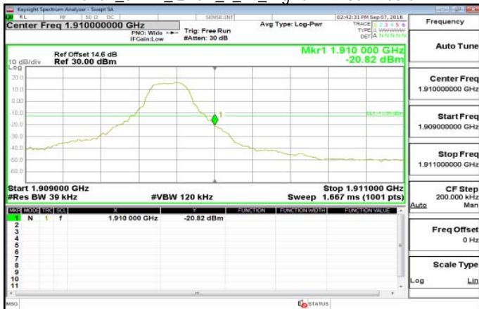
Band2_3MHz_QPSK_1_14_HighCH19185-1908.5
