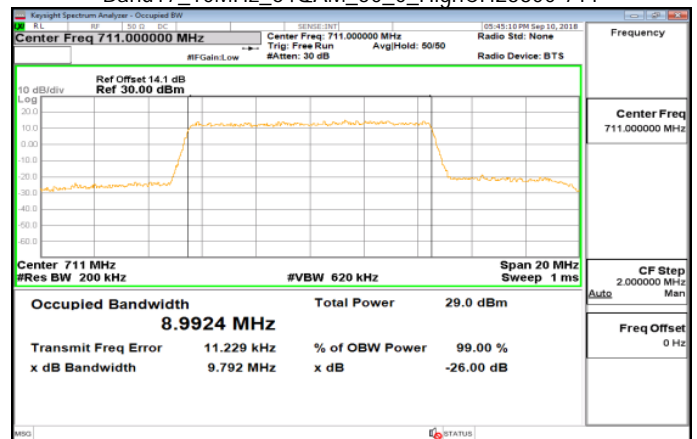
Band17_10MHz_64QAM_50_0_HighCH23800-711
