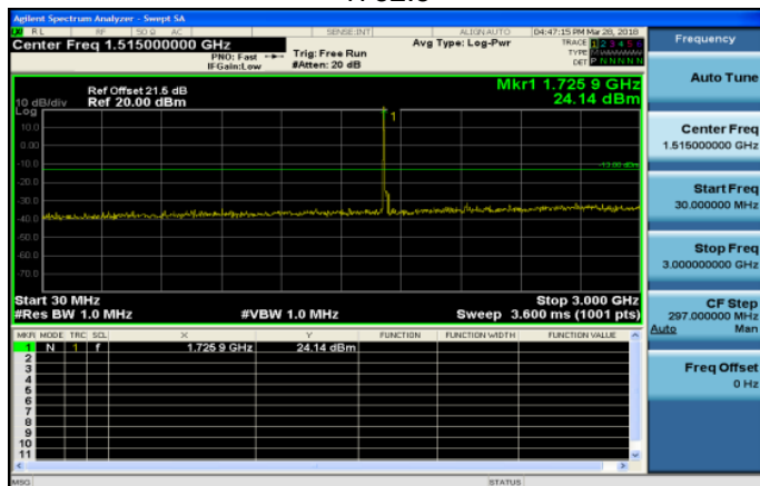
30MHz~3GHz_Band4_15MHz_QPSK_1_0_MidCH20175-1732.5
