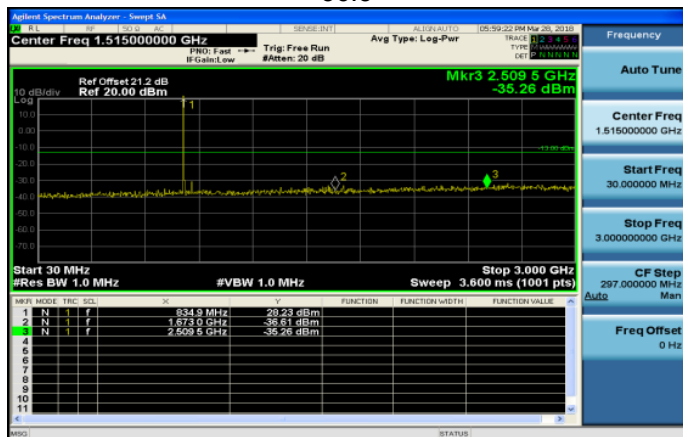
30MHz~3GHz_Band5_3MHz_QPSK_1_0_MidCH20525-8 36.5
