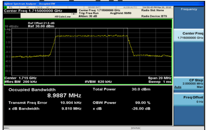
Band4 10MHz QPSK 50 0 LowCH20000-1715
