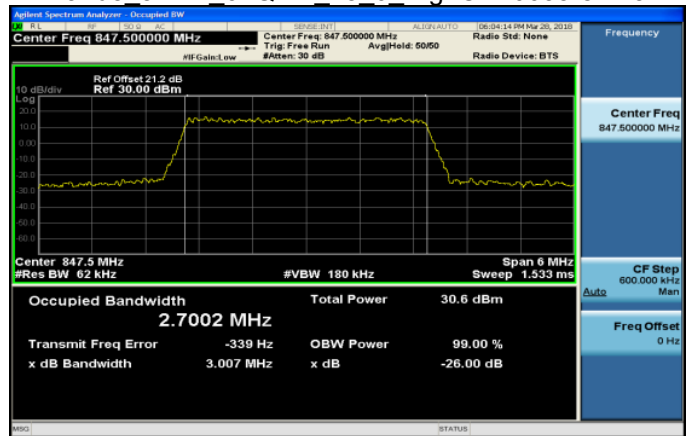
Band5 3MHz 64QAM 15_0 HighCH20635-847.5
