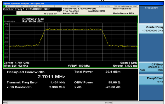
Band4 3MHz 64QAM 15 0 HighCH20385-1753.5
