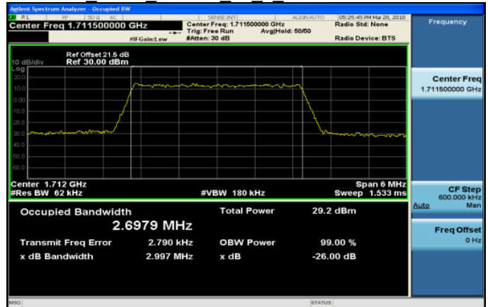
Band4 3MHz 64QAM 15 0 LowCH19965-1711.5
