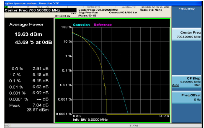
LTE_Band12_3MHz_64QAM_15_0_LowCH23025-700.5
