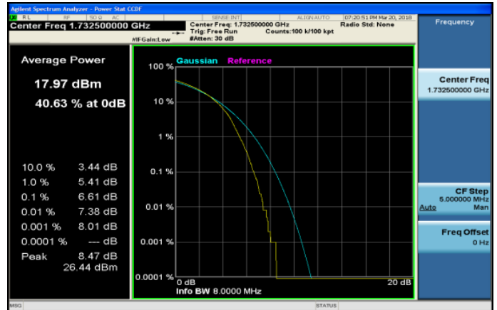
LTE_Band4_20MHz_64QAM_100_0_MidCH20175-1732.5
