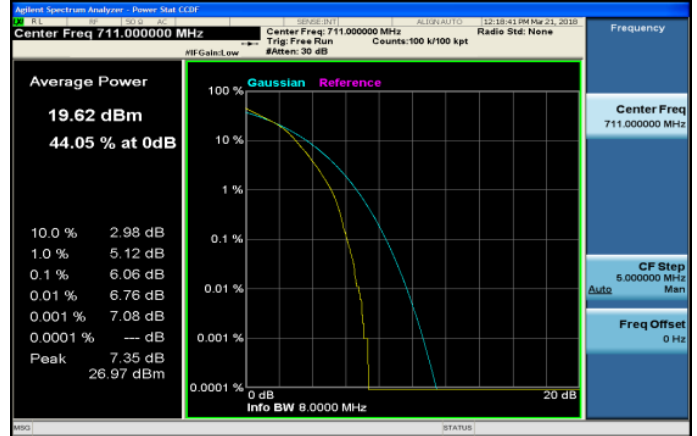
LTE_Band17_10MHz_64QAM_50_0_HighCH23800-711
