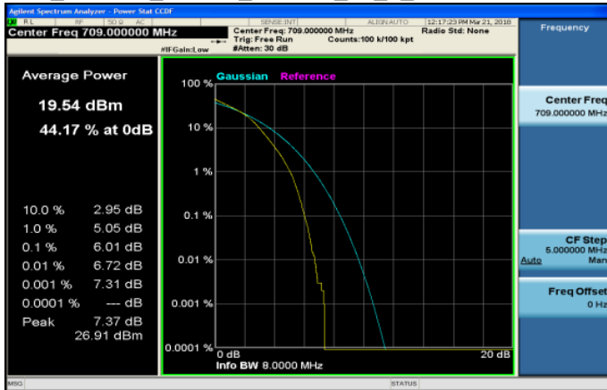
LTE_Band17_10MHz_64QAM_50_0_LowCH23780-709
