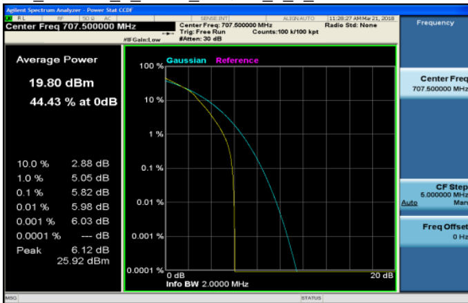
LTE_Band12_1_4MHz_64QAM_6_0_MidCH23095-707.5
