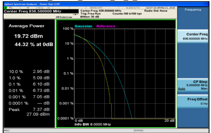
LTE_Band5_10MHz_64QAM_50_0_MidCH20525-836.5
