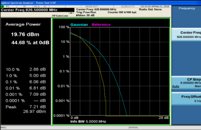
LTE_Band5_5MHz_64QAM_25_0_LowCH20425-826.5
