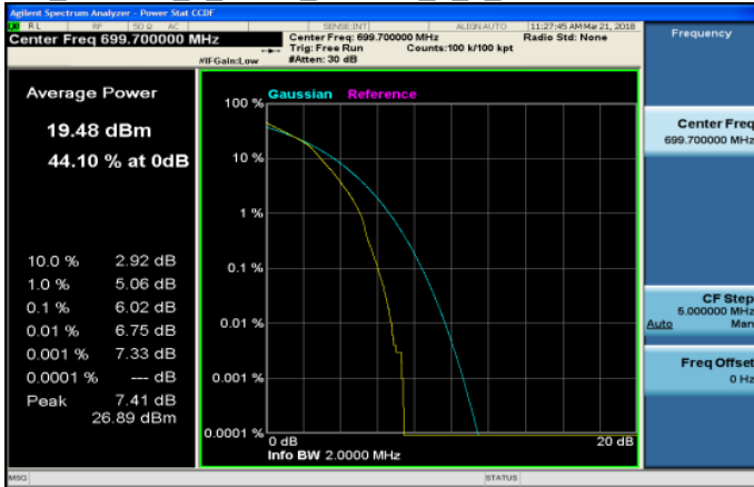
LTE_Band12_1_4MHz_64QAM_6_0_LowCH23017-699.7
