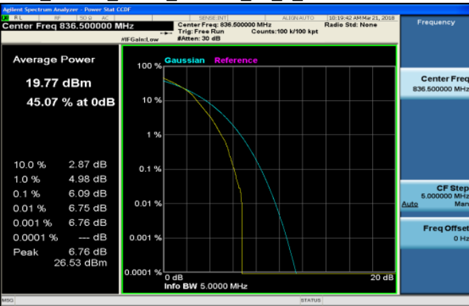
LTE_Band5_5MHz_64QAM_25_0_MidCH20525-836.5
