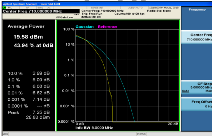
LTE_Band17_10MHz_64QAM_50_0_MidCH23790-710
