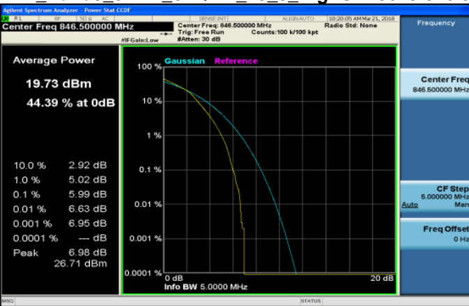
LTE_Band5_5MHz_64QAM_25_0_HighCH20625-846.5
