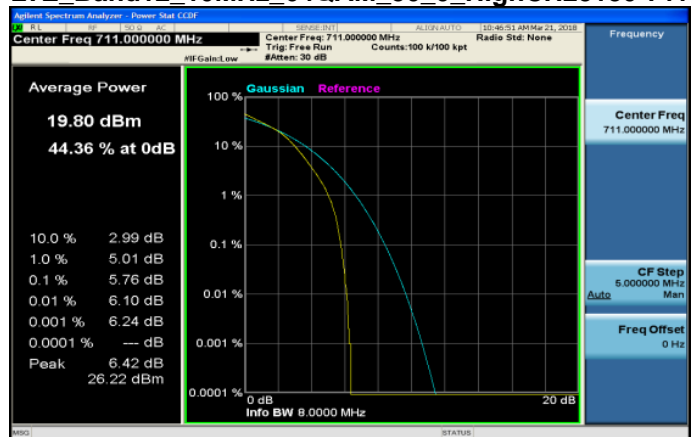
LTE_Band12_10MHz_64QAM_50_0_HighCH23130-711
