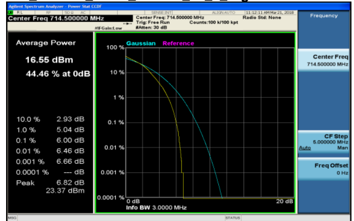
LTE_Band12_3MHz_64QAM_15_0_HighCH23165-714.5
