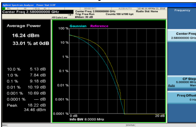
LTE_Band38_20MHz_64QAM_100_0_LowCH37850-258 0
