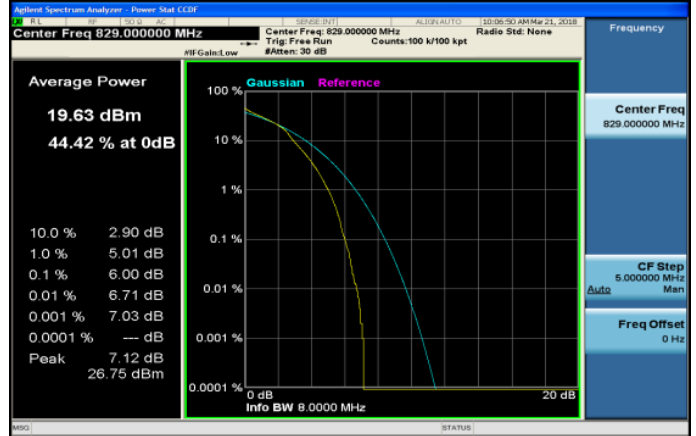
LTE_Band5_10MHz_64QAM_50_0_LowCH20450-829
