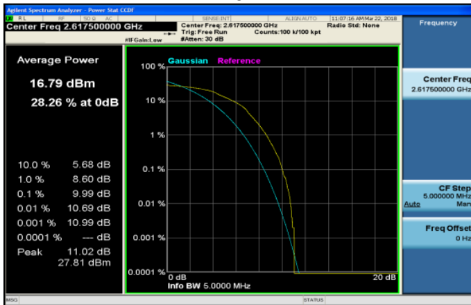
LTE_Band38_5MHz_64QAM_25_0_HighCH38225-2617. 5
