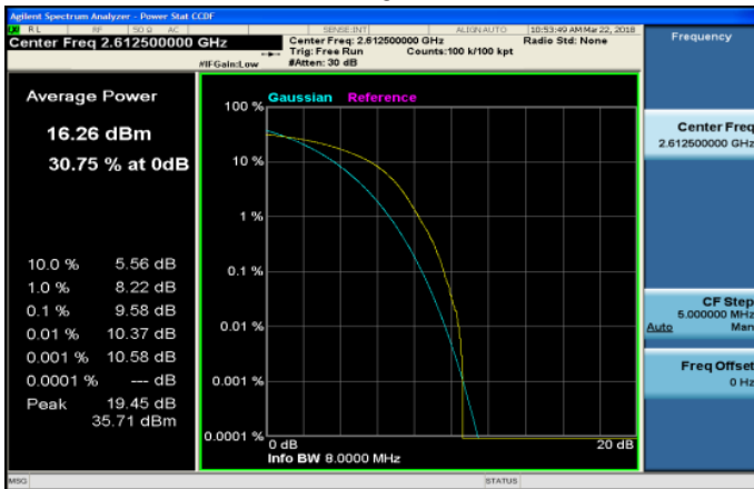
LTE_Band38_15MHz_64QAM_75_0_HighCH38175-2612 5
