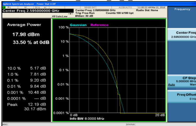
LTE_Band38_10MHz_64QAM_50_0_MidCH38000-2595
