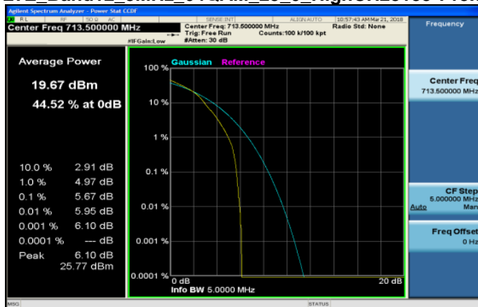
LTE_Band12_5MHz_64QAM_25_0_HighCH23155-713.5
