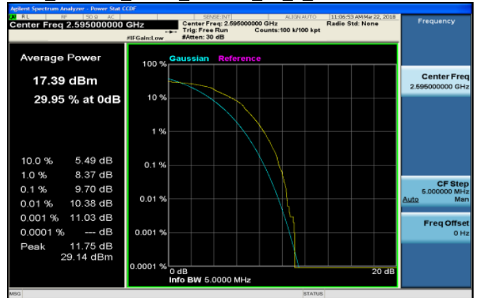
LTE_Band38_5MHz_64QAM_25_0_MidCH38000-2595
