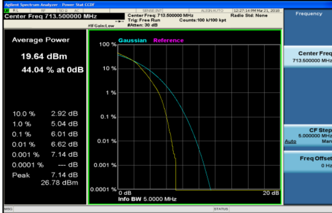
LTE_Band17_5MHz_64QAM_25_0_HighCH23825-713.5
