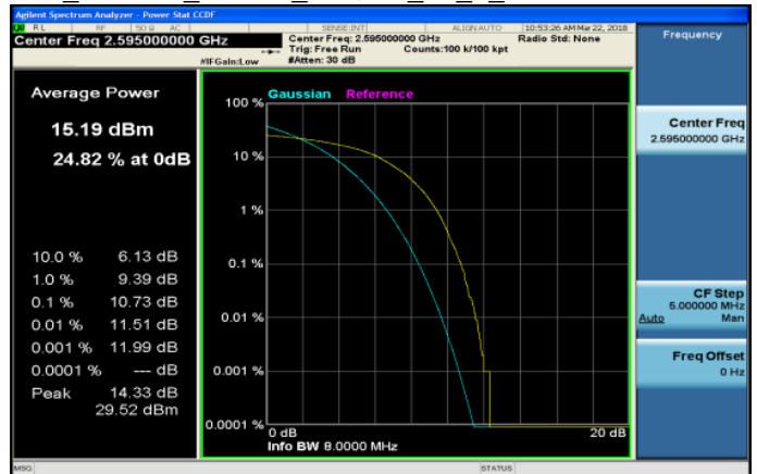
LTE_Band38_15MHz_64QAM_75_0_MidCH38000-2595
