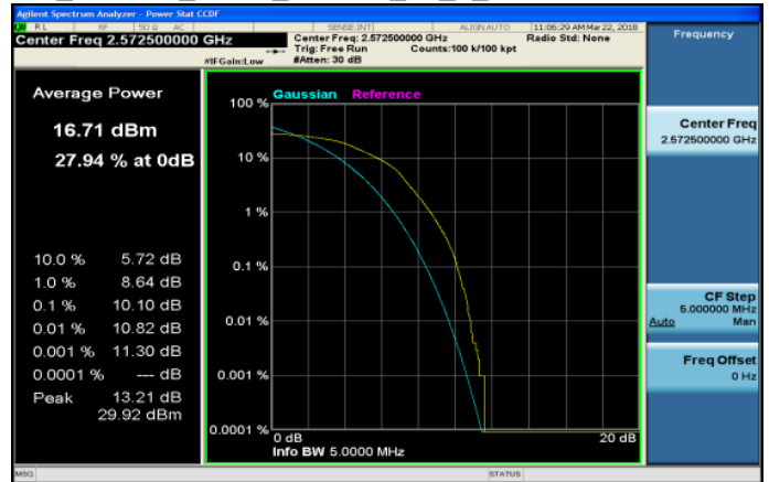
LTE_Band38_5MHz_64QAM_25_0_LowCH37775-2572.5
