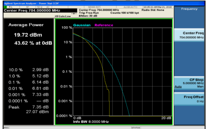
LTE_Band12_10MHz_64QAM_50_0_LowCH23060-704
