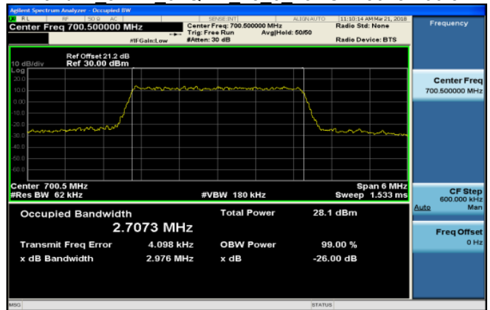
Band12_3MHz_64QAM_15_0_LowCH23025-700.5
