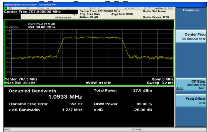
Band12_1_4MHz_16QAM_6_0_MidCH23095-707.5
