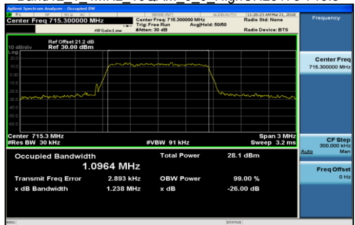
Band12_1_4MHz_16QAM_6_0_HighCH23173-715.3
