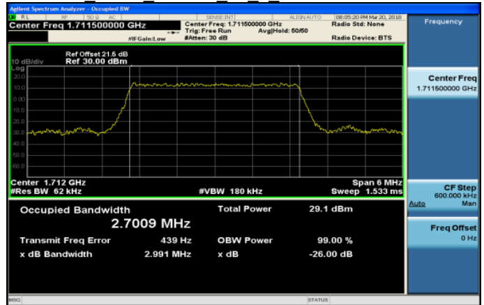
Band4_3MHz_64QAM_15_0_LowCH19965-1711.5
