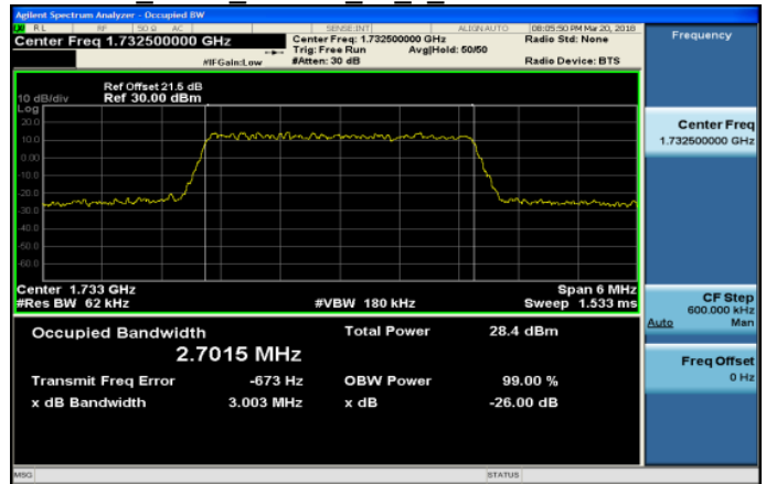
Band4_3MHz_64QAM_15_0_MidCH20175-1732.5
