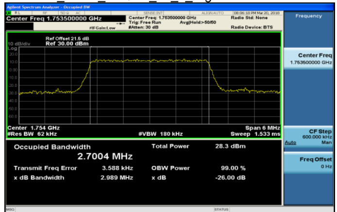
Band4_3MHz_64QAM_15_0_HighCH20385-1753.5
