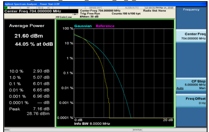
LTE_Band12_10MHz_64QAM_50_0_LowCH23060-704
