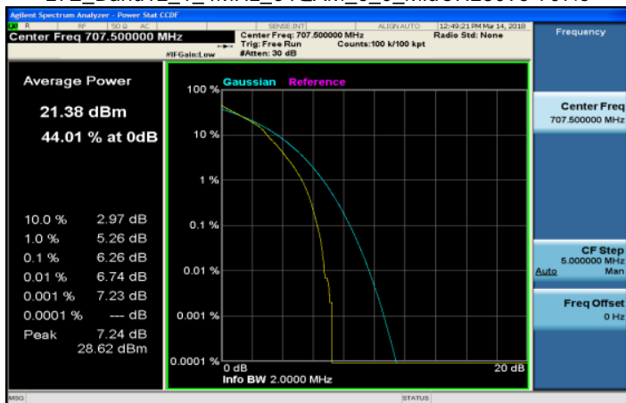
LTE_Band12_1_4MHz_64QAM_6_0_MidCH23095-707.5
