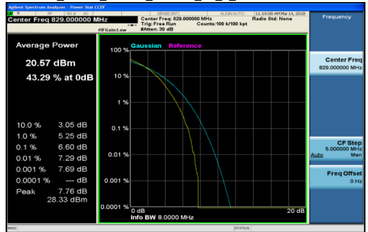
LTE_Band5_10MHz_64QAM_50_0_LowCH20450-829
