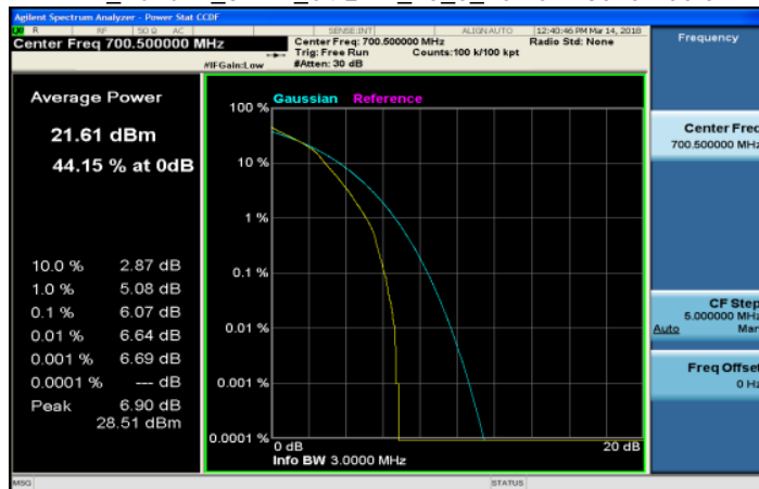
LTE_Band12_3MHz_64QAM_15_0_LowCH23025-700.5
