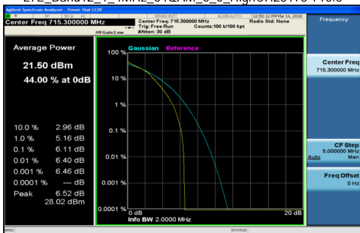
LTE_Band12_1_4MHz_64QAM_6_0_HighCH23173-715.3
