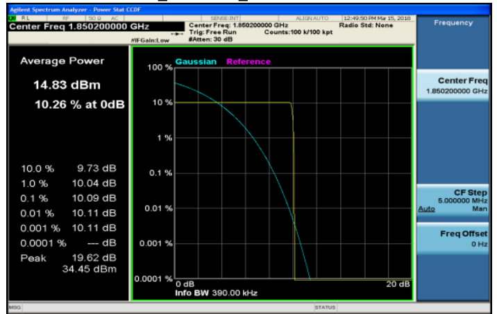
GPRS_1900MHz_LowCH512-1850.2
