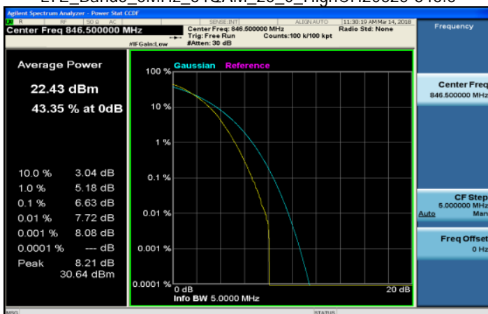
LTE_Band5_5MHz_64QAM_25_0_HighCH20625-846.5
