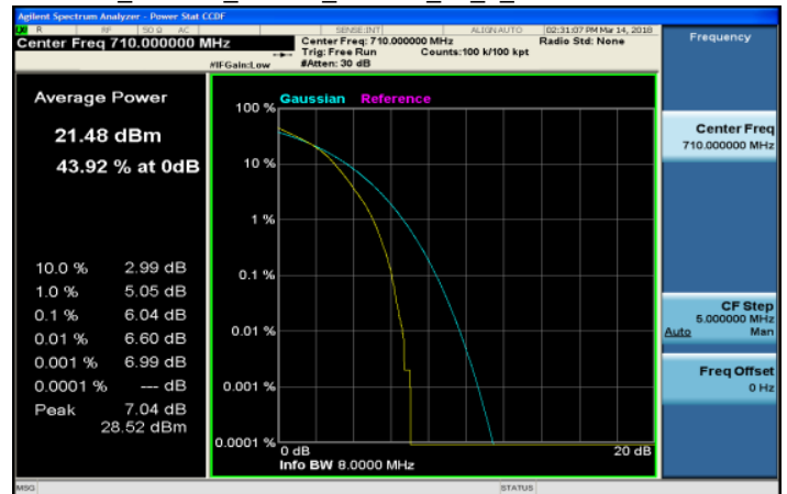
LTE_Band17_10MHz_64QAM_50_0_MidCH23790-710
