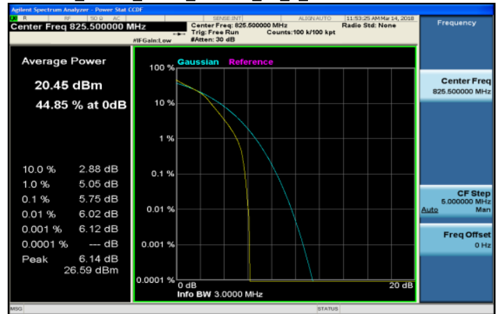
LTE_Band5_3MHz_64QAM_15_0_LowCH20415-825.5
