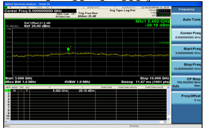
3GHz~10GHz_Band12_1_4MHz_QPSK_1_0_HighCH23173-715.3
