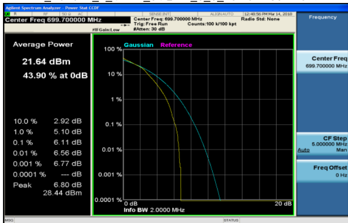
LTE_Band12_1_4MHz_64QAM_6_0_LowCH23017-699.7
