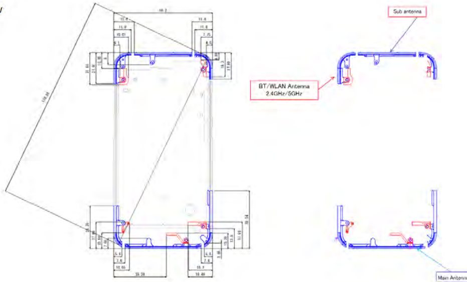
Fig.17 Antenna position of EUT
