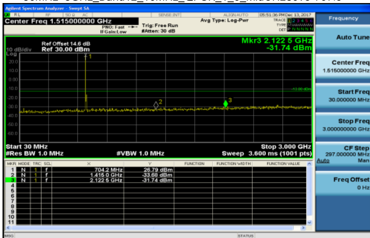
30MHz-3GHz_Band12_10MHz_QPSK_1_0_MidCH23095-707.5
