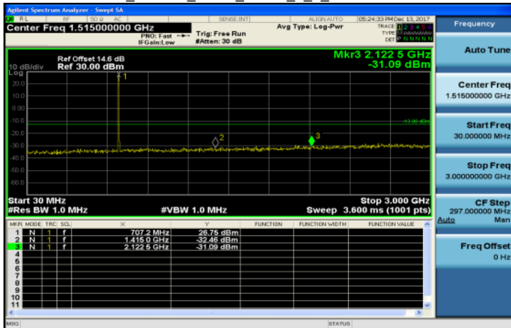
30MHz~3GHz_Band12_3MHz_QPSK_1_0_MidCH23095-707.5
