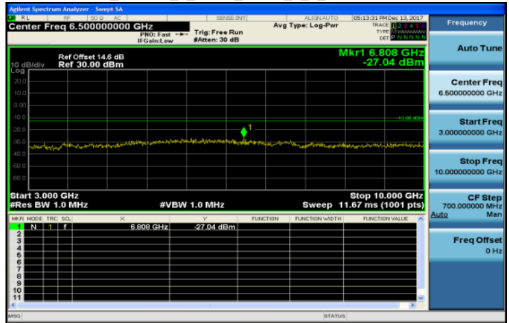
3GHz-10GHz_Band12_1_4MHz_QPSK_1_0_MidCH23095-707.5
