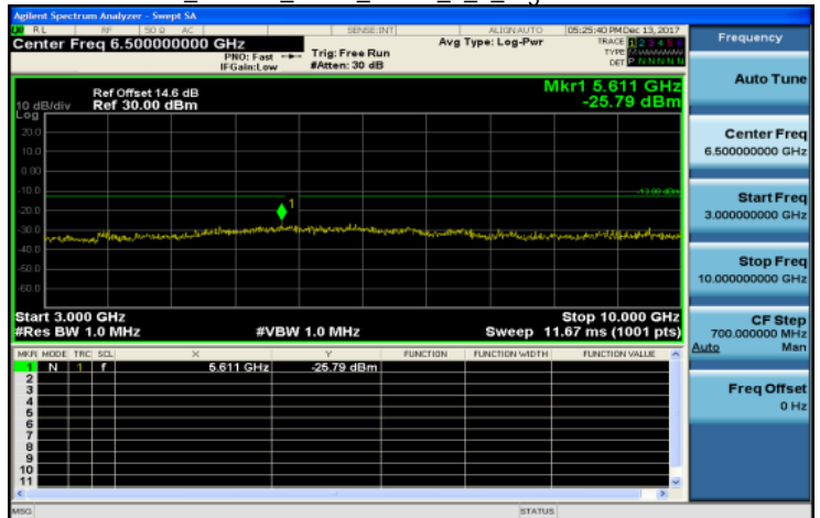
3GHz~10GHz_Band12_3MHz_QPSK_1_0_HighCH23165-714.5
