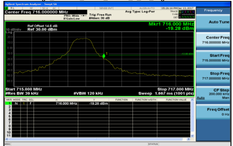
Band Edge_Band12_3MHz_QPSK_1_14_HighCH23165-714.5
