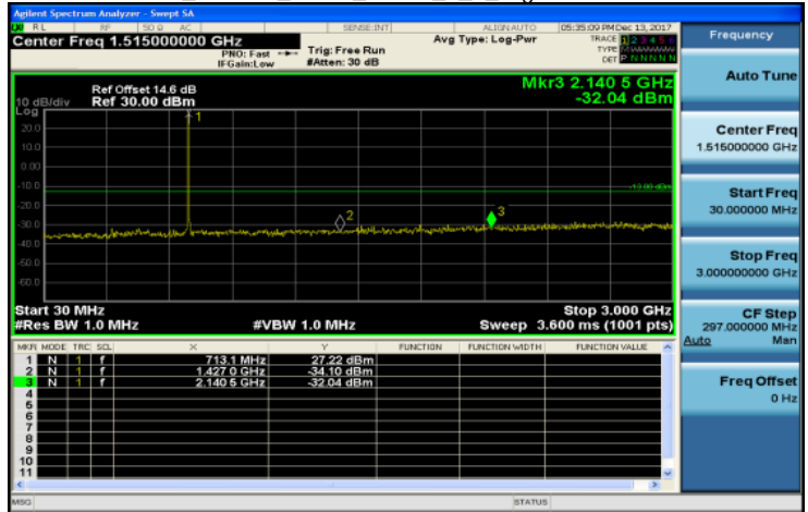
30MHz~3GHz_Band12_5MHz_QPSK_1_0_HighCH23155-713.5
