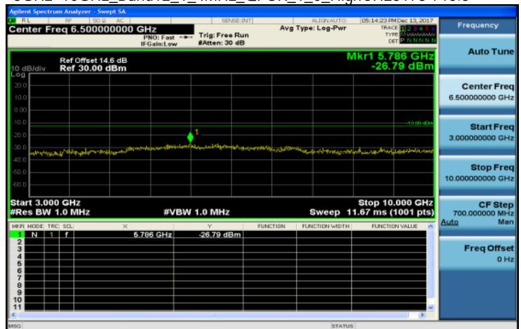
3GHz-10GHz_Band12_1_4MHz_QPSK_1_0_HighCH23173-715.3
