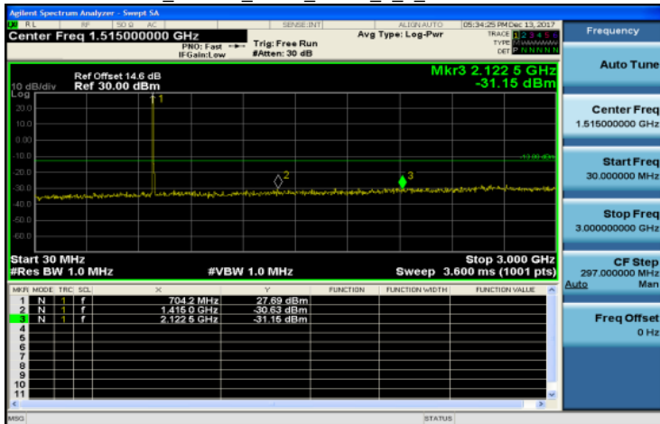
30MHz~3GHz_Band12_5MHz_QPSK_1_0_MidCH23095-707.5
