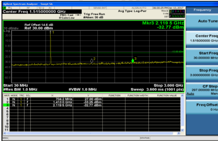
30MHz~3GHz_Band17_5MHz_QPSK_1_0_LowCH23755-706.5
