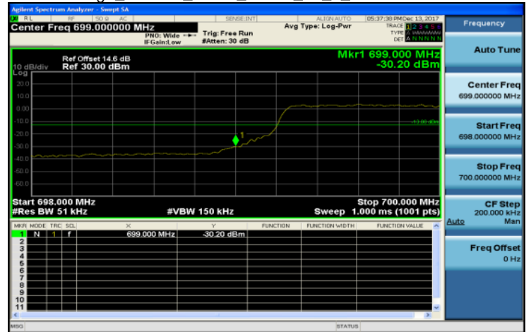
Band Edge_Band12_5MHz_QPSK_25_0_LowCH23035-701.5
