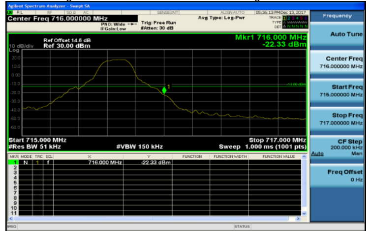
Band Edge_Band12_5MHz_QPSK_1_24_HighCH23155-713.5
