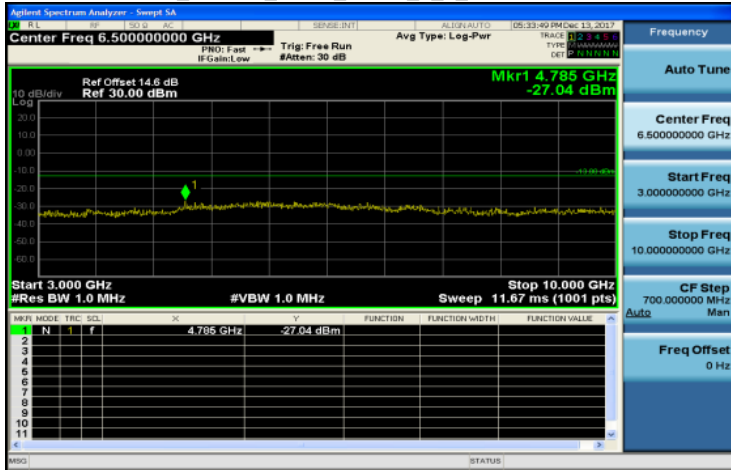
3GHz~10GHz_Band12_5MHz_QPSK_1_0_LowCH23035-701.5
