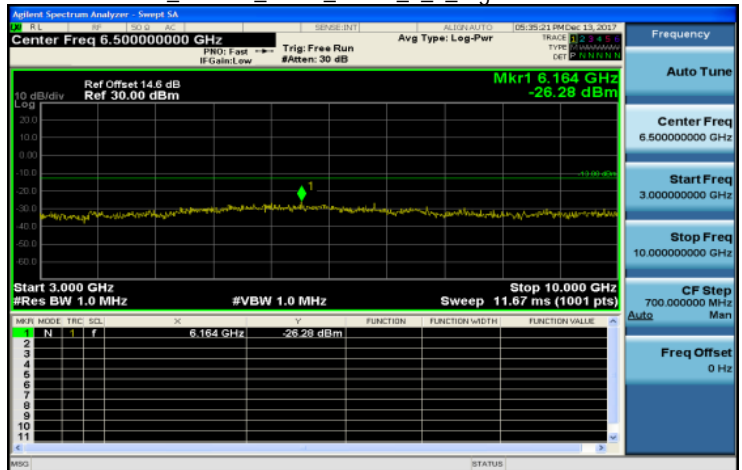
3GHz~10GHz_Band12_5MHz_QPSK_1_0_HighCH23155-713.5
