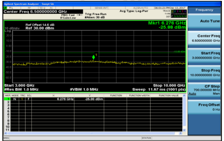
3GHz~10GHz_Band17_5MHz_QPSK_1_0_MidCH23790-710
