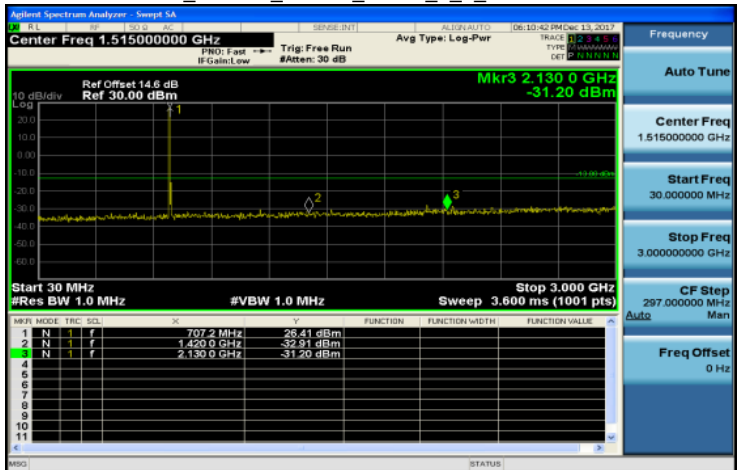
30MHz-3GHz_Band17_10MHz_QPSK_1_0_MidCH23790-710
