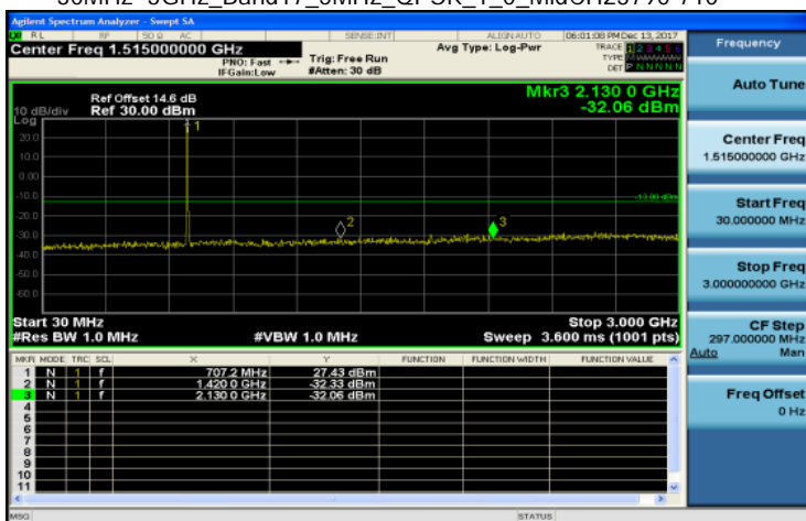
30MHz~3GHz_Band17_5MHz_QPSK_1_0_MidCH23790-710
