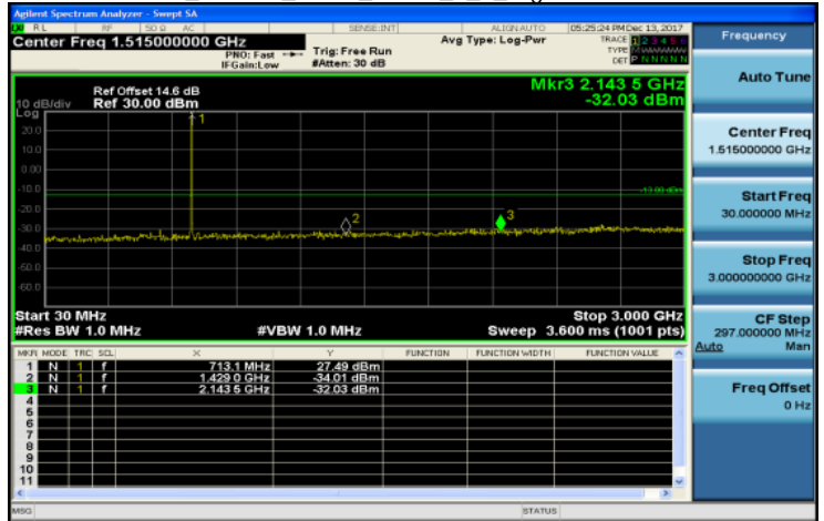
30MHz~3GHz_Band12_3MHz_QPSK_1_0_HighCH23165-714.5
