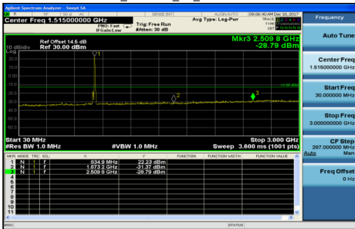
30MHz~3GHz_WCDMA_B5_MidCH4183-836.6
