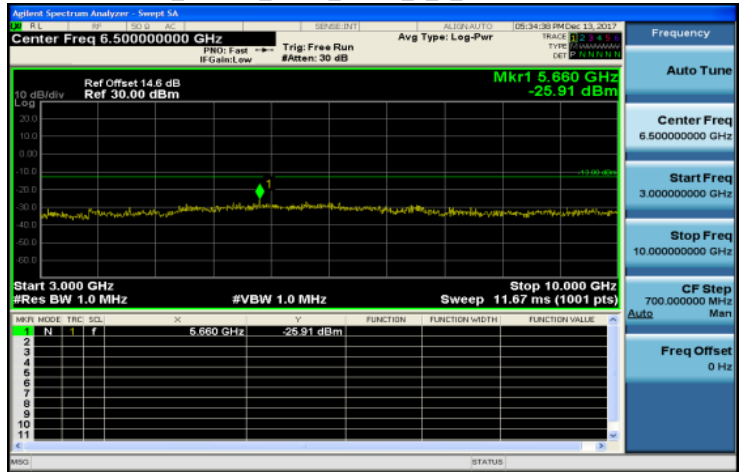
3GHz~10GHz_Band12_5MHz_QPSK_1_0_MidCH23095-707.5
