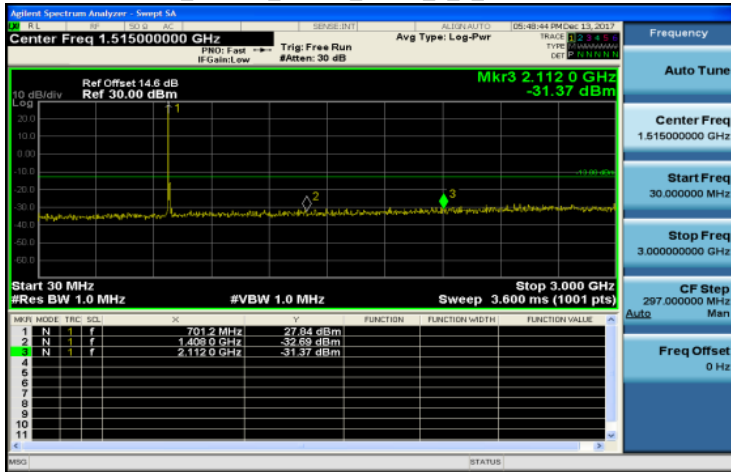
30MHz-3GHz_Band12_10MHz_QPSK_1_0_LowCH23060-704
