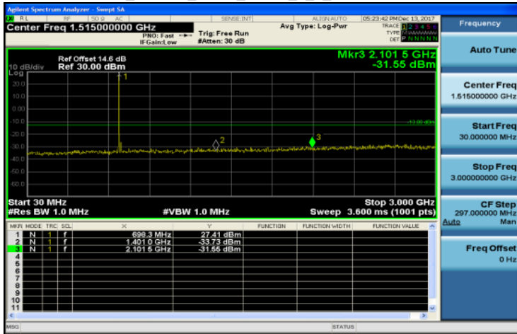
30MHz~3GHz_Band12_3MHz_QPSK_1_0_LowCH23025-700.5
