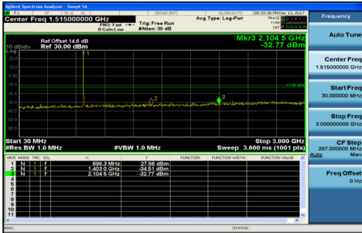
30MHz~3GHz_Band12_5MHz_QPSK_1_0_LowCH23035-701.5
