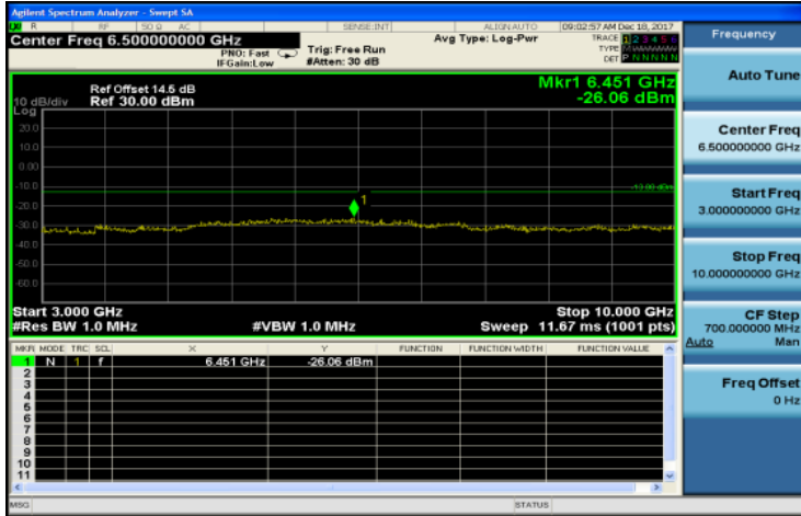
3GHz~10GHz_WCDMA_B5_LowCH4132-826.4
