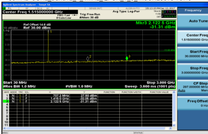
30MHz-3GHz_Band12_1_4MHz_QPSK_1_0_MidCH23095-707.5
