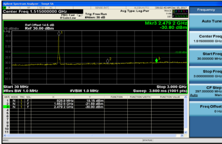
30MHz~3GHz_WCDMA_B5_LowCH4132-826.4
