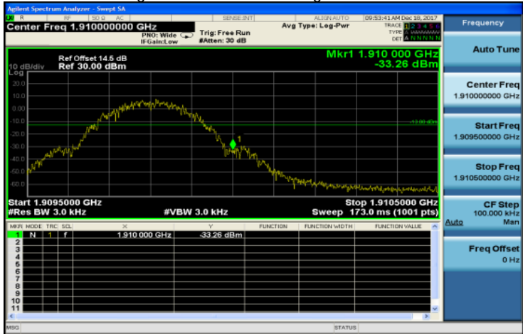
Band Edge_GSM_1900MHz_HighCH810-1909.8
