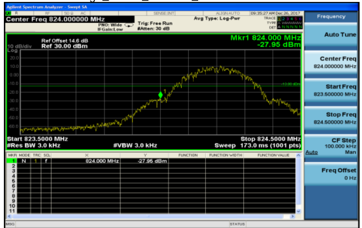
Band Edge_GPRS_850MHz_LowCH128-824.2
