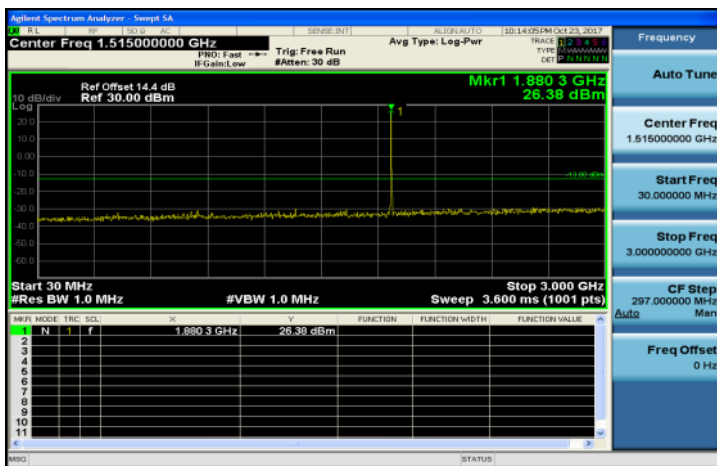
30MHz~3GHz_Band2_3MHz_QPSK_1_0_MidCH18900-1880
