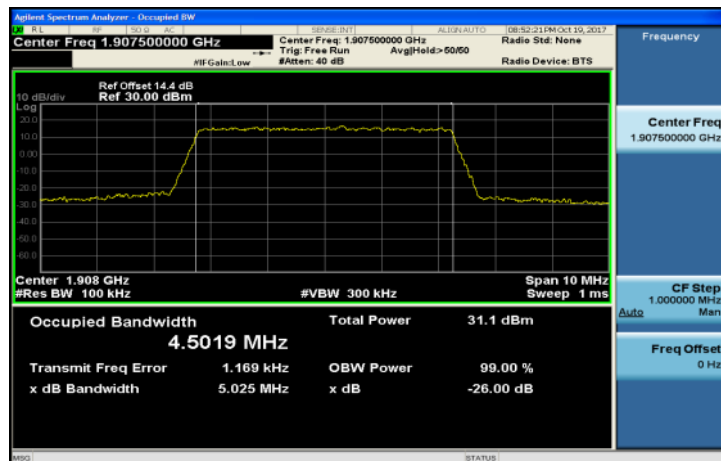
Band2_5MHz_QPSK_25_0_HighCH19175-1907.5
