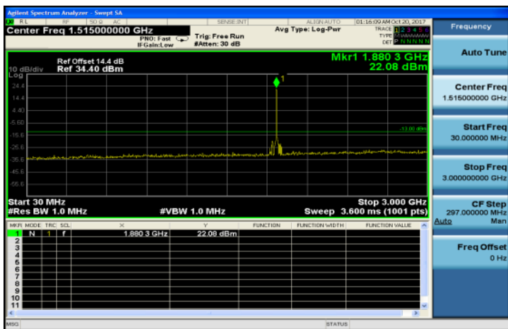
30MHz~3GHz_HSUPA_B2_MidCH9400-1880
