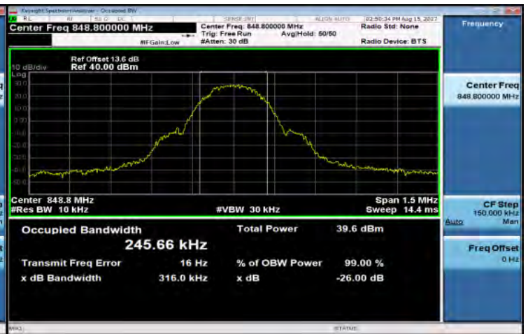
GPRS_850MHz_HighCH251-848.8
