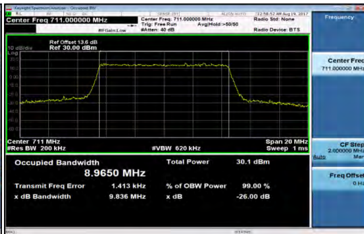
Band12_10MHz_16QAM_50_0_HighCH23130-711
