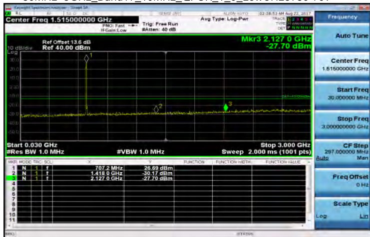
30MHz-3GHz_Band17_10MHz_QPSK_1_0_LowCH23780-709
