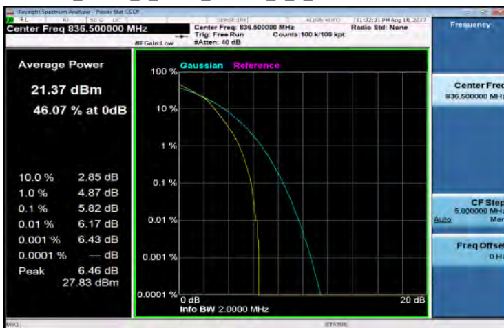
LTE_Band5_1_4MHz_16QAM_6_0_Channel Mid
