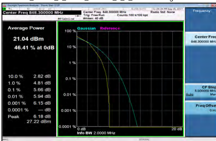
LTE_Band5_1_4MHz_16QAM_6_0_Channel High
