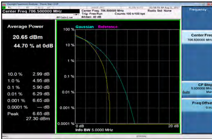
LTE_Band17_5MHz_16QAM_25_0_Channel Low
