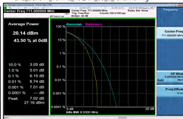
LTE_Band17_10MHz_16QAM_50_0_Channel High
