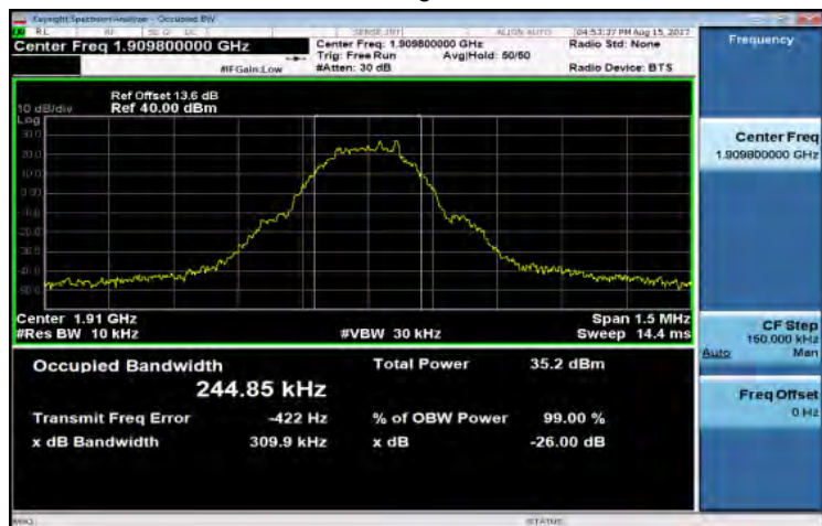
GRPS_1900MHz_HighCH810-1909.8
