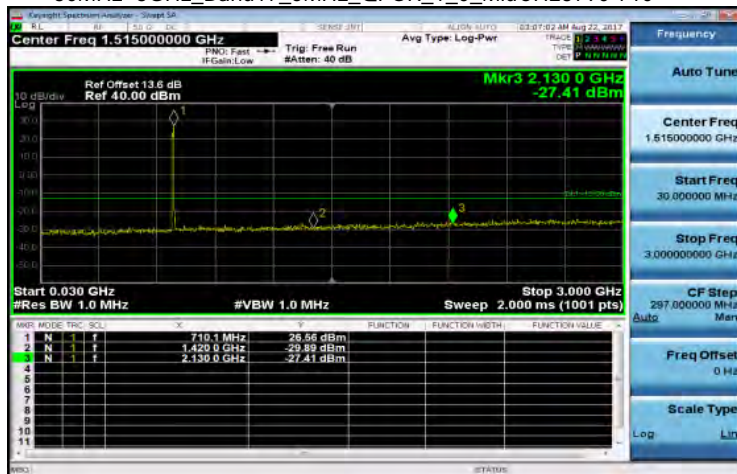
30MHz~3GHz_Band17_5MHz_QPSK_1_0_MidCH23790-710
