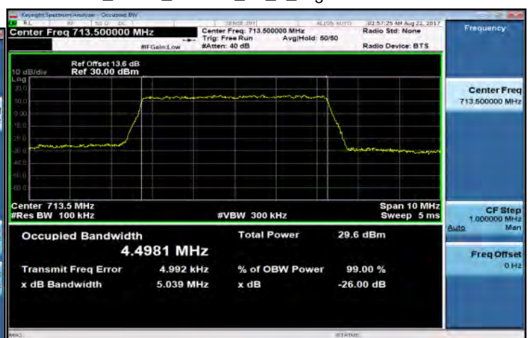
Band17_5MHz_16QAM_25_0_HighCH23825-713.5
