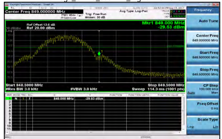
Band Edge_GPRS_850MHz_HighCH251-848.8
