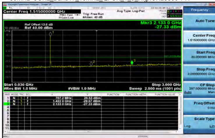
30MHz-3GHz_Band17_10MHz_QPSK_1_0_HighCH23800-711
