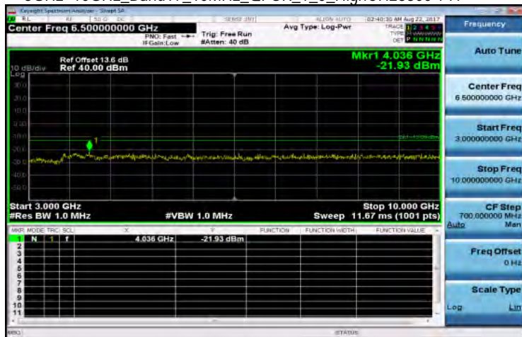
3GHz-10GHz_Band17_10MHz_QPSK_1_0_HighCH23800-711
