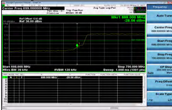
Band Edge_Band12_3MHz_QPSK_15_0_LowCH23025-700.5
