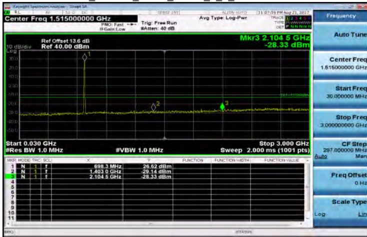
30MHz~3GHz_Band12_5MHz_QPSK_1_0_LowCH23035-701.5
