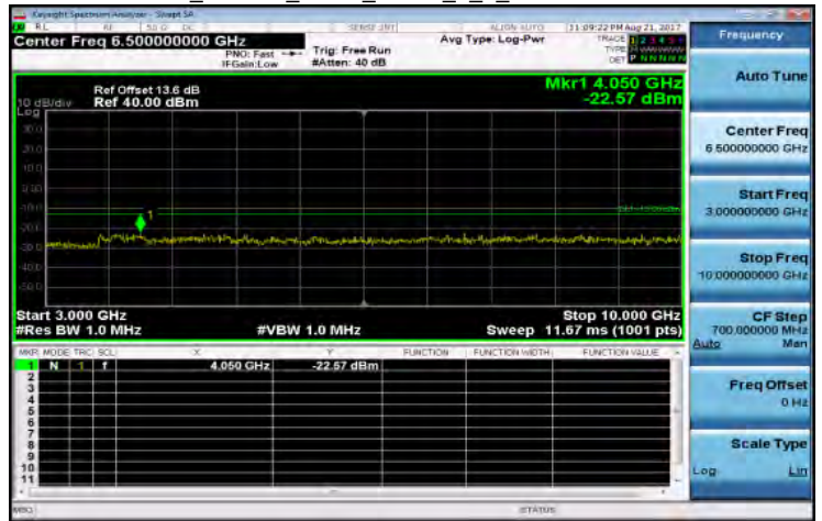
3GHz~10GHz_Band12_5MHz_QPSK_1_0_MidCH23095-707.5
