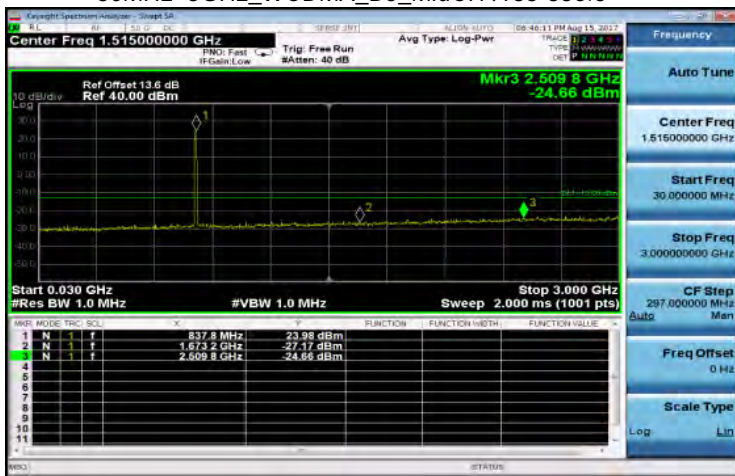
30MHz~3GHz_WCDMA_B5_MidCH4183-836.6
