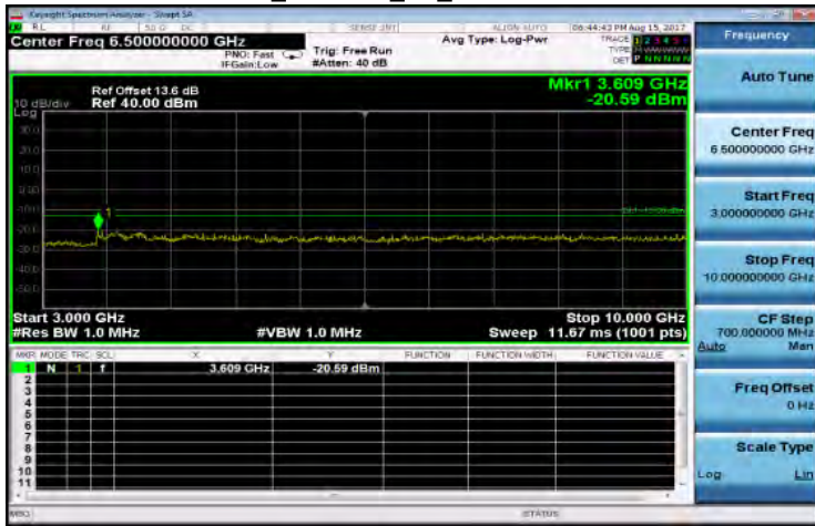
3GHz~10GHz_WCDMA_B5_LowCH4132-826.4
