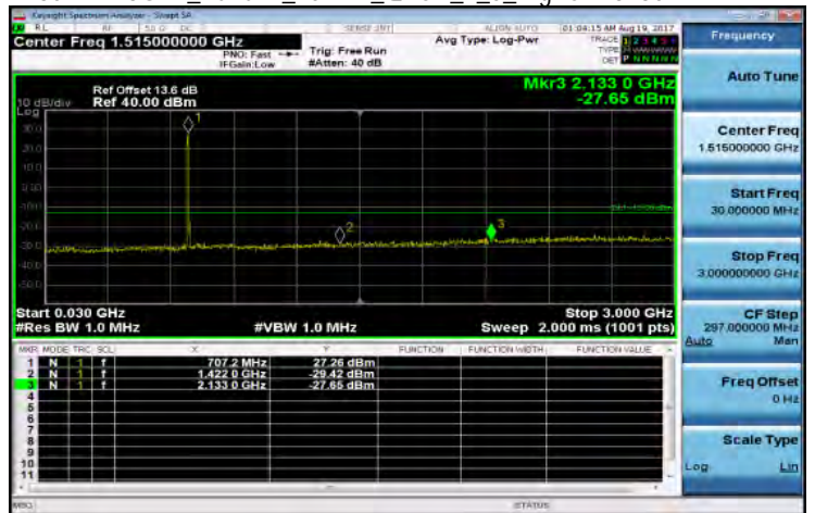
30MHz-3GHz_Band12_10MHz_QPSK_1_0_HighCH23130-711
