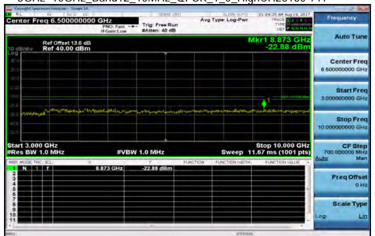
3GHz-10GHz_Band12_10MHz_QPSK_1_0_HighCH23130-711
