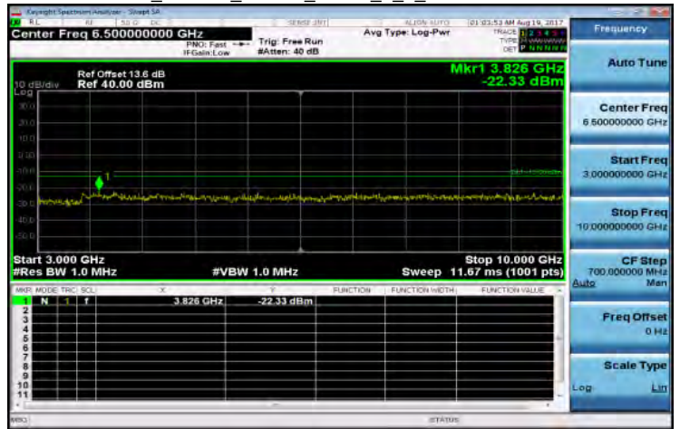
3GHz-10GHz_Band12_10MHz_QPSK_1_0_MidCH23095-707.5
