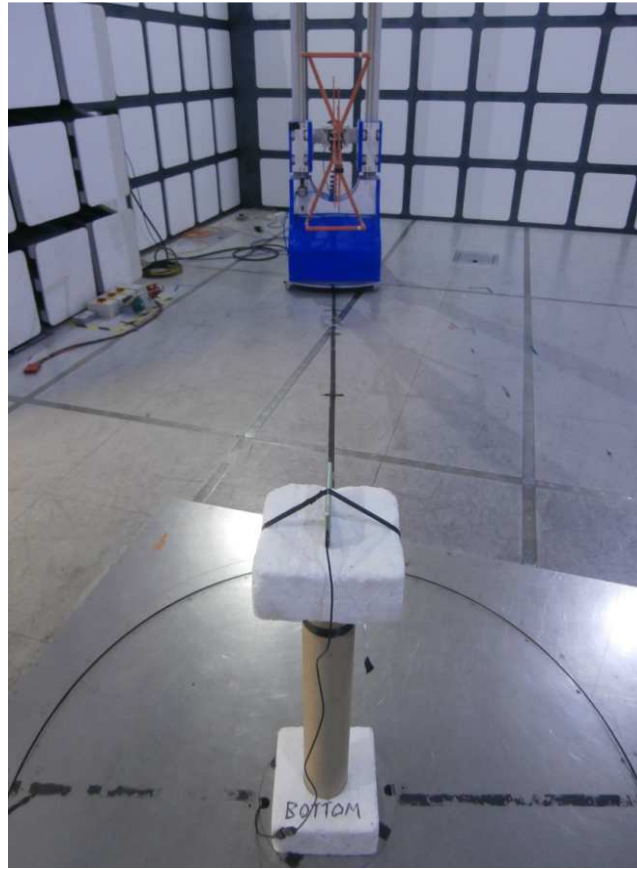
Radiated Emissions 30 MHz to 1 GHz
