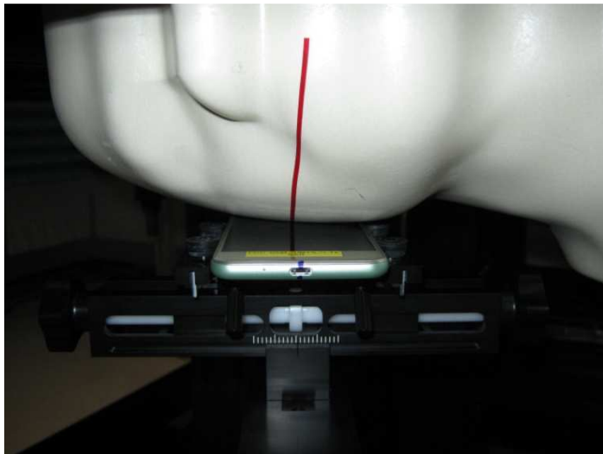
SAR - RH - Cheek
