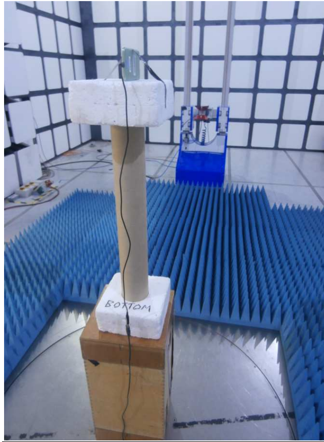
Radiated Emissions 1 GHz to 18 GHz
