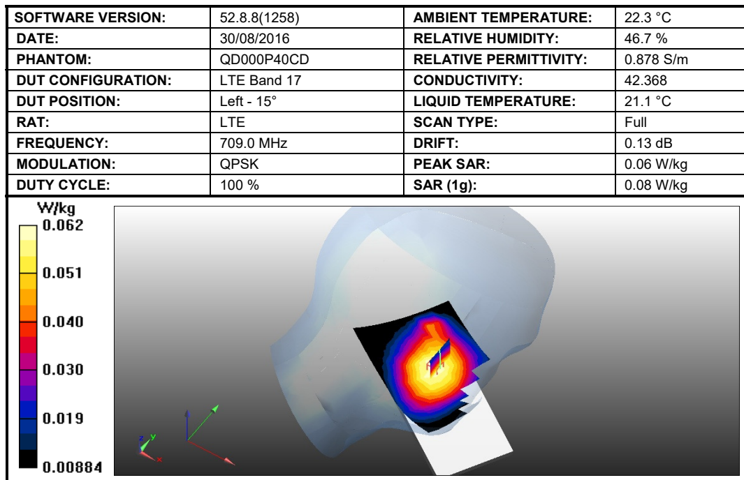
Figure 33: SAR Head Testing Results for the Sharp Smart phone at 709.0 MHz.
