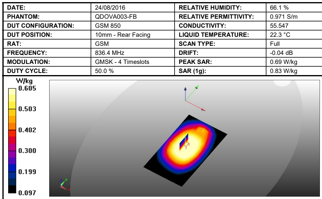
Figure 14: SAR Head Testing Results for the Sharp Smart phone at 836.4 MHz.
