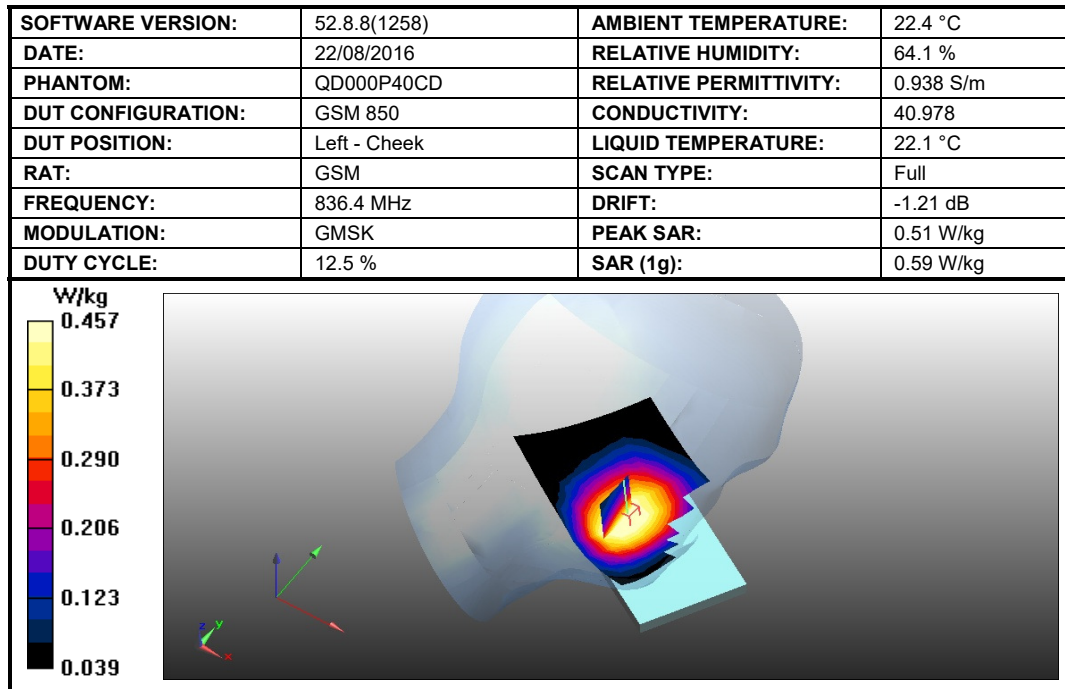
Figure 5: SAR Head Testing Results for the Sharp Smart phone at 836.4 MHz.
