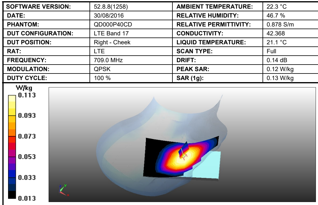
Figure 34: SAR Head Testing Results for the Sharp Smart phone at 709.0 MHz.
