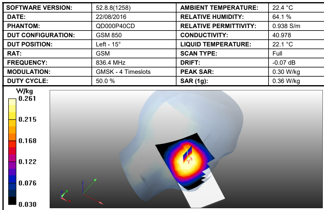
Figure 10: SAR Head Testing Results for the Sharp Smart phone at 836.4 MHz.
