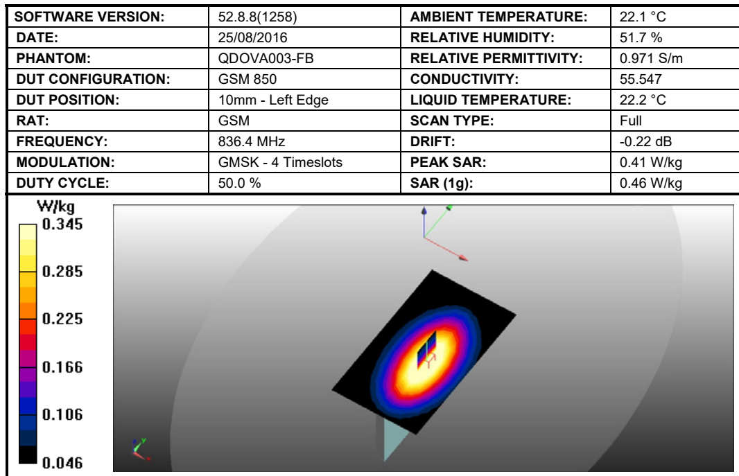
Figure 16: SAR Head Testing Results for the Sharp Smart phone at 836.4 MHz.
