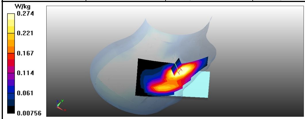
Figure 22: SAR Head Testing Results for the Sharp Smart phone at 1850.2 MHz.
