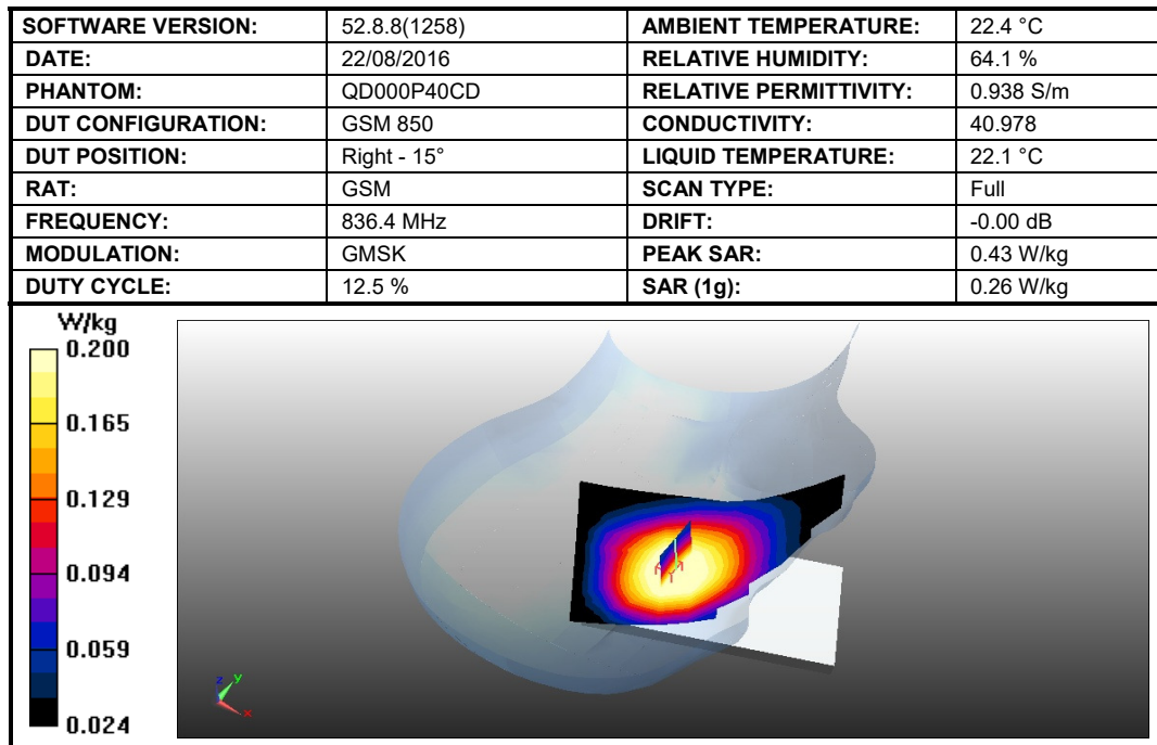
Figure 8: SAR Head Testing Results for the Sharp Smart phone at 836.4 MHz.
