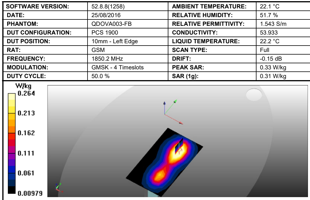
Figure 30: SAR Head Testing Results for the Sharp Smart phone at 1850.2 MHz.
