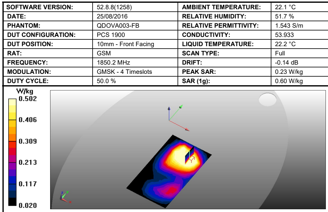
Figure 28: SAR Head Testing Results for the Sharp Smart phone at 1850.2 MHz.
