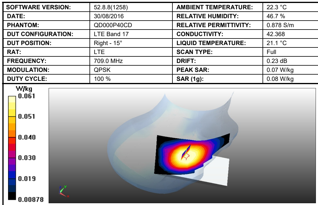
Figure 35: SAR Head Testing Results for the Sharp Smart phone at 709.0 MHz.
