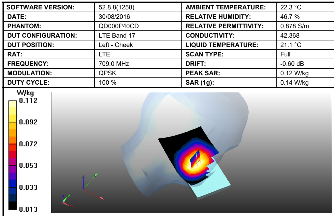
Figure 32: SAR Head Testing Results for the Sharp Smart phone at 709.0 MHz.
