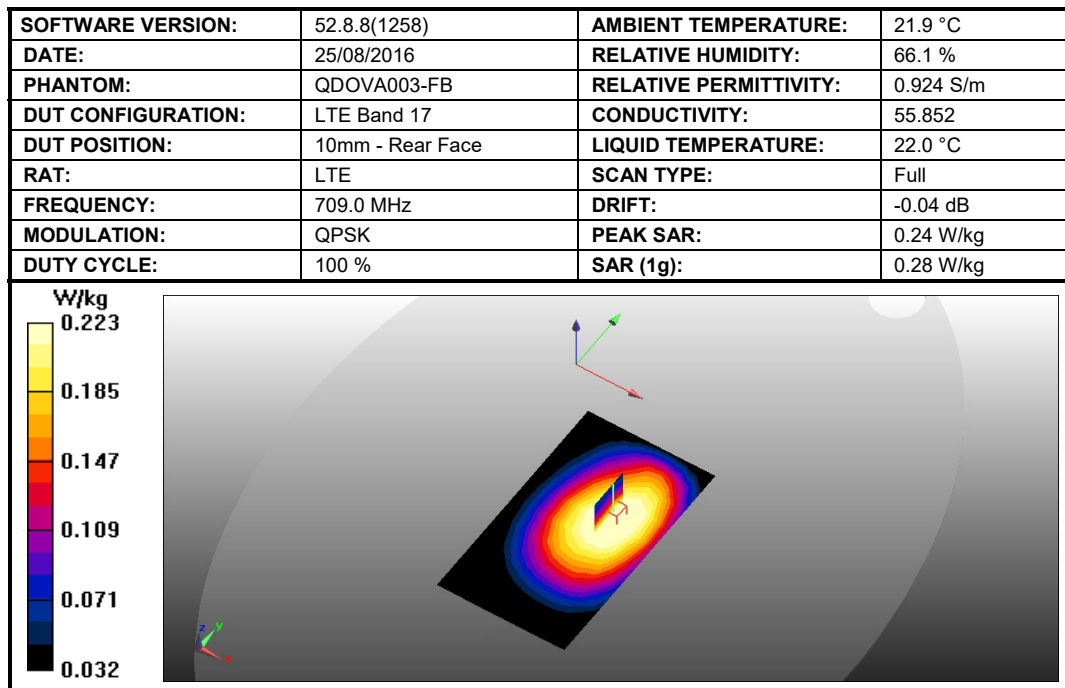
Figure 37: SAR Head Testing Results for the Sharp Smart phone at 709.0 MHz.
