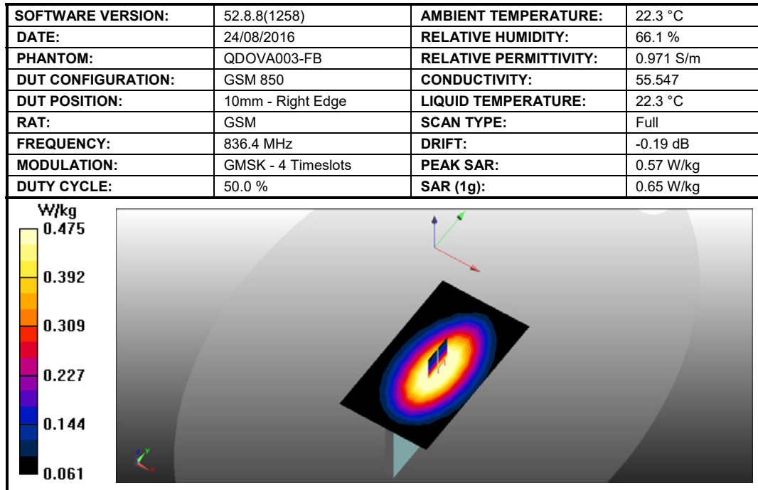
Figure 15: SAR Head Testing Results for the Sharp Smart phone at 836.4 MHz
