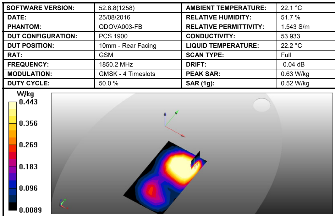
Figure 29: SAR Head Testing Results for the Sharp Smart phone at 1850.2 MHz.
