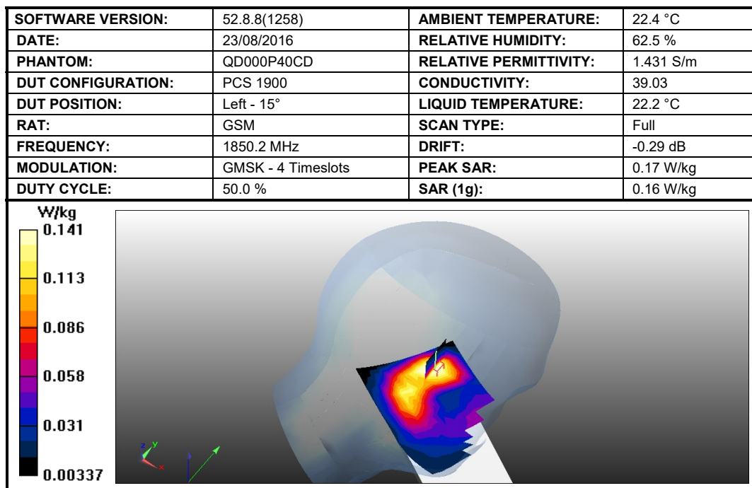
Figure 25: SAR Head Testing Results for the Sharp Smart phone at 1850.2 MHz.
