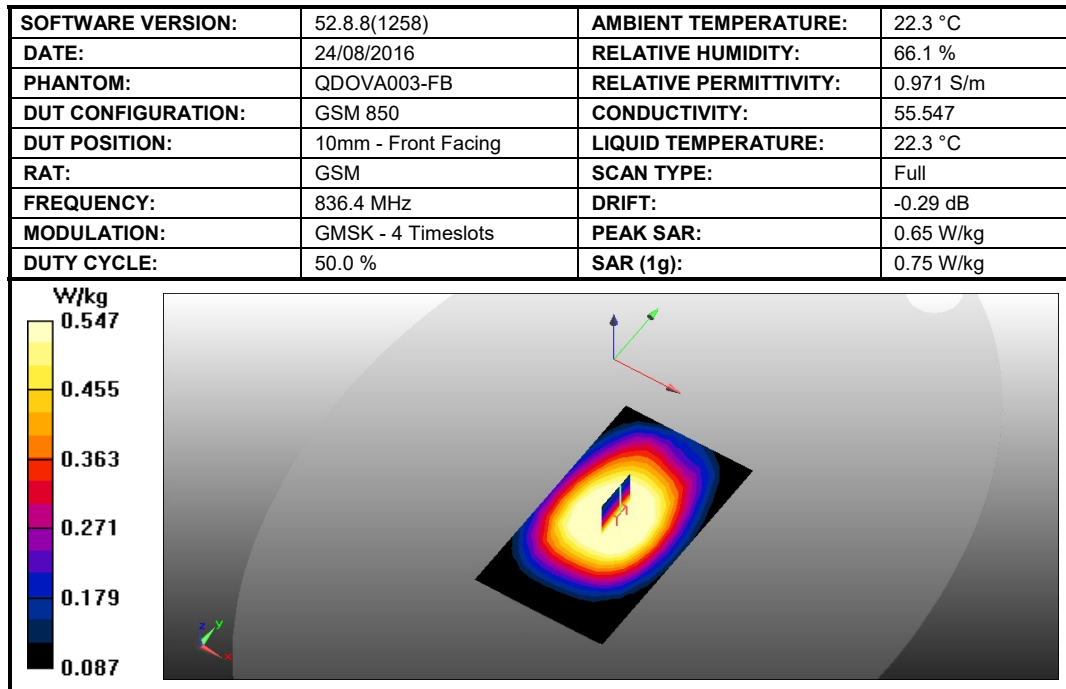
Figure 13: SAR Head Testing Results for the Sharp Smart phone at 836.4 MHz.
