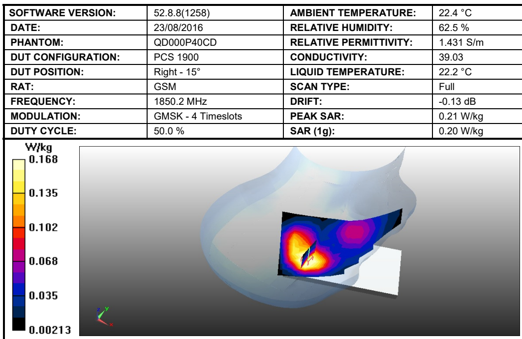
Figure 27 SAR Head Testing Results for the Sharp Smart phone at 1850.2 MHz.
