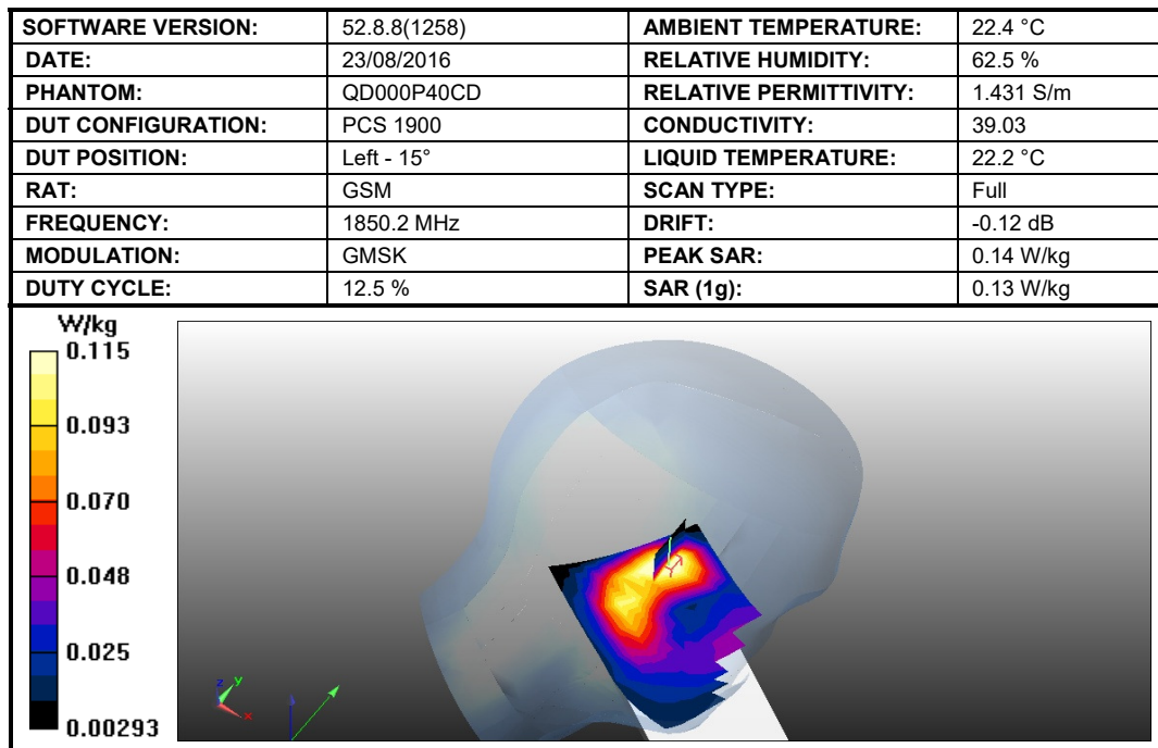
Figure 21: SAR Head Testing Results for the Sharp Smart phone at 1850.2 MHz.
