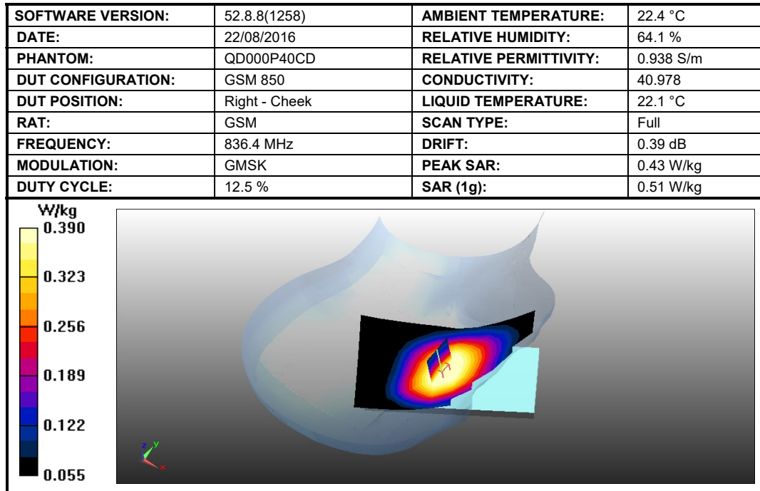
Figure 7: SAR Head Testing Results for the Sharp Smart phone at 836.4 MHz.
