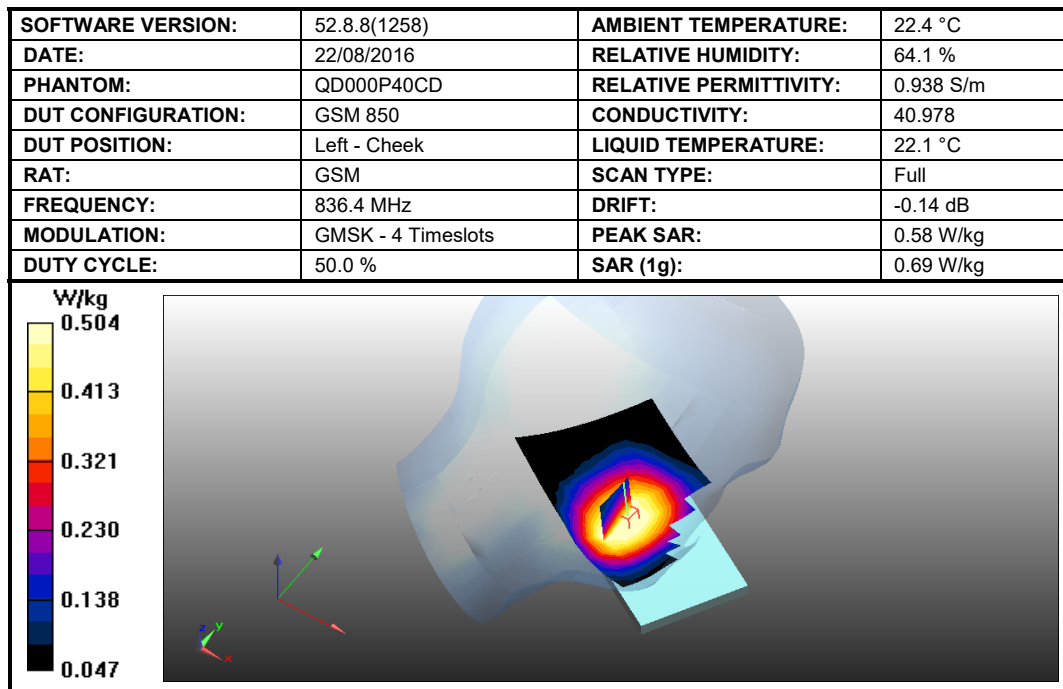
Figure 9: SAR Head Testing Results for the Sharp Smart phone at 836.4 MHz.
