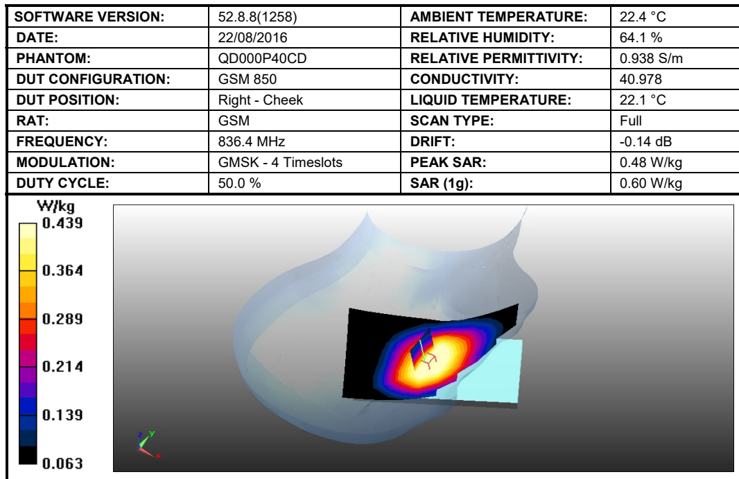
Figure 11: SAR Head Testing Results for the Sharp Smart phone at 836.4 MHz.
