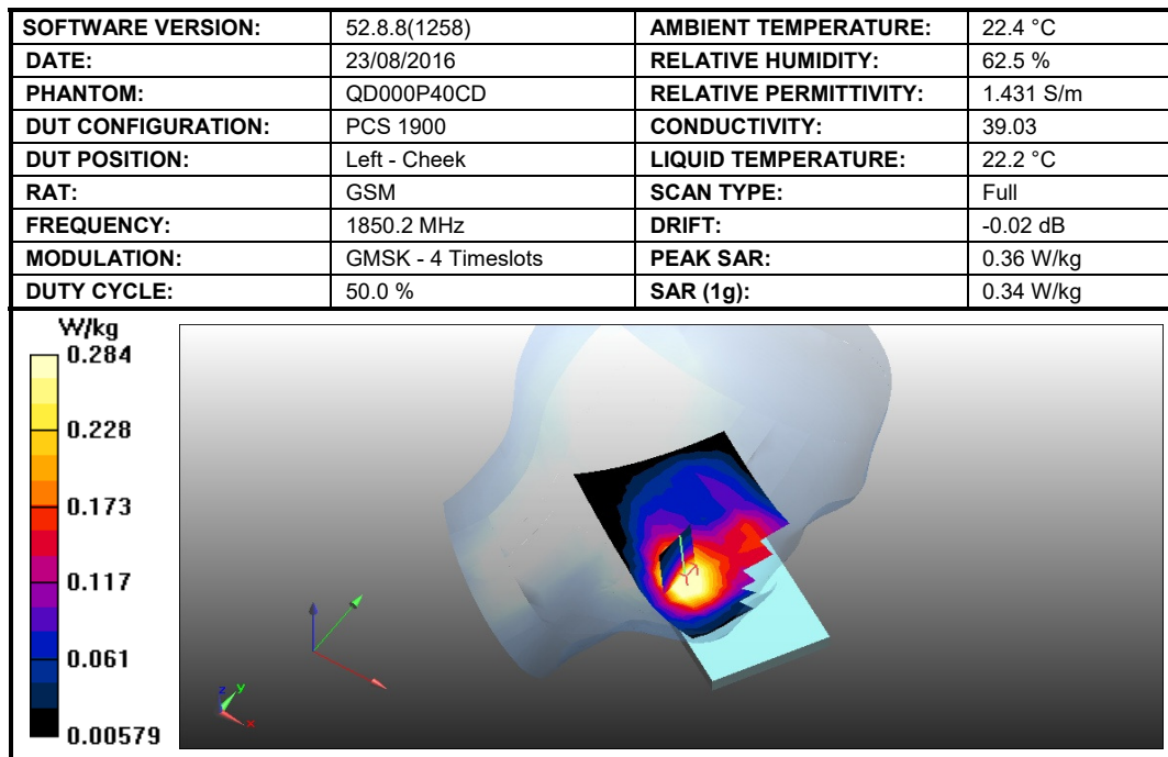
Figure 24: SAR Head Testing Results for the Sharp Smart phone at 1850.2 MHz.
