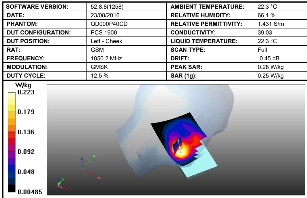
Figure 20: SAR Head Testing Results for the Sharp Smart phone at 1850.2 MHz.
