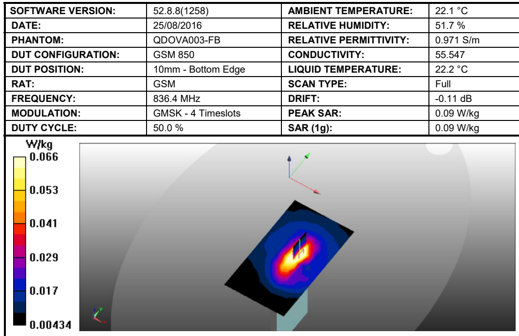
Figure 17: SAR Head Testing Results for the Sharp Smart phone at 836.4 MHz.
