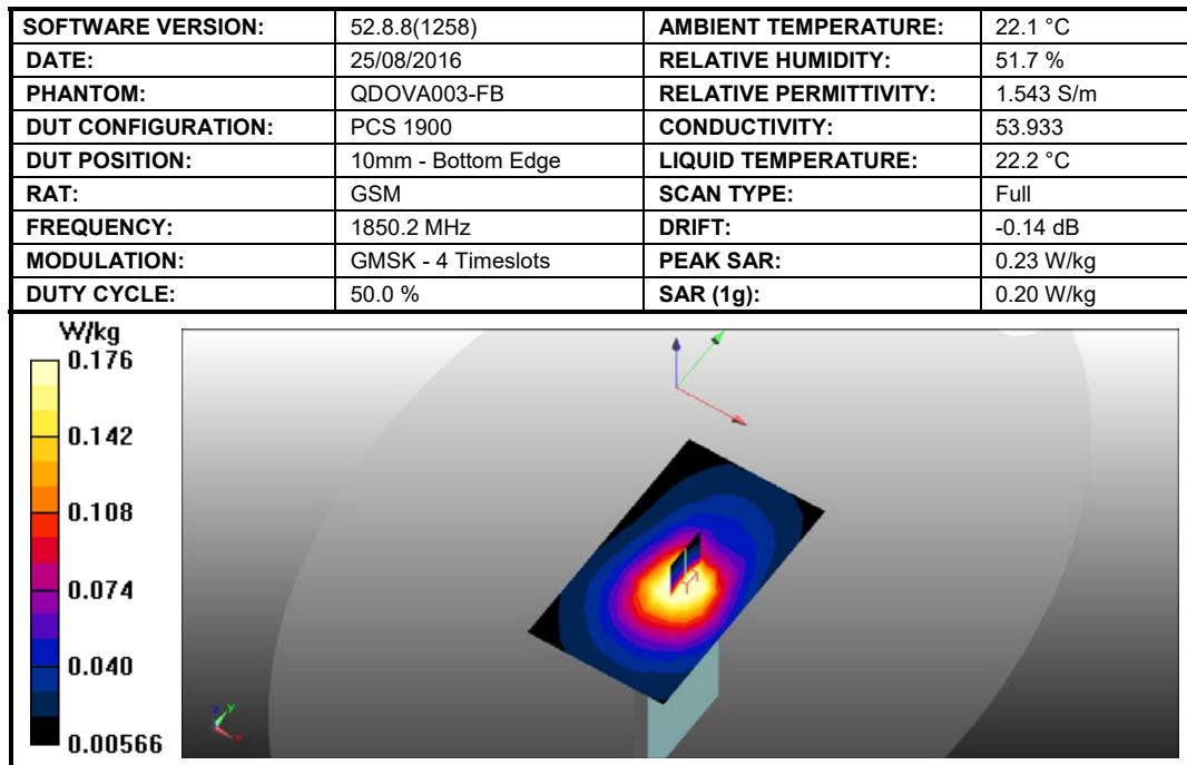
Figure 31: SAR Head Testing Results for the Sharp Smart phone at 1850.2 MHz.
