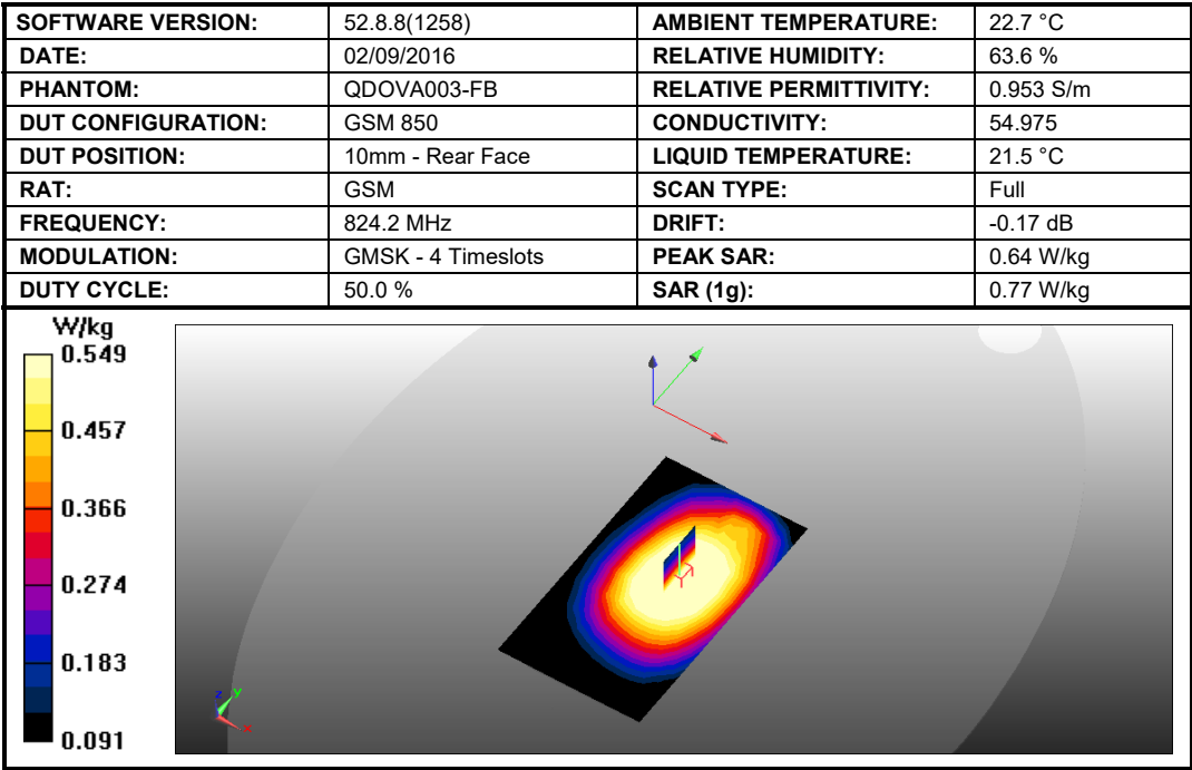
Figure 19: SAR Head Testing Results for the Sharp Smart phone at 824.2 MHz.
