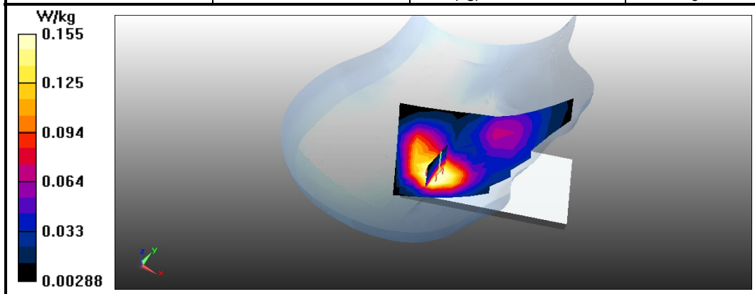
Figure 23: SAR Head Testing Results for the Sharp Smart phone at 1850.2 MHz.
