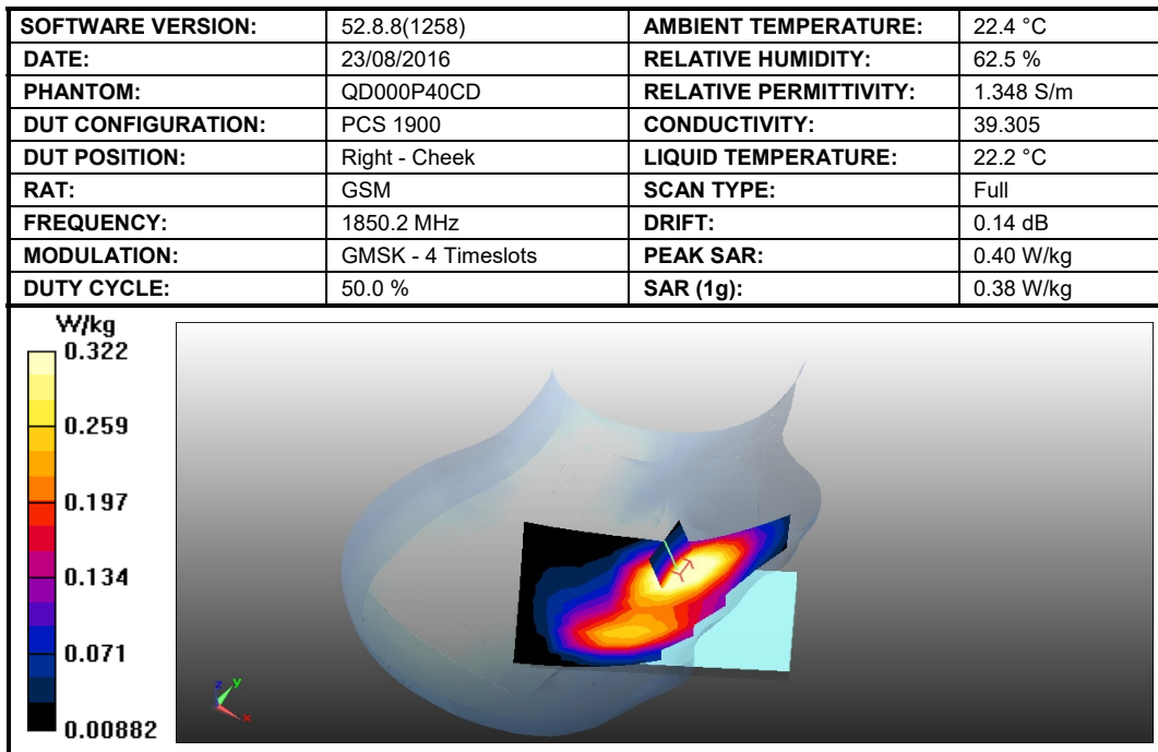
Figure 26: SAR Head Testing Results for the Sharp Smart phone at 1850.2 MHz.
