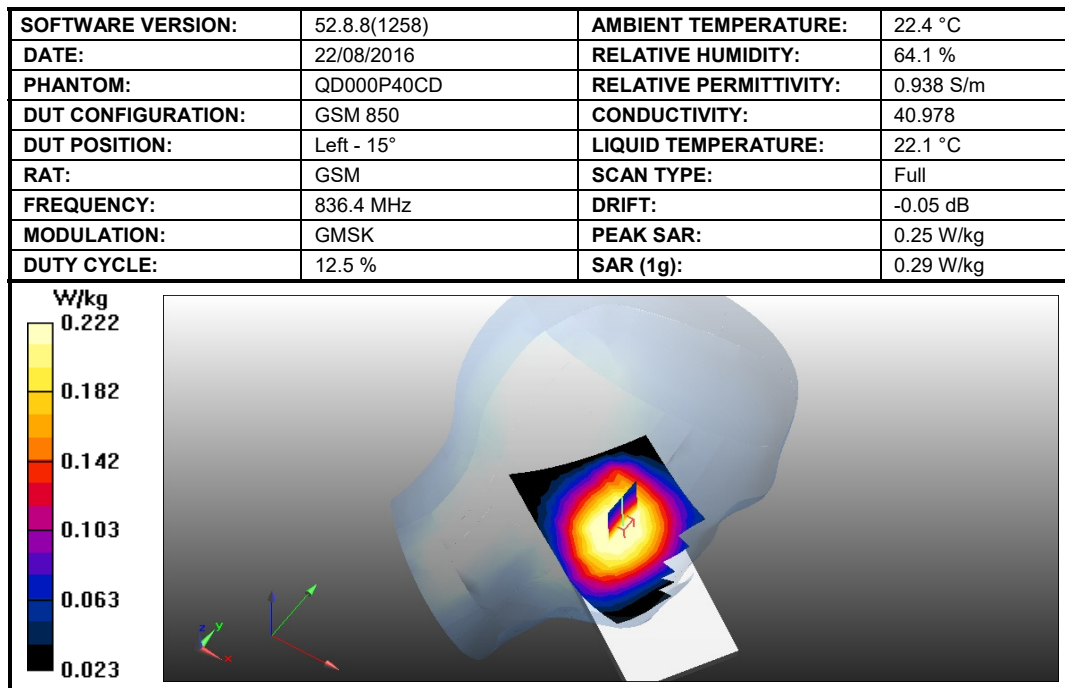
Figure 6: SAR Head Testing Results for the Sharp Smart phone at 836.4 MHz.
