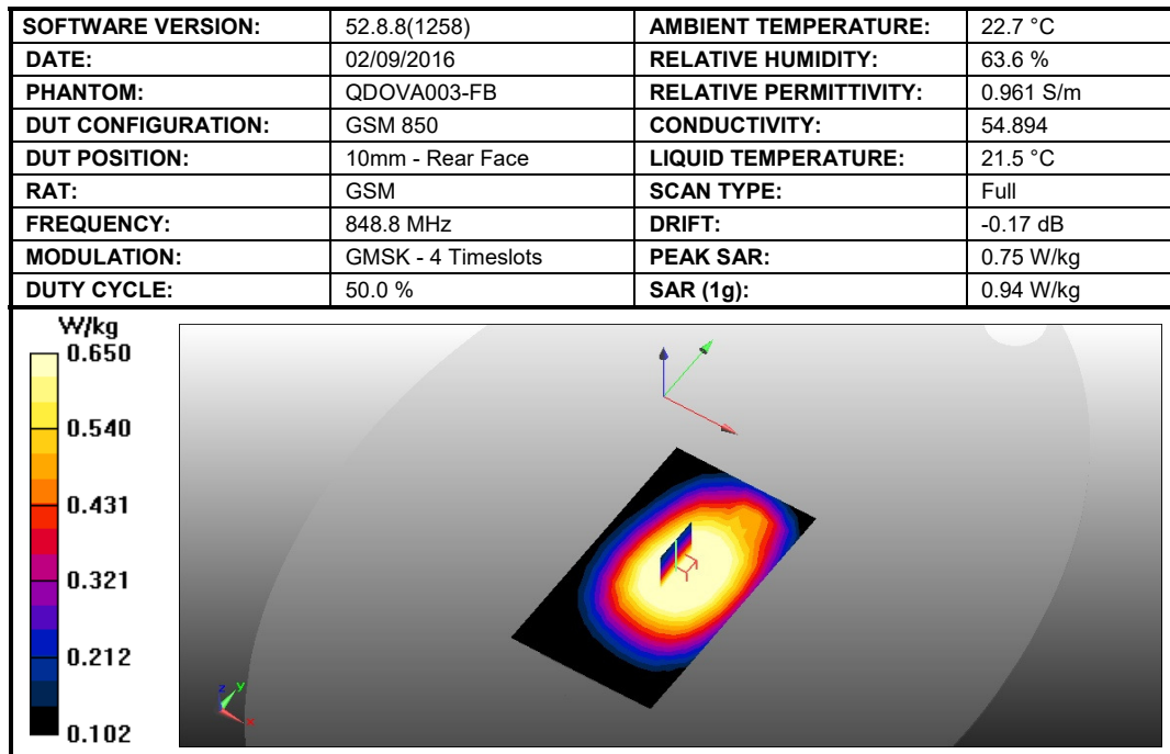
Figure 18 SAR Head Testing Results for the Sharp Smart phone at 848.8 MHz.
