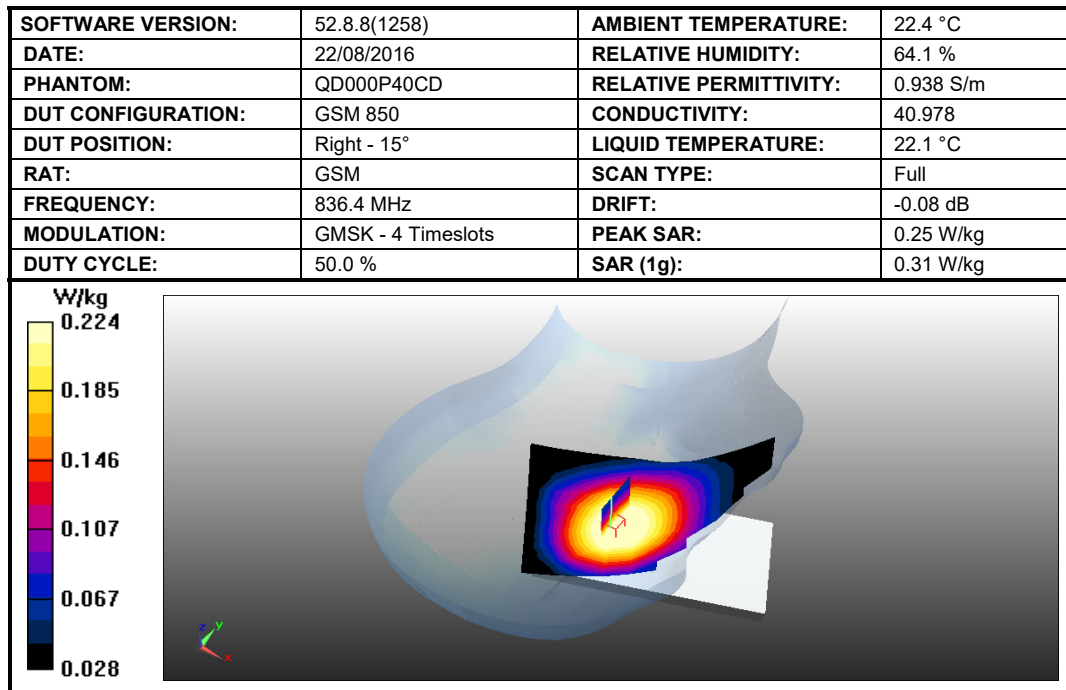
Figure 12: SAR Head Testing Results for the Sharp Smart phone at 836.4 MHz.
