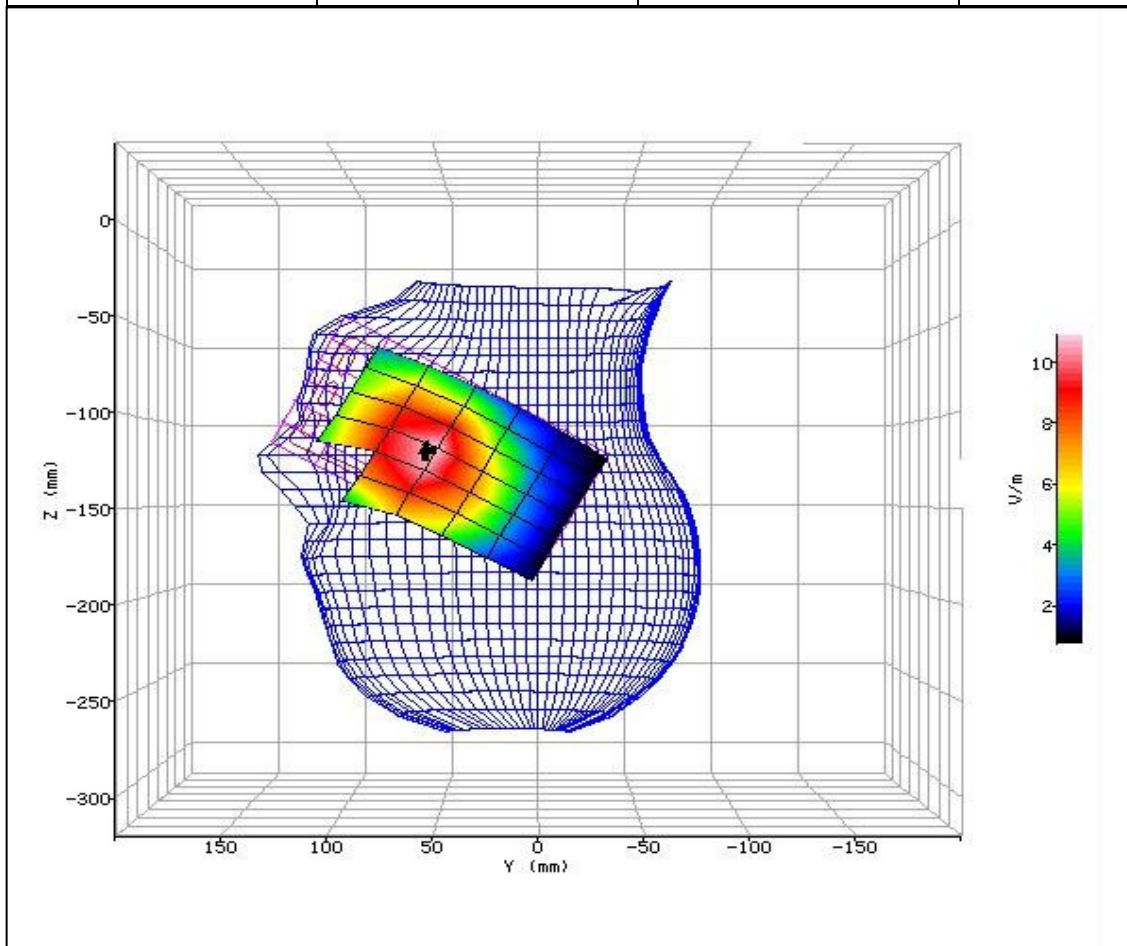
Figure 28: SAR Head Testing Results for the Mobile Handset at 710.0MHz.
