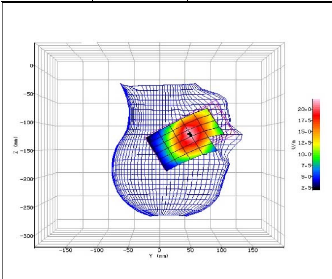
Figure 12: SAR Head Testing Results for the Sharp Smart phone at 836.4MHz.
