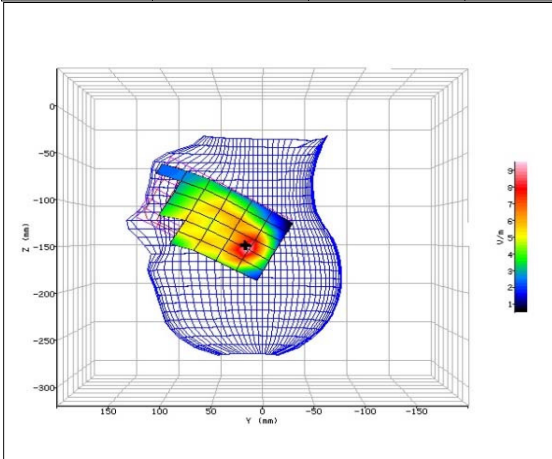
Figure 47: SAR Head Testing Results for the Sharp Smart phone at 1909.8MHz.
