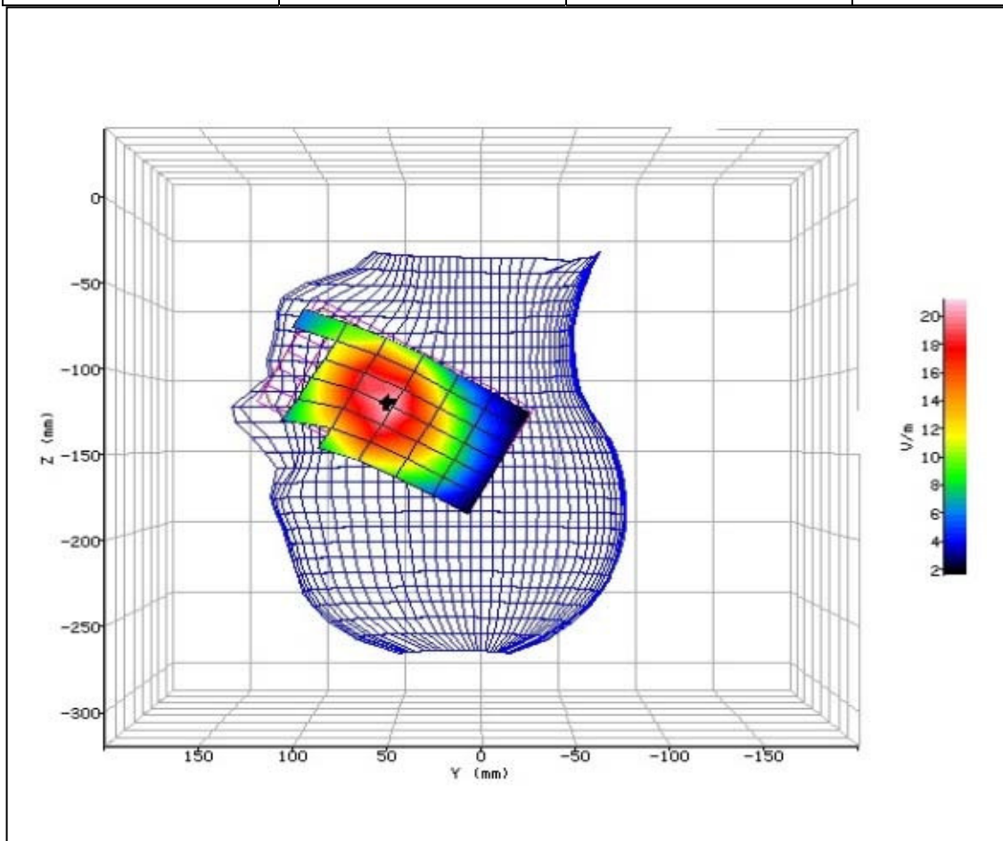
Figure 6: SAR Head Testing Results for the Sharp Smart phone at 836.4MHz.
