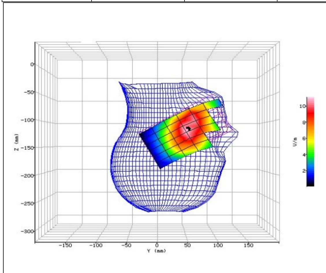
Figure 30: SAR Head Testing Results for the Sharp Smart phone at 709.0MHz.
