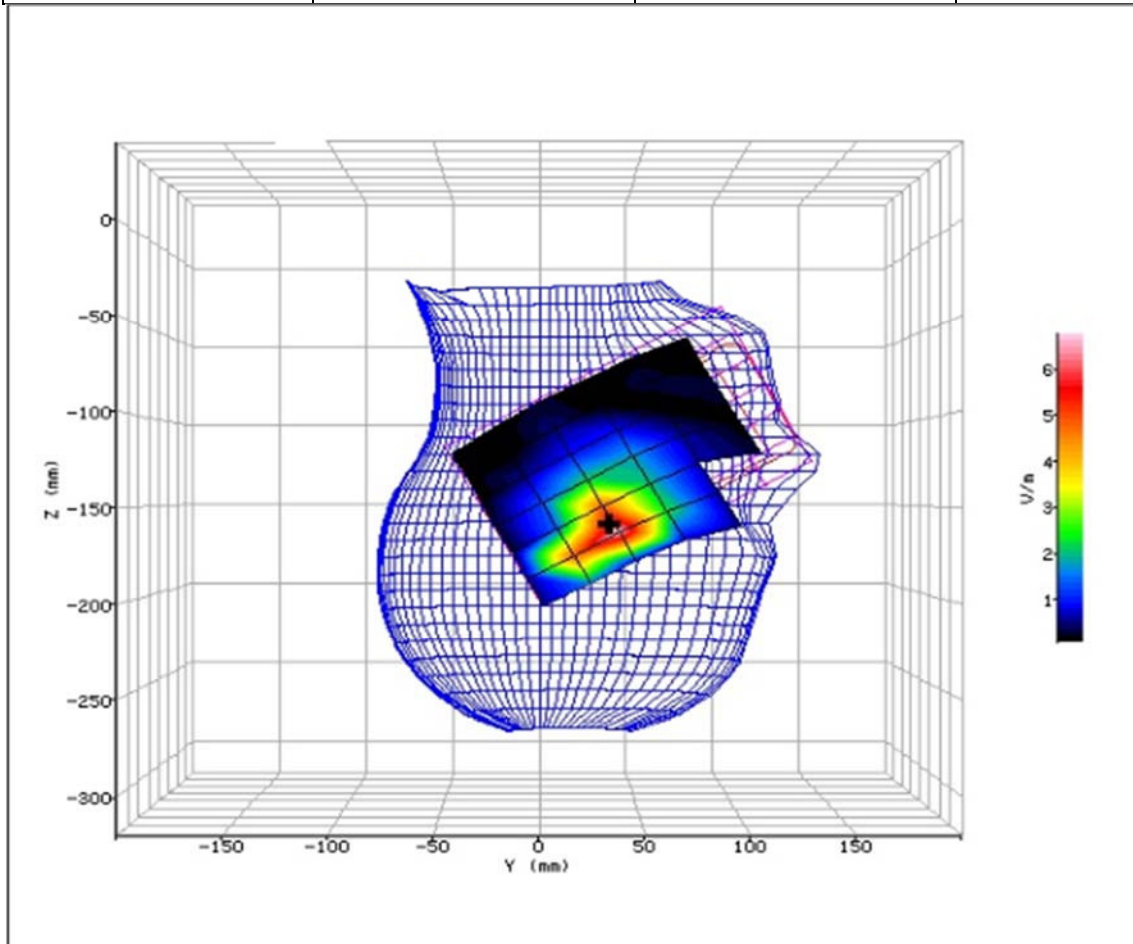
Figure 104: SAR Head Testing Results for the Sharp Smart phone at 2437.0MHz.
