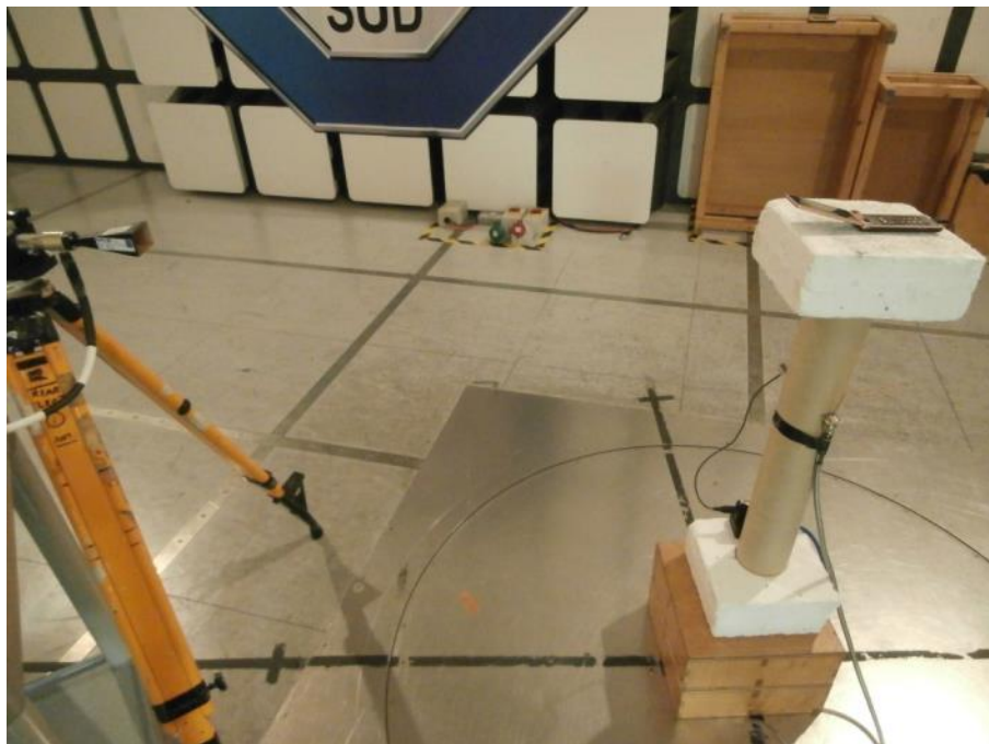
Radiated Emissions 18 GHz to 20 GHz
