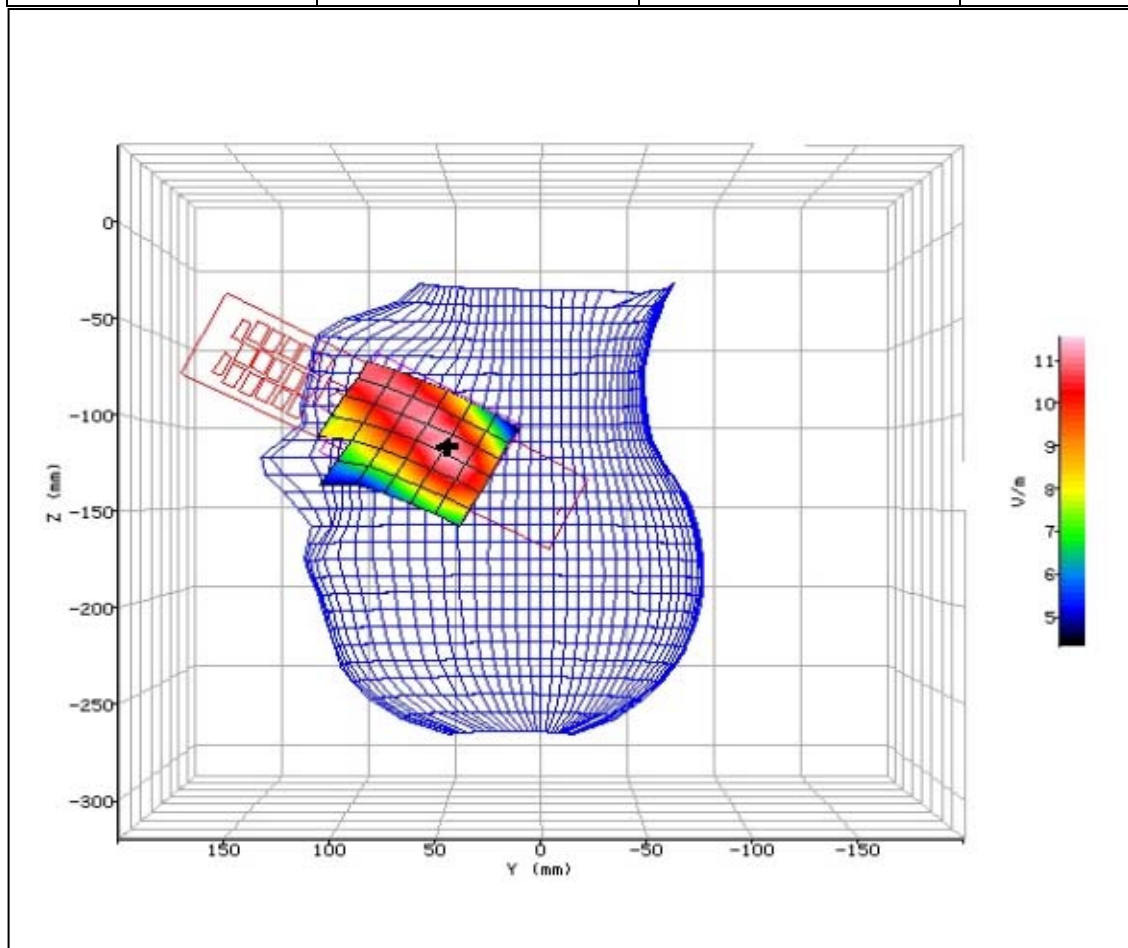
Figure 22: SAR Head Testing Results for the Sharp SHF32 Mobile Handset at 826.4MHz.
