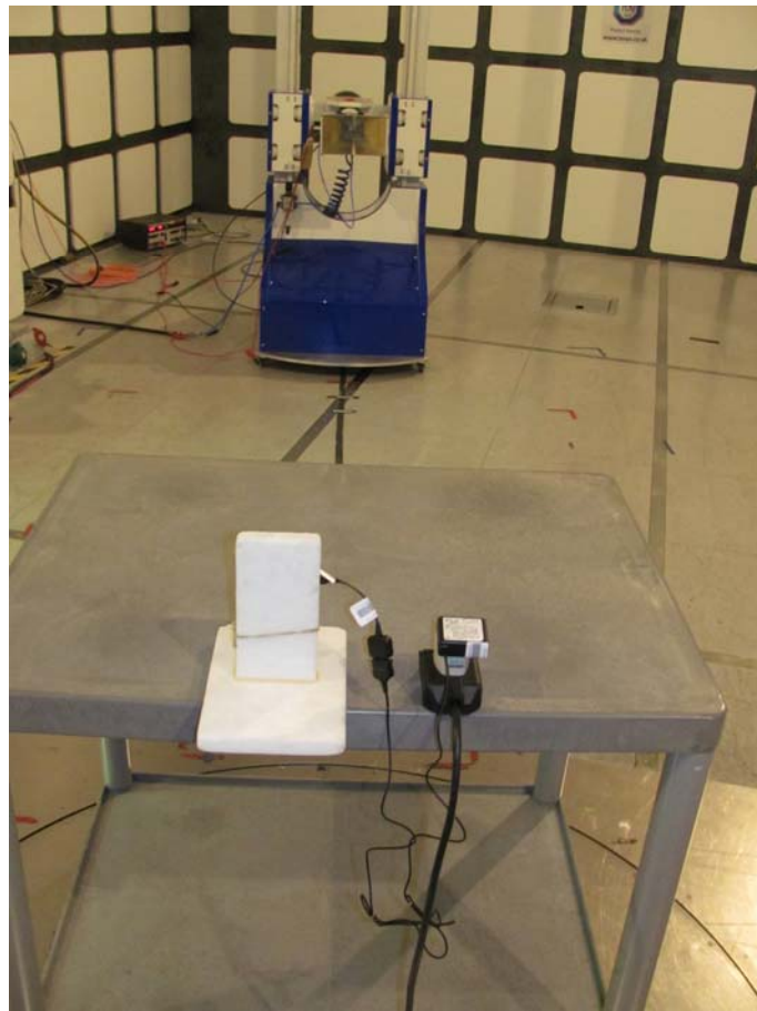
1GHz-13GHz – Radiated Emissions
