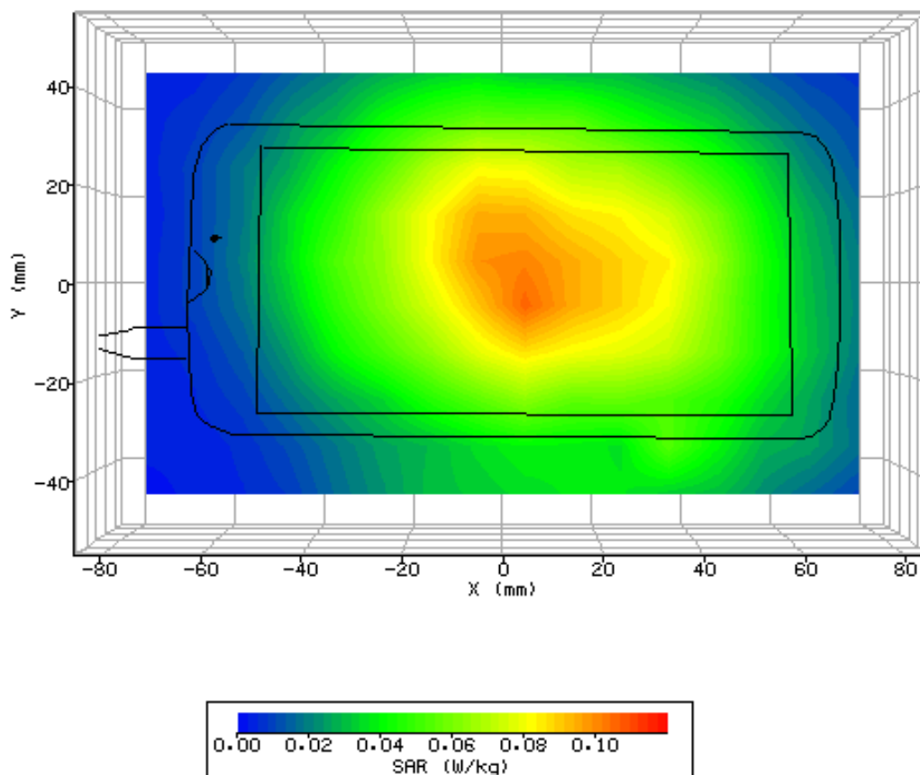
Figure 12: SAR Body Testing Results for the CDMA SHI13 Mobile Handset at 824.7MHz.
