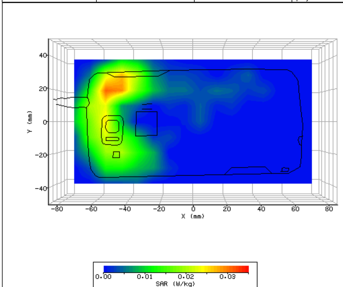
Figure 19: SAR Body Testing Results for the CDMA SHI13 Mobile Handset at 2412MHz.
