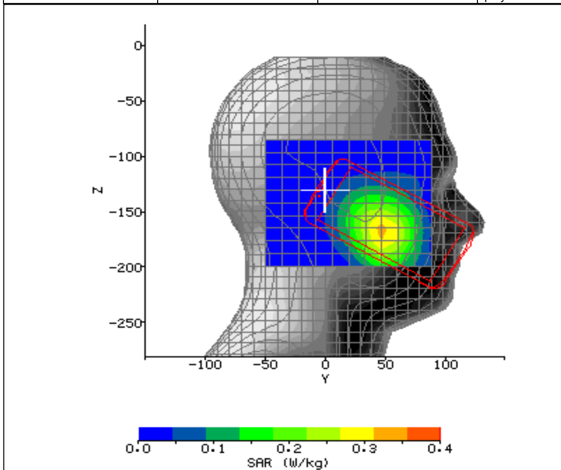
Figure 10: SAR Head Testing Results for the CDMA SHI13 Mobile Handset at 824.7MHz.
