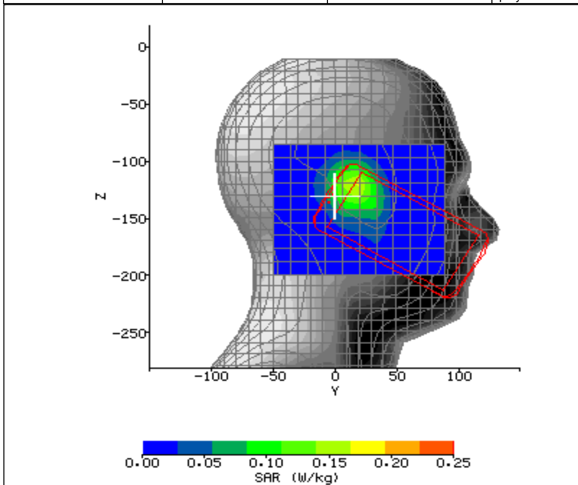
Figure 16: SAR Head Testing Results for the CDMA SHI13 Mobile Handset at 2412MHz.
