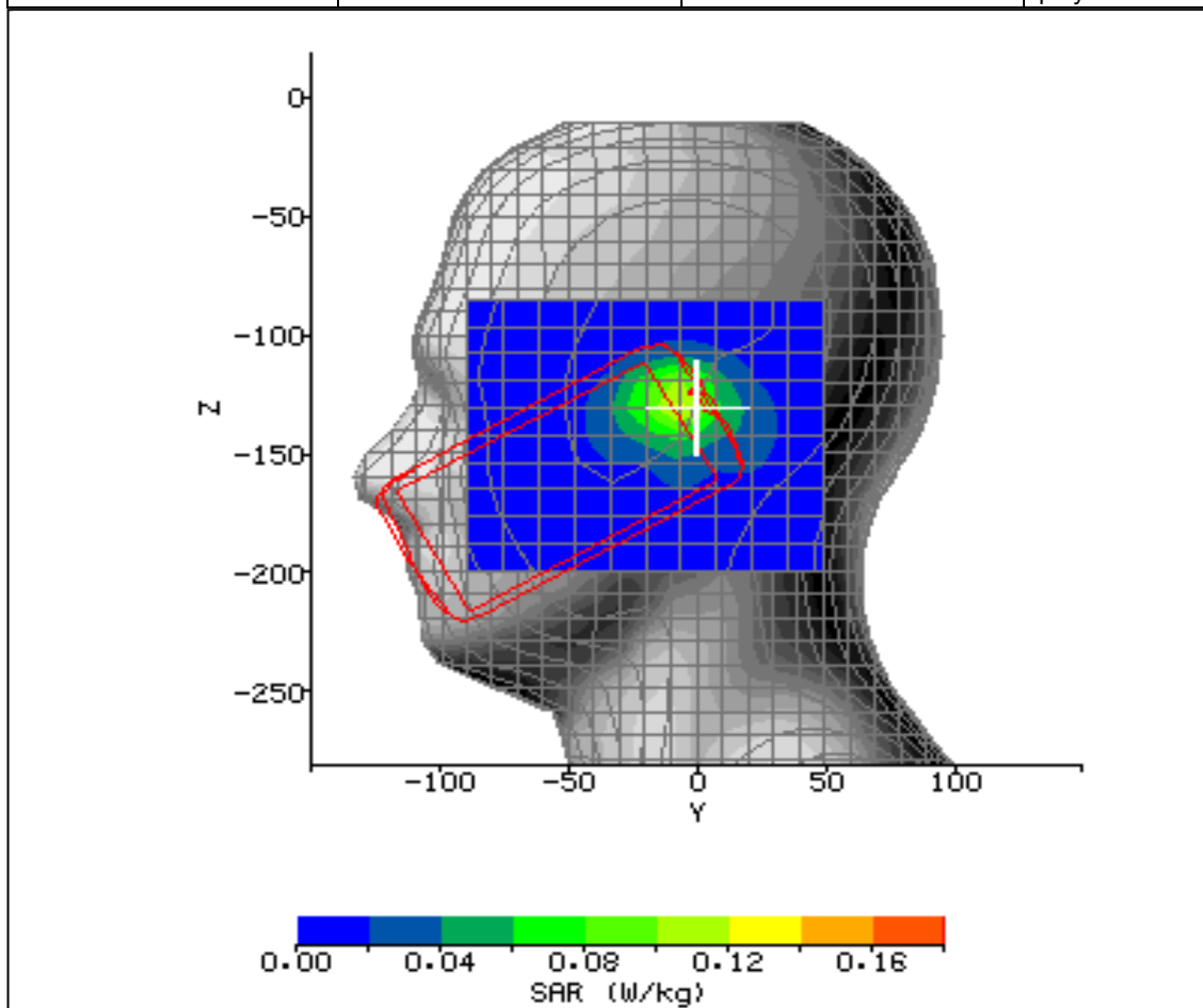
Figure 15: SAR Head Testing Results for the CDMA SHI13 Mobile Handset at 2412MHz.
