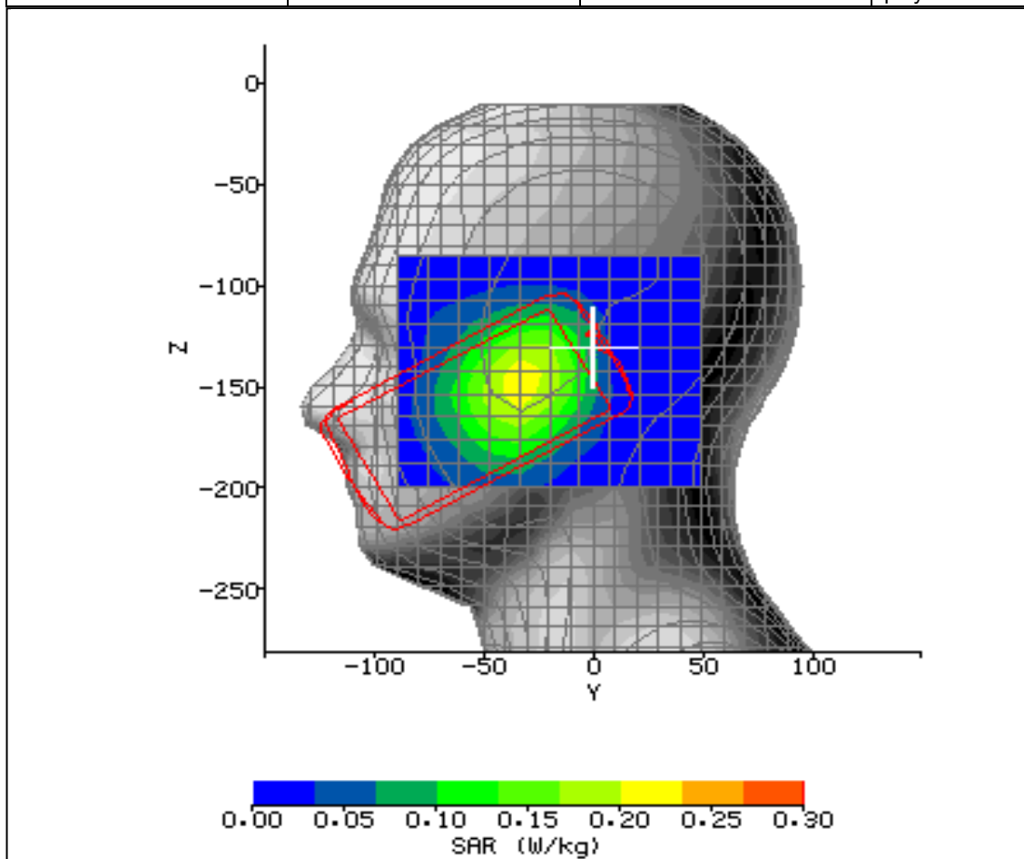
Figure 9: SAR Head Testing Results for the CDMA SHI13 Mobile Handset at 824.7MHz.
