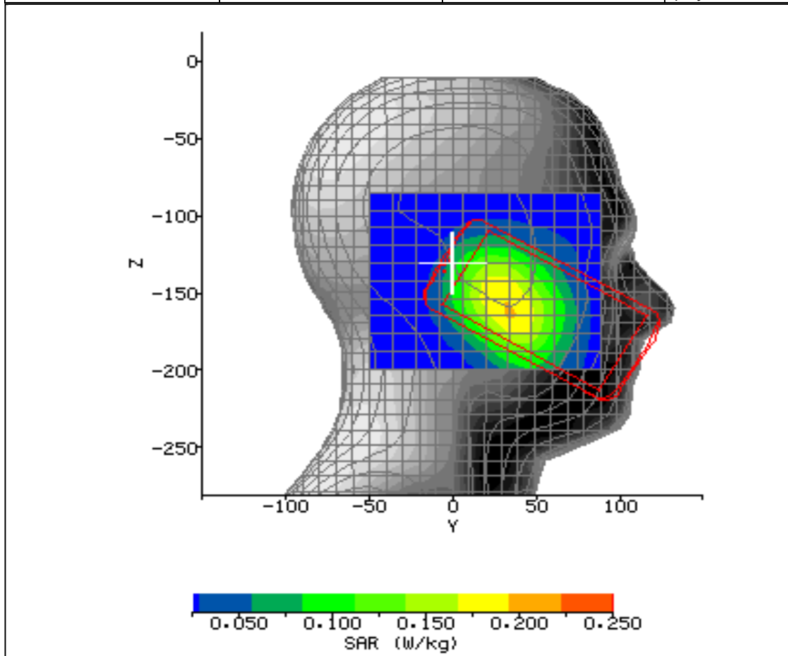
Figure 11: SAR Head Testing Results for the CDMA SHI13 Mobile Handset at 824.7MHz.
