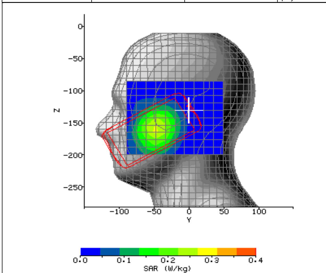
Figure 8: SAR Head Testing Results for the CDMA SHI13 Mobile Handset at 824.7MHz.
