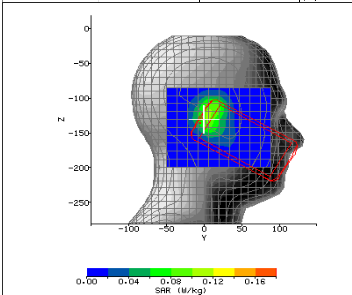
Figure 17: SAR Head Testing Results for the CDMA SHI13 Mobile Handset at 2412MHz.
