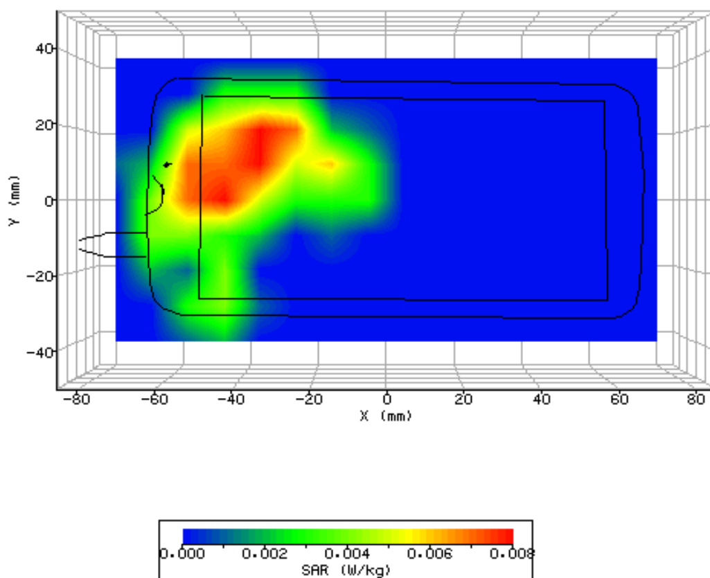
Figure 18: SAR Body Testing Results for the CDMA SHI13 Mobile Handset at 2412MHz.
