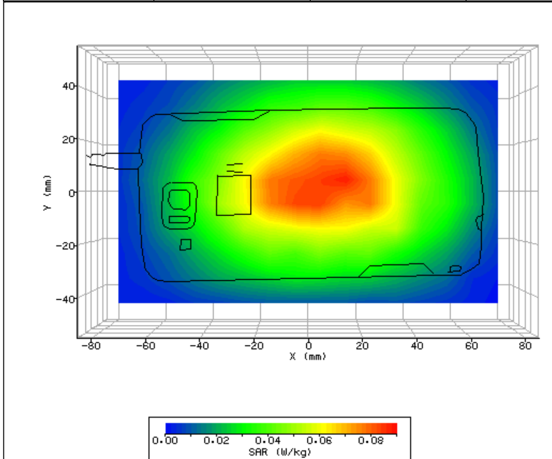
Figure 13: SAR Body Testing Results for the CDMA SHI13 Mobile Handset at 824.7MHz.
