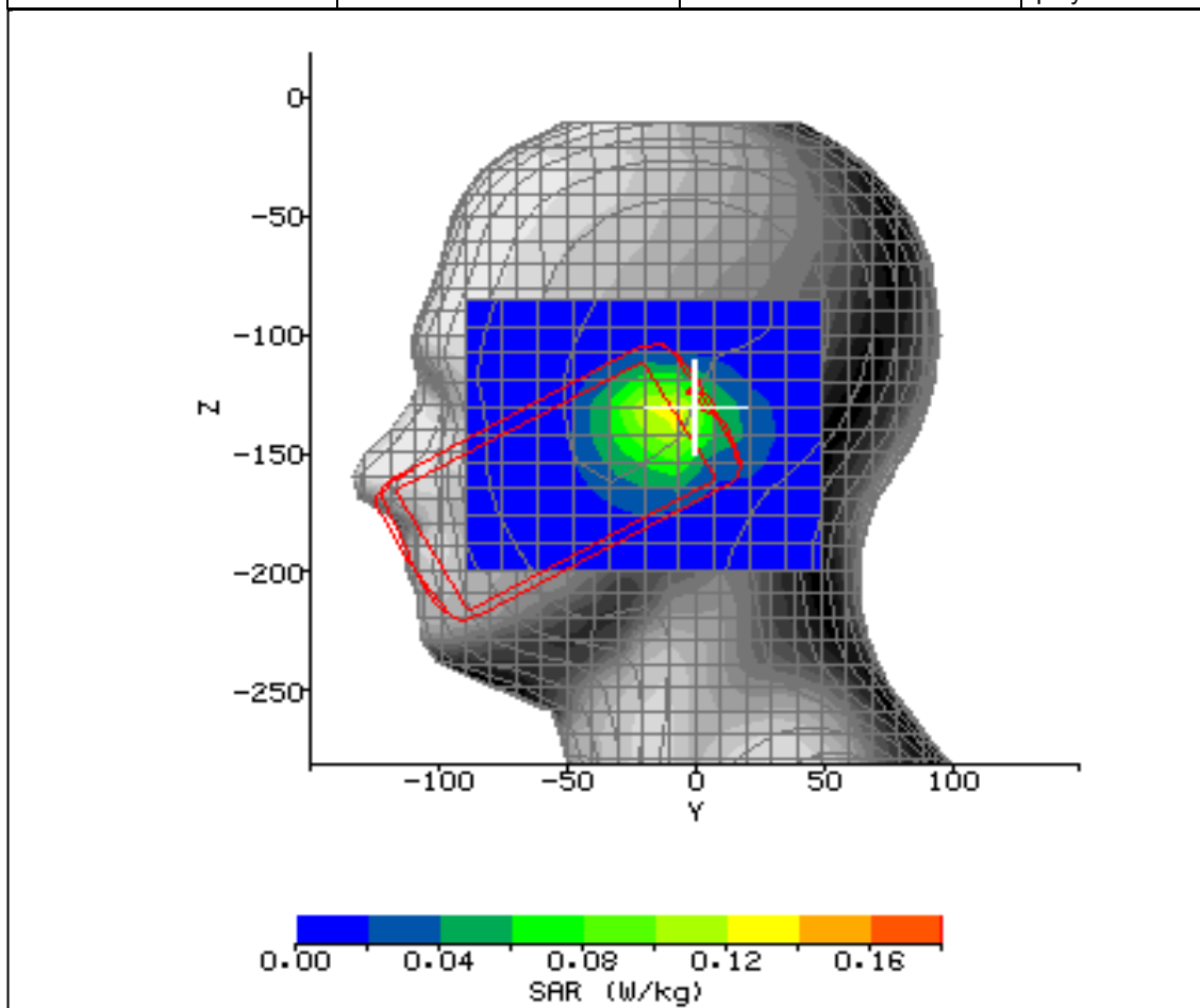
Figure 14: SAR Head Testing Results for the CDMA SHI13 Mobile Handset at 2412MHz.
