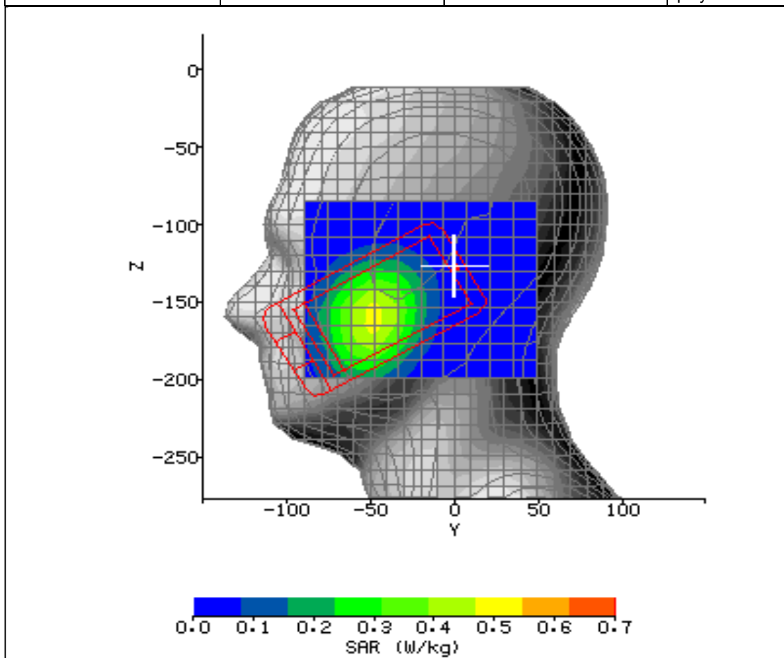
Figure 8: SAR Head Testing Results for the CDMA SHX11 Mobile Handset at 836.52MHz.
