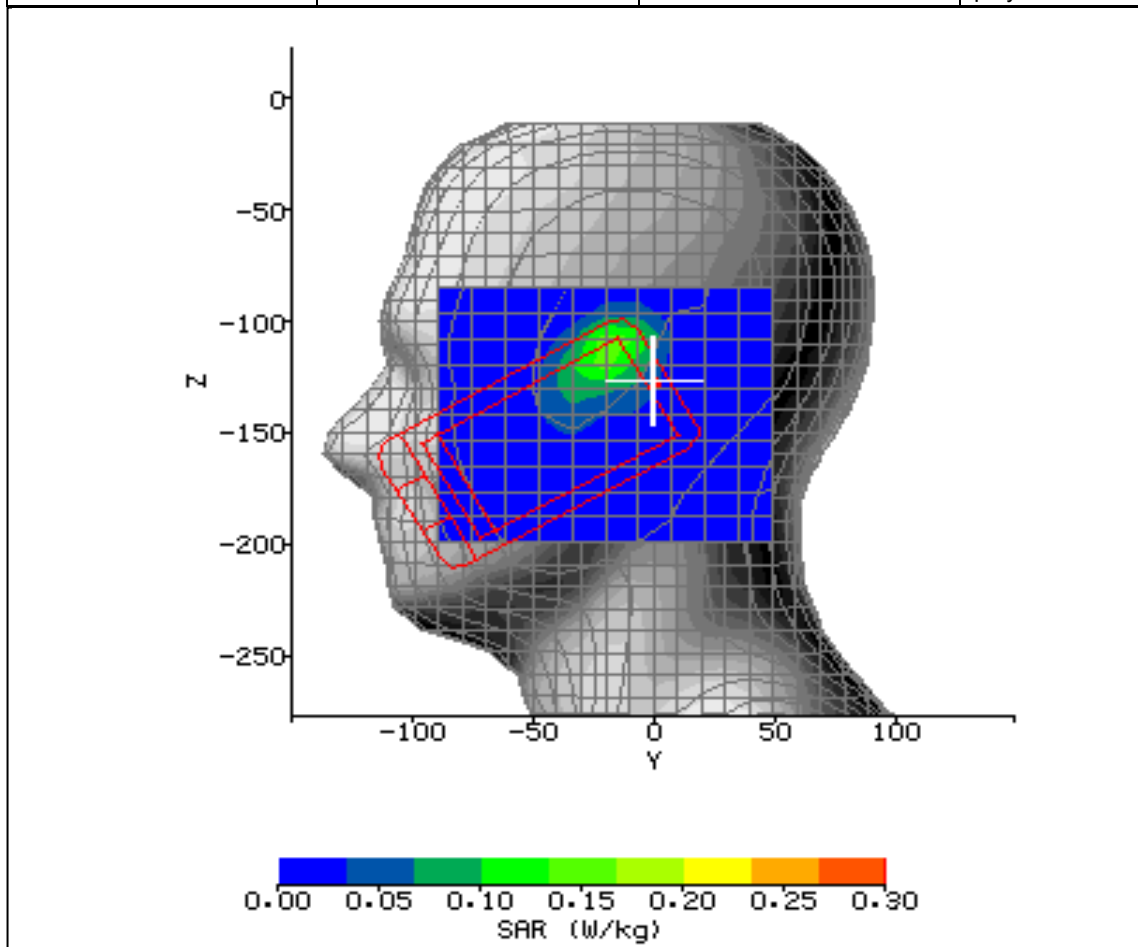
Figure 20: SAR Head Testing Results for the CDMA SHX11 Mobile Handset at 2437.0MHz.
