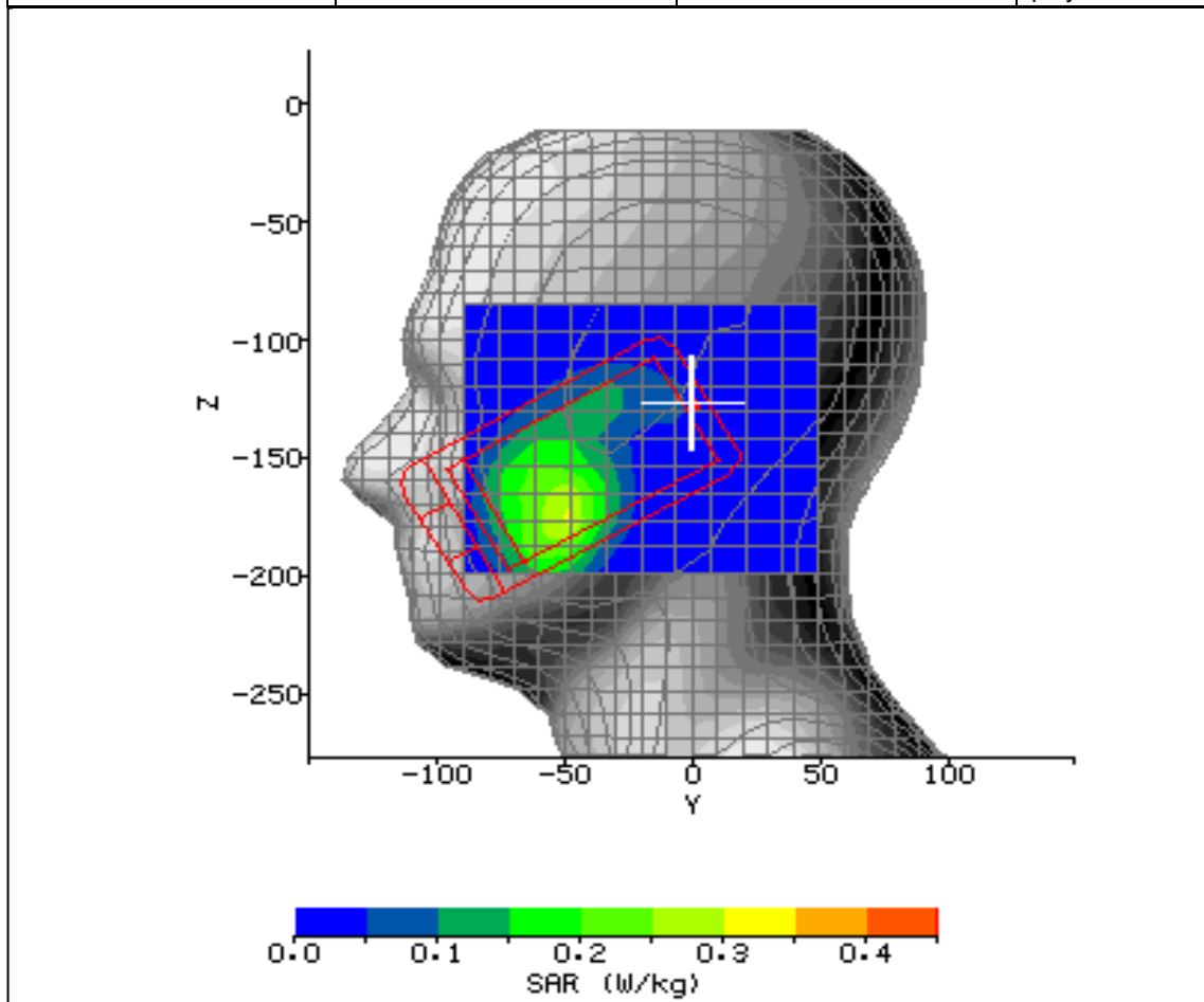
Figure 14: SAR Head Testing Results for the CDMA SHX11 Mobile Handset at 1909.8MHz.
