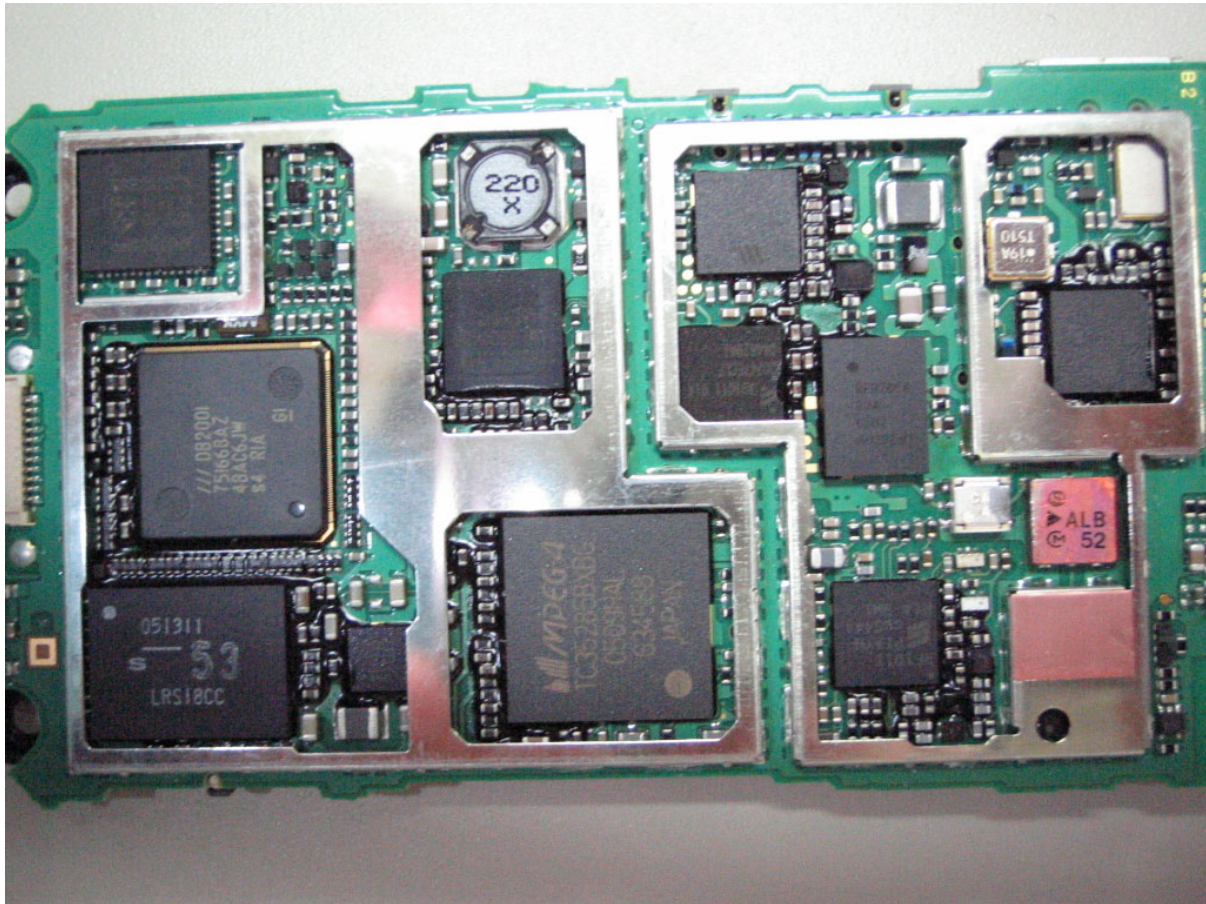
Inside (Shield)
