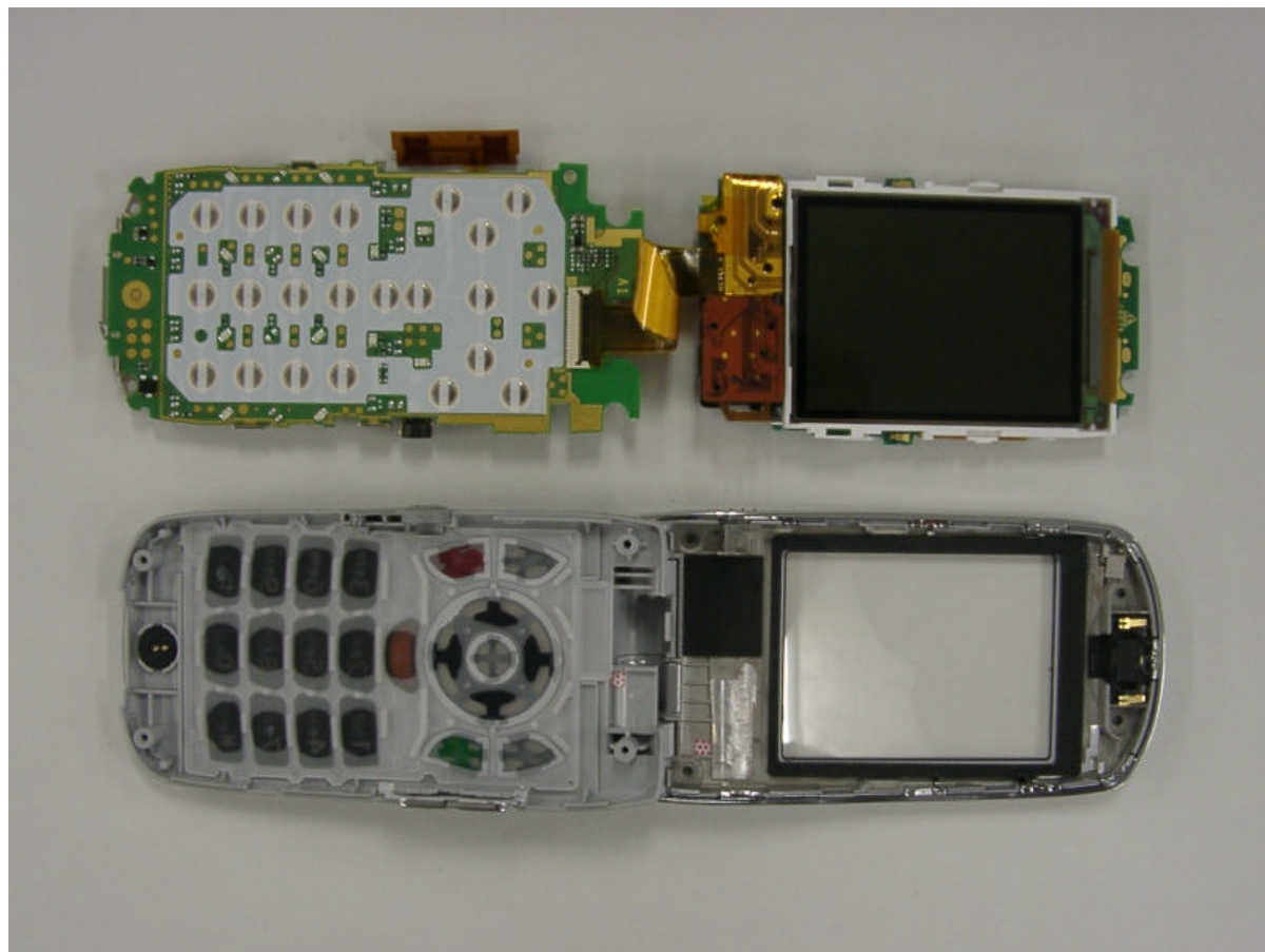
GX30 Photo(Internal)
