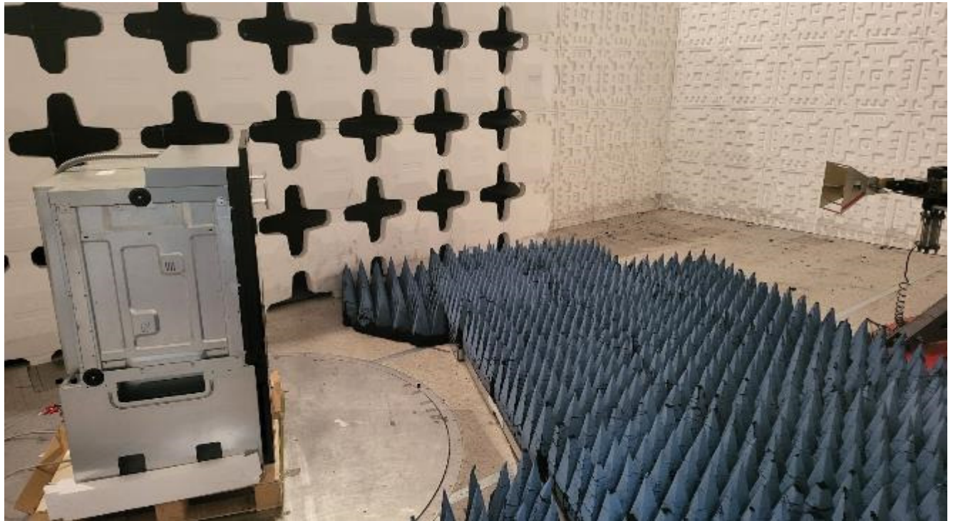
Figure 12. Photograph of Radiated Emissions Test Configuration, above 1000 MHz
