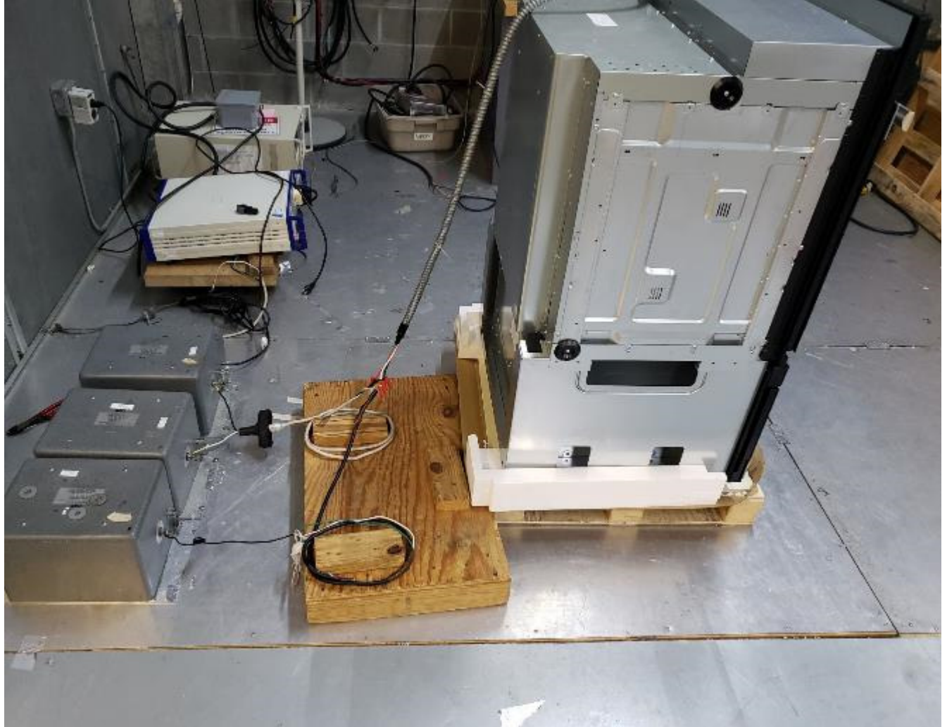
Figure 8. Photograph of Conducted Emissions Test Configuration
