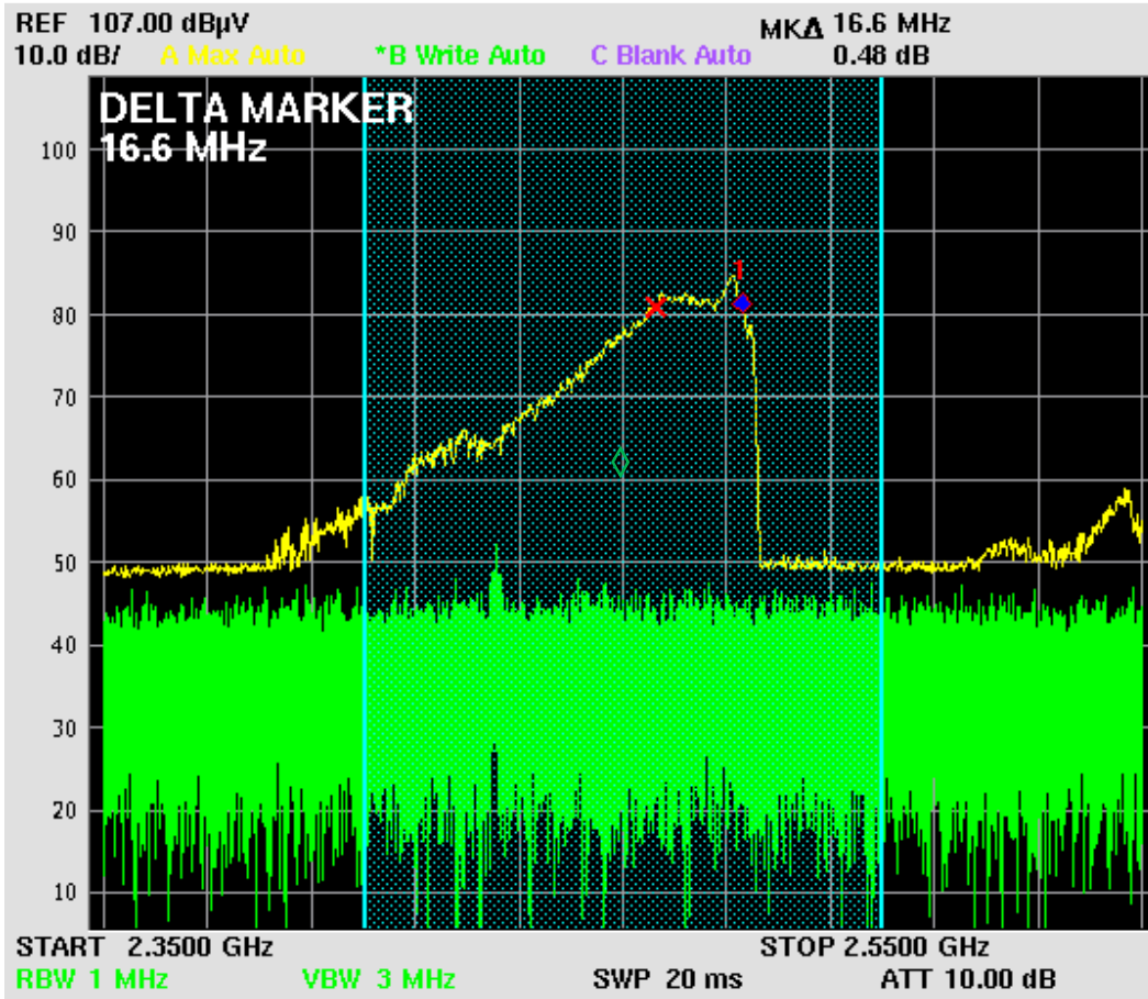
Figure 13. Frequency Variation at Nominal Voltage
