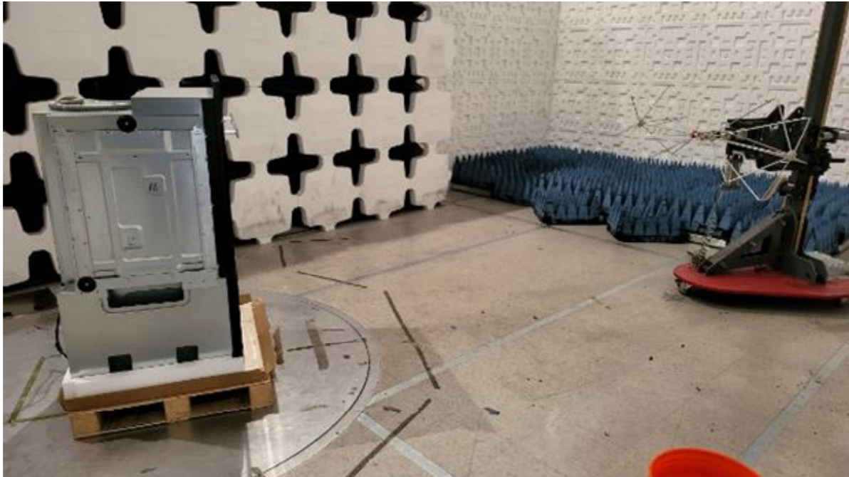
Figure 10. Photograph of Radiated Emissions Test Configuration, 30 - 200 MHz
