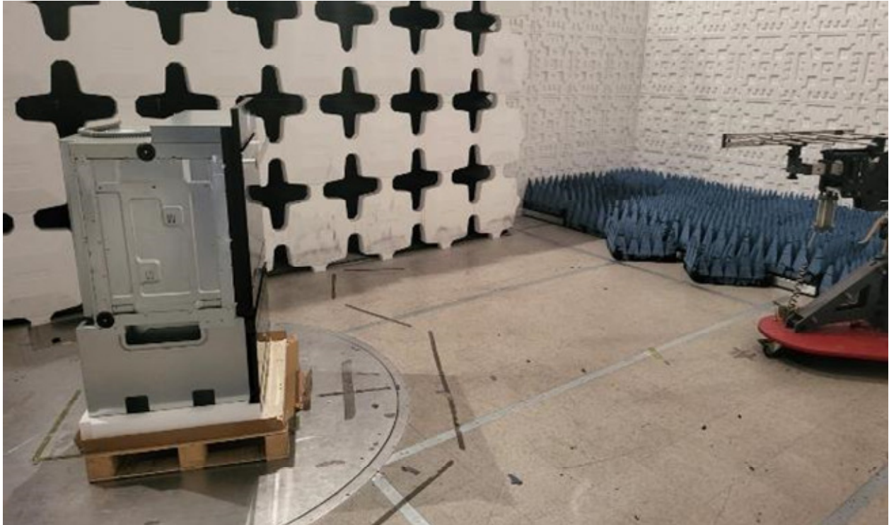
Figure 11. Photograph of Radiated Emissions Test Configuration, 200 - 1000 MHz
