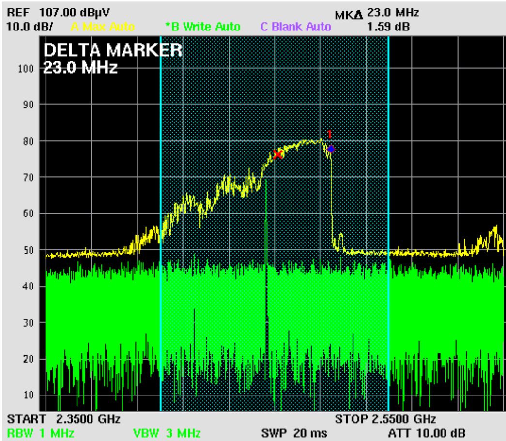
Figure 15. Frequency Variation at High Voltage
