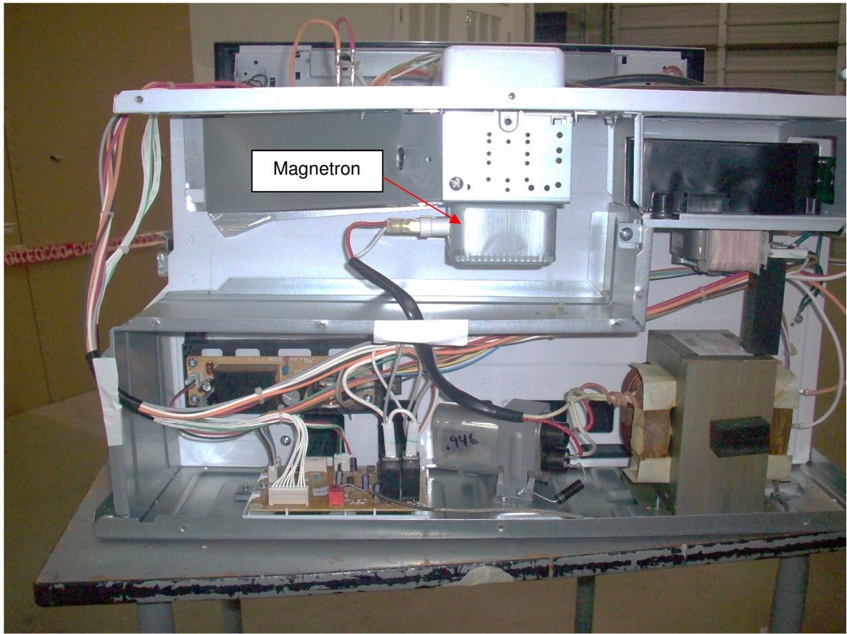
Figure 3. Rear View
