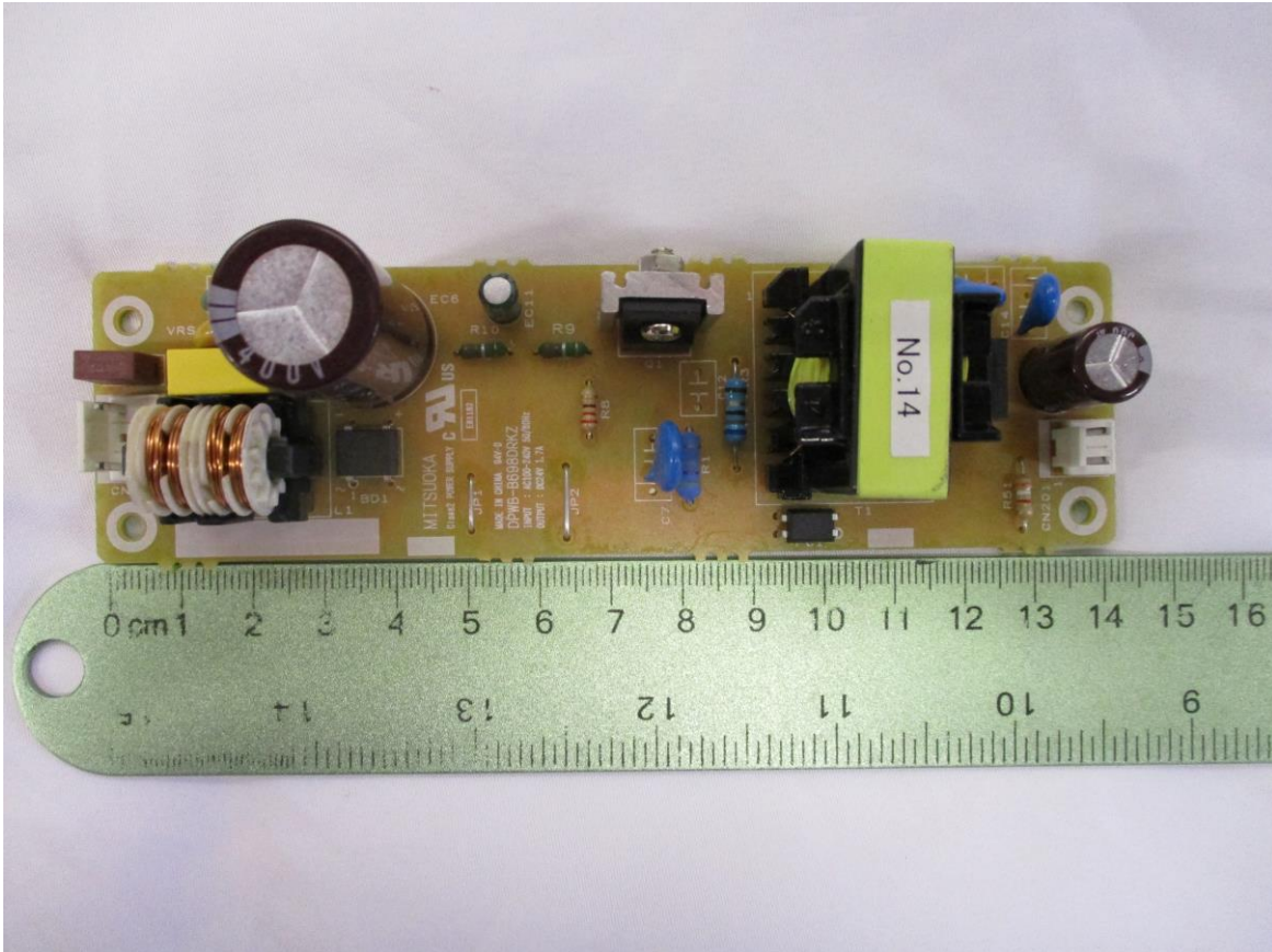
Figure 5. Mitsuoka Switching Power Supply- Top Side
