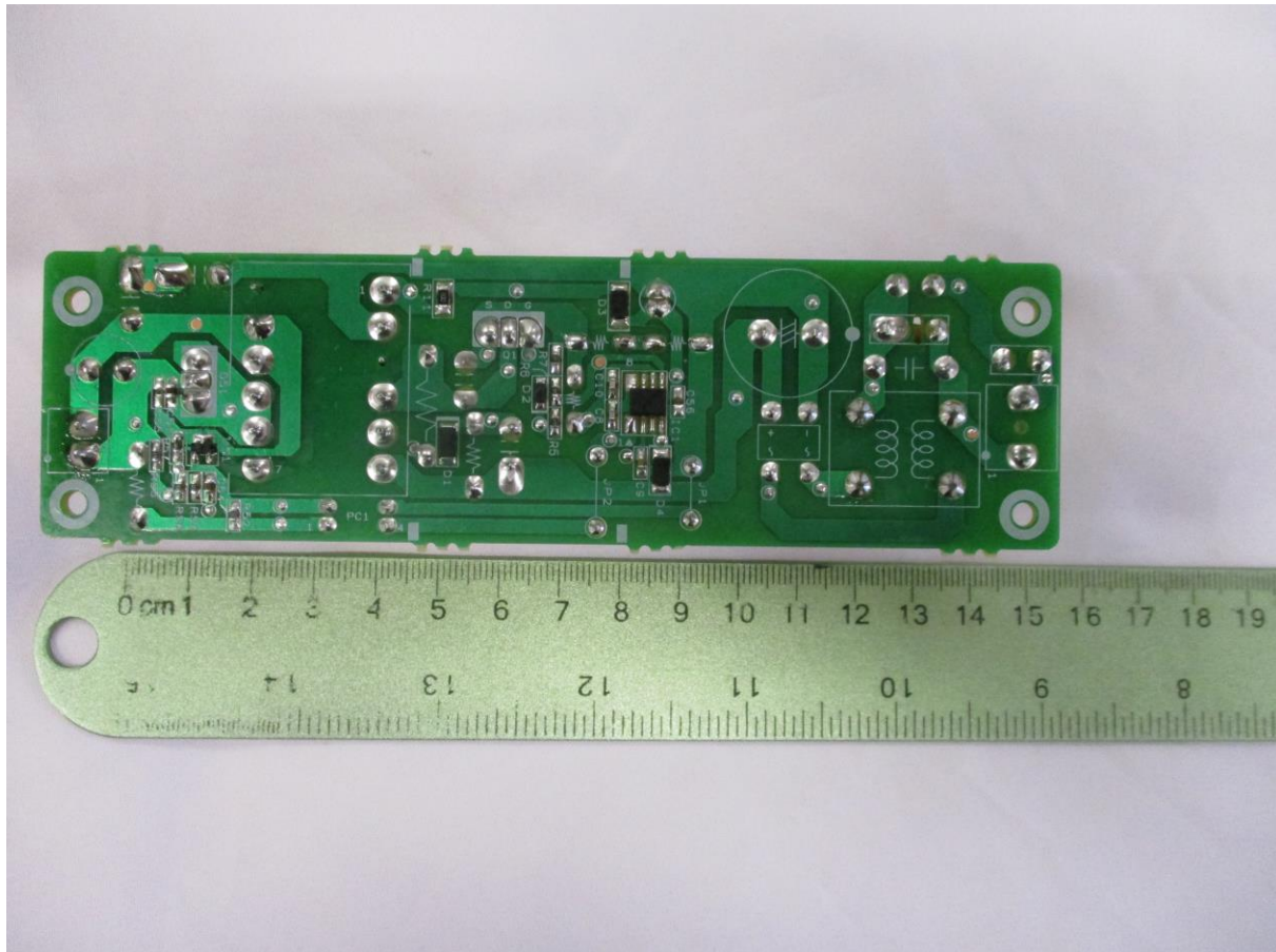
Figure 6. Mitsuoka Switching Power Supply- Bottom Side
