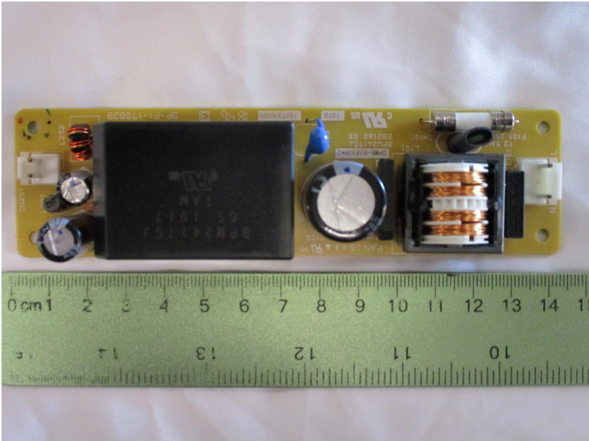
Figure 7. Tamura Switching Power Supply- Top Side
