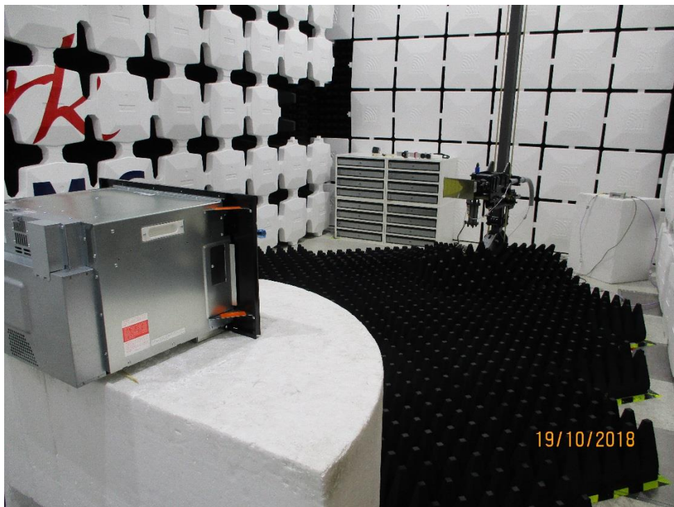
Radiated electric field emissions > 1GHz
