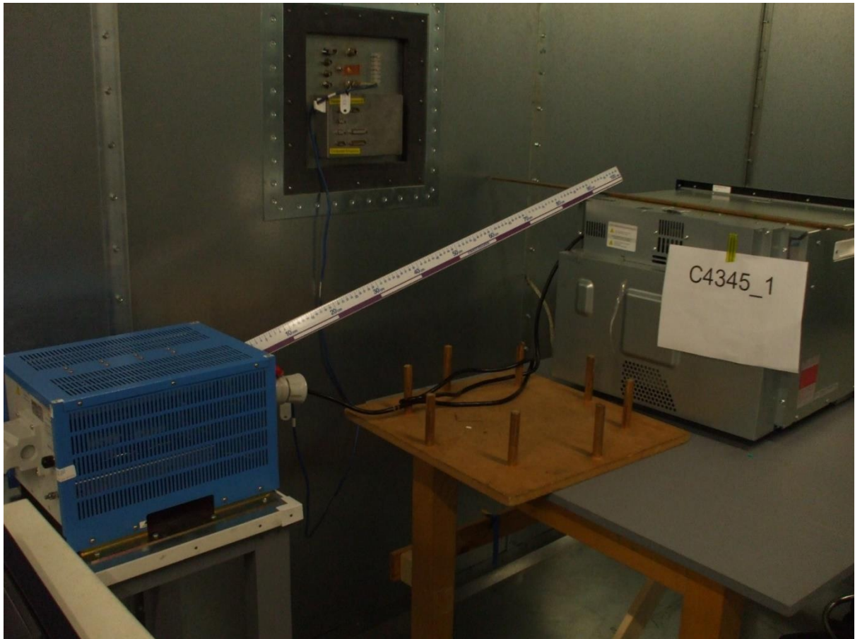
Mains conducted Emissions
