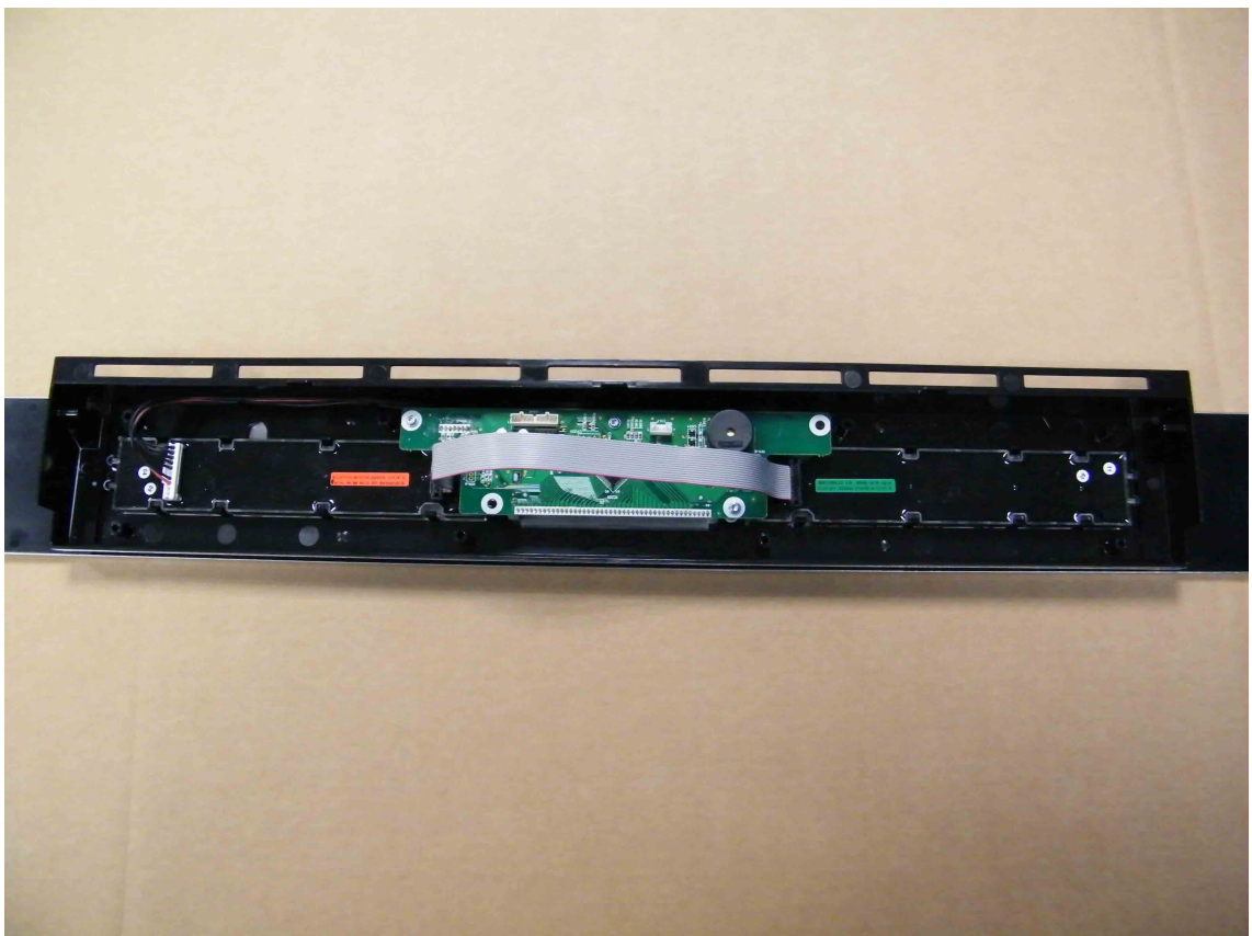
STAINLESS CONTROL PANEL WITH REAR COVER REMOVED
