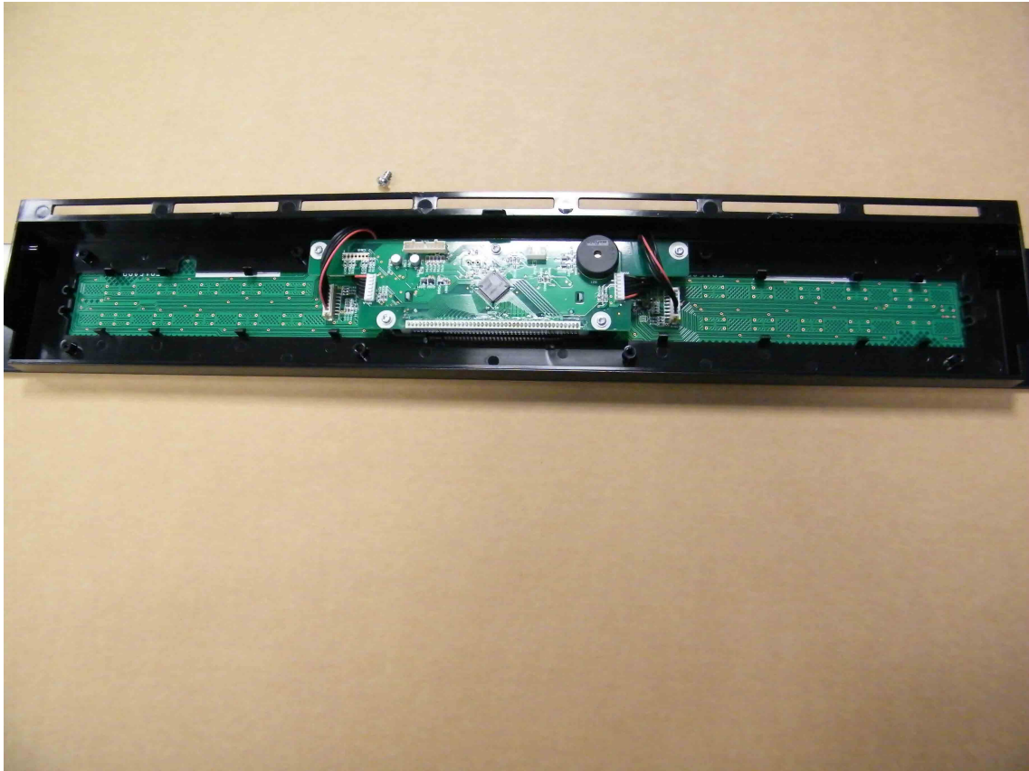
GLASS CONTROL PANEL WITH REAR COVER REMOVED
