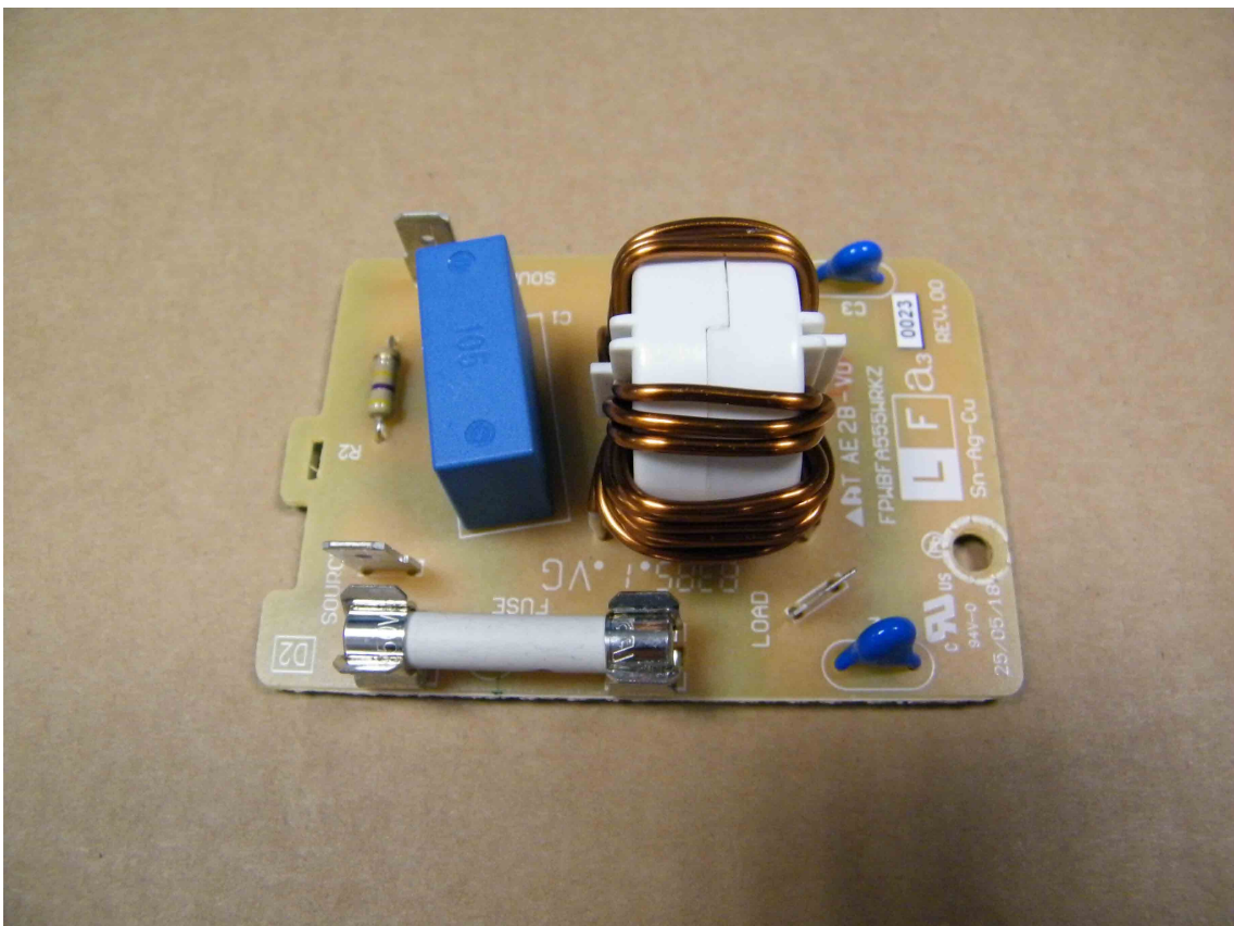
NOISE FILTER UNIT
