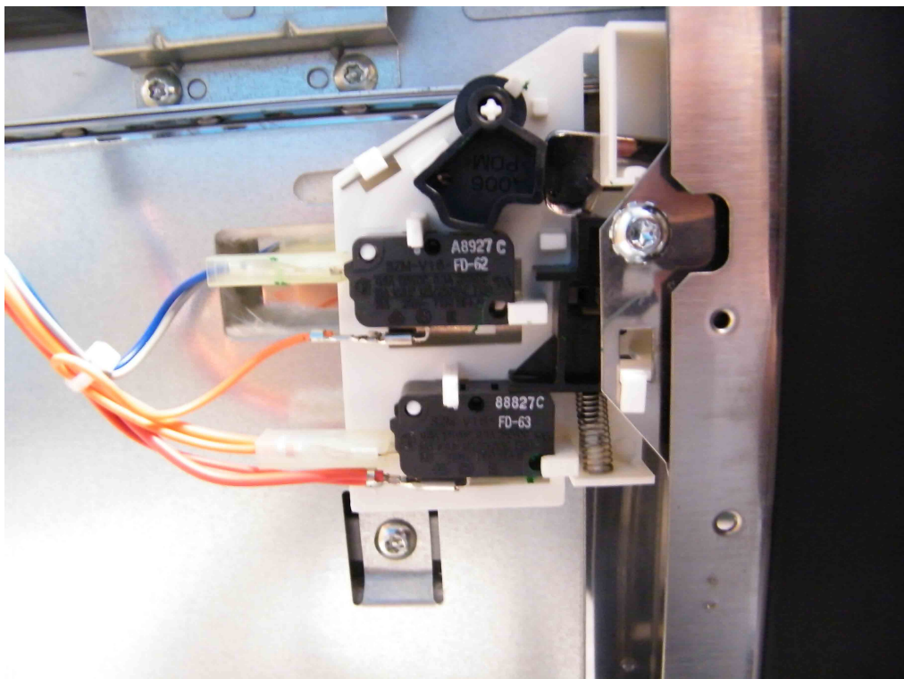
LEFT SIDE LATCH ASSEMBLY
