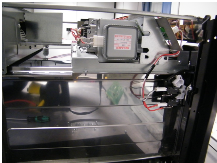
Internal - Left Side View
