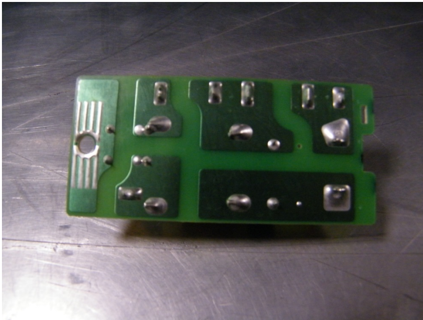
PWB - Noise Filter Unit Rear View
