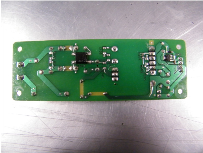
Power Module - Rear View
