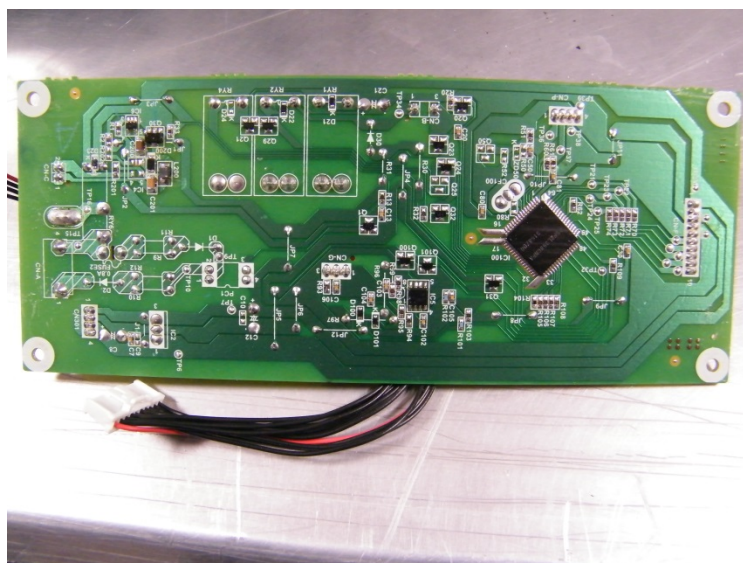
PWB - Control Unit Rear View
