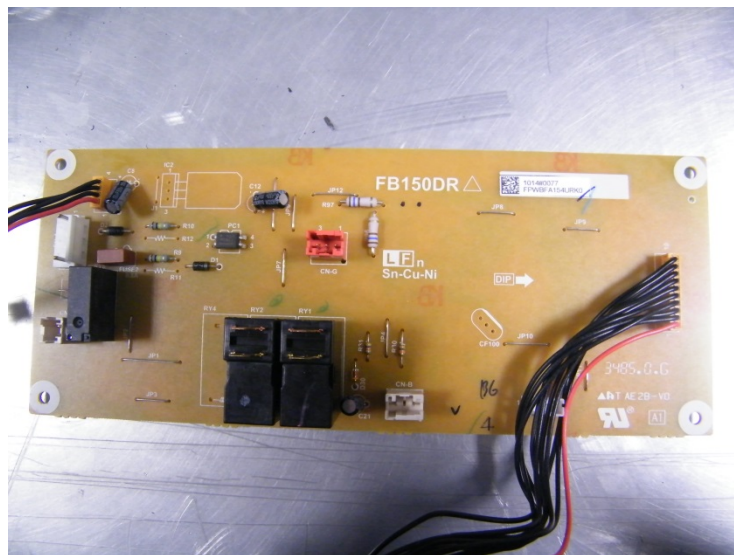
PWB - Control Unit Front View
