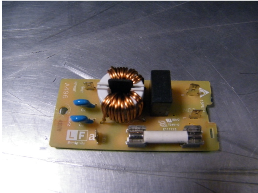
PWB - Noise Filter Unit Front View
