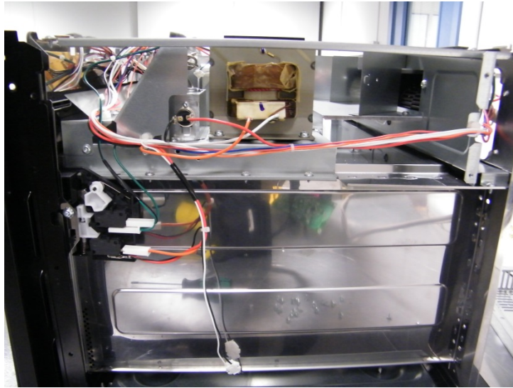
Internal - Right Side View
