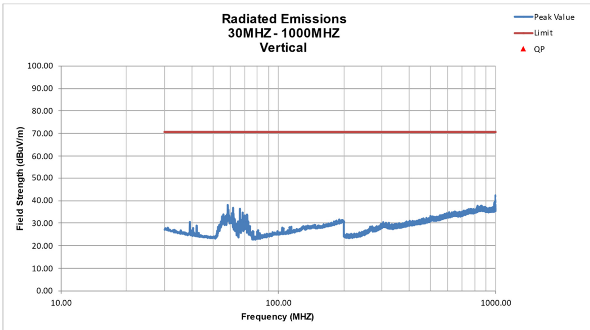
Figure 5. Radiated Emissions Below 30-1000 MHz Vertical
