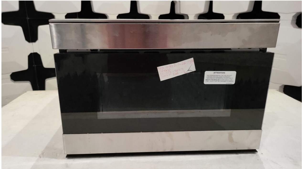
Figure 9. Photograph of Radiated Emissions Test Configuration, Close-Up
