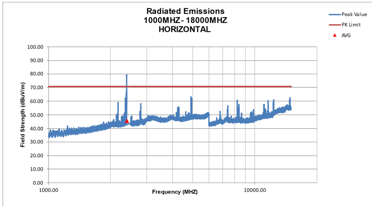
Figure 6. Radiated Emissions Above 1 GHz Horizontal
