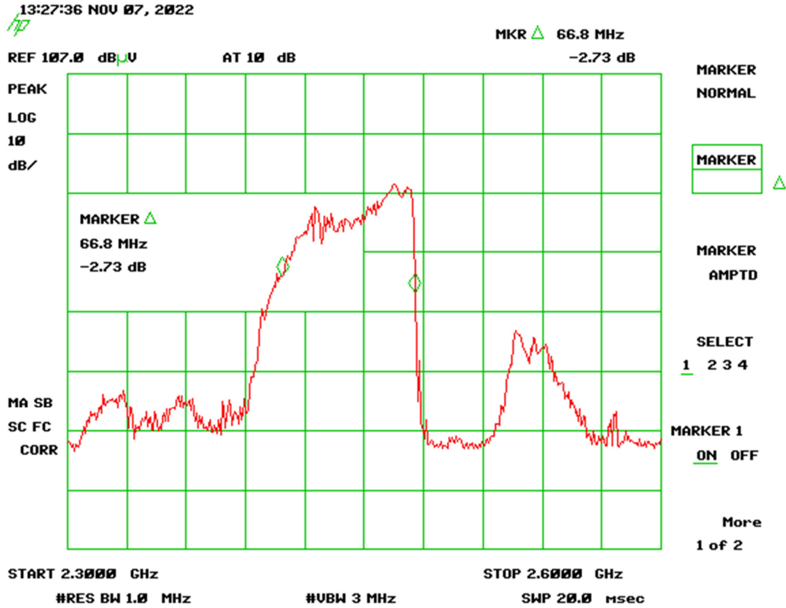
Figure 14. Frequency Variation at Low Voltage
