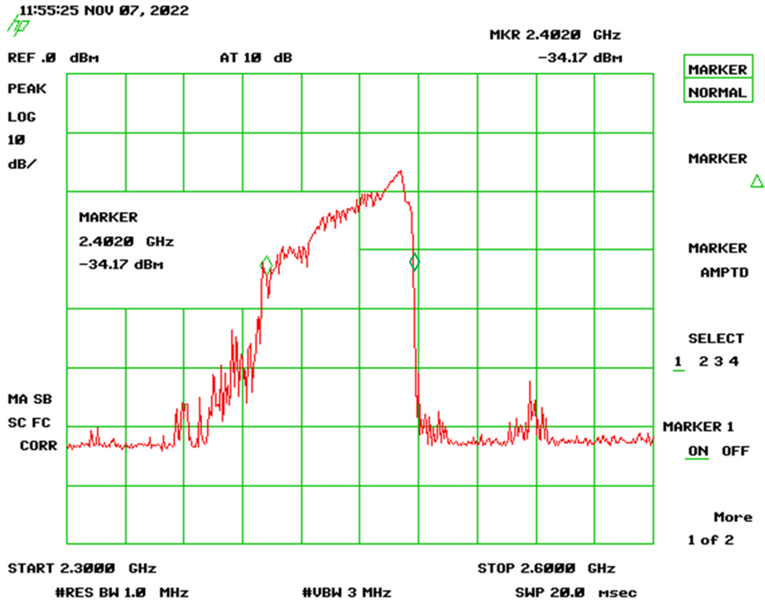
Figure 13. Frequency Variation at Nominal Voltage
