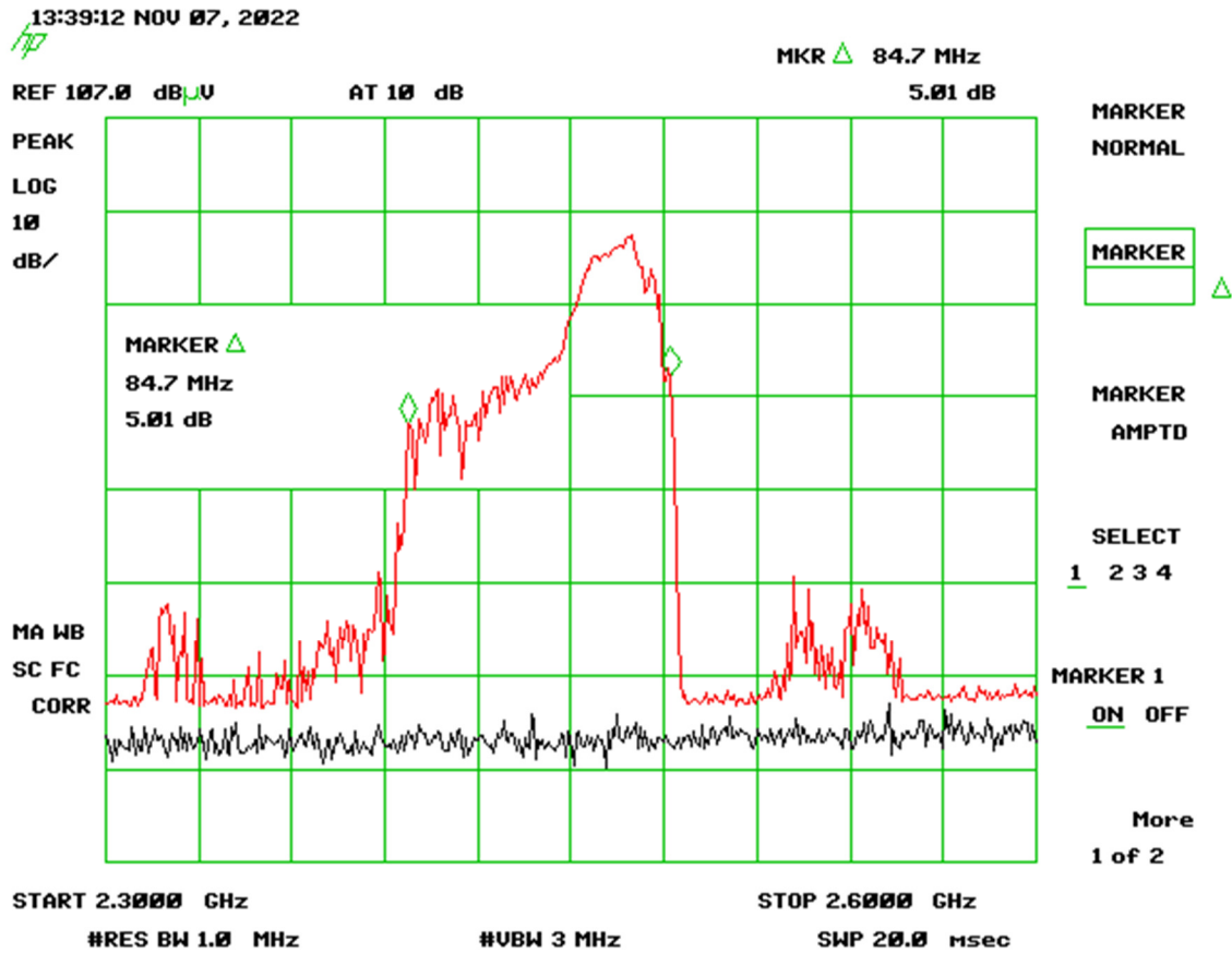
Figure 15. Frequency Variation at High Voltage
