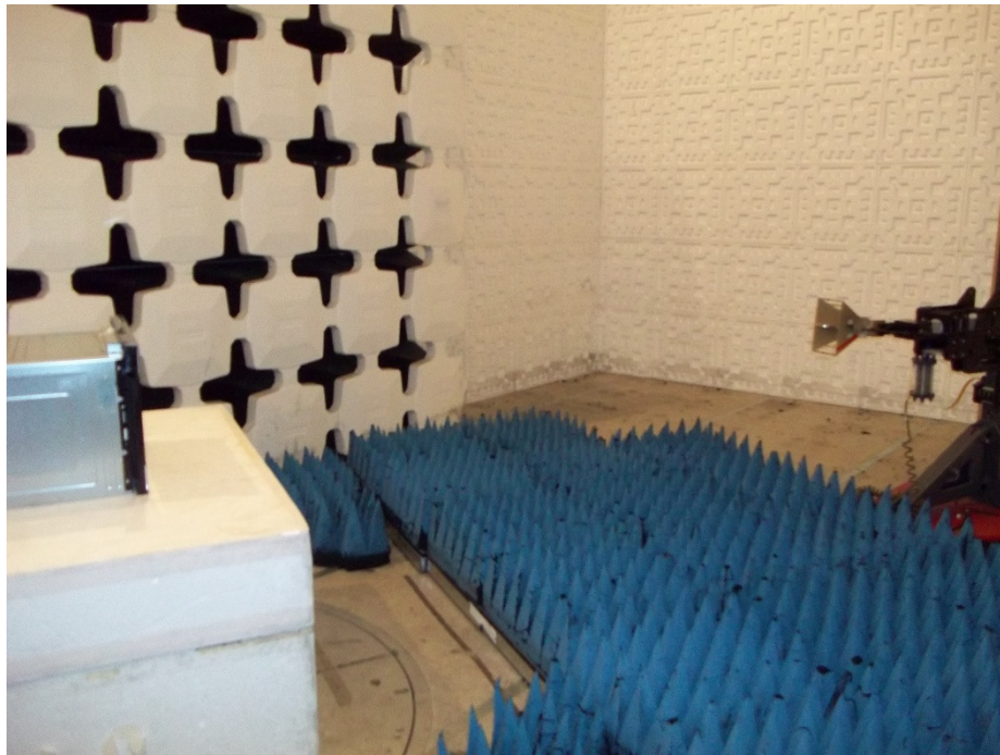
Figure 12. Photograph of Radiated Emissions Test Configuration, above 1000 MHz
