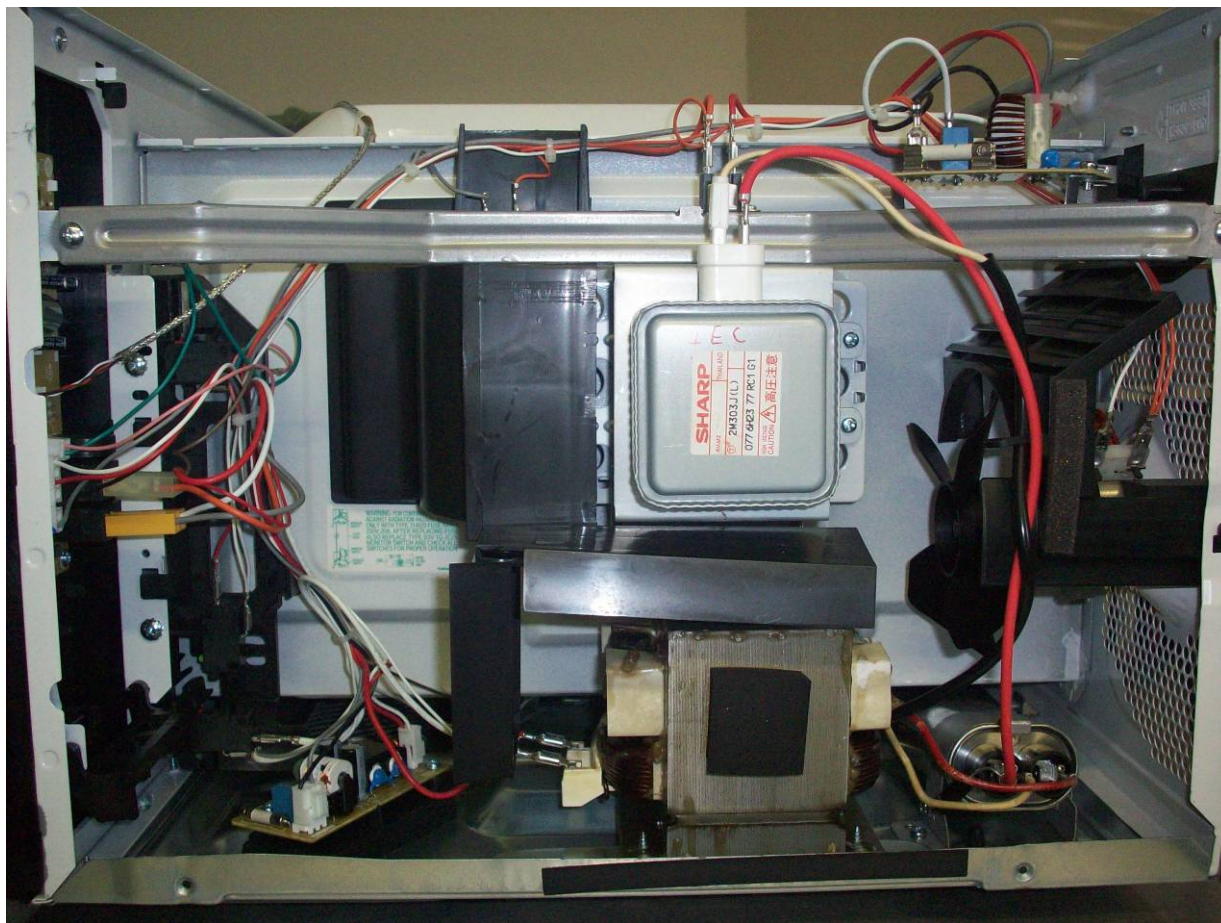
Figure 2. Magnetron Location
