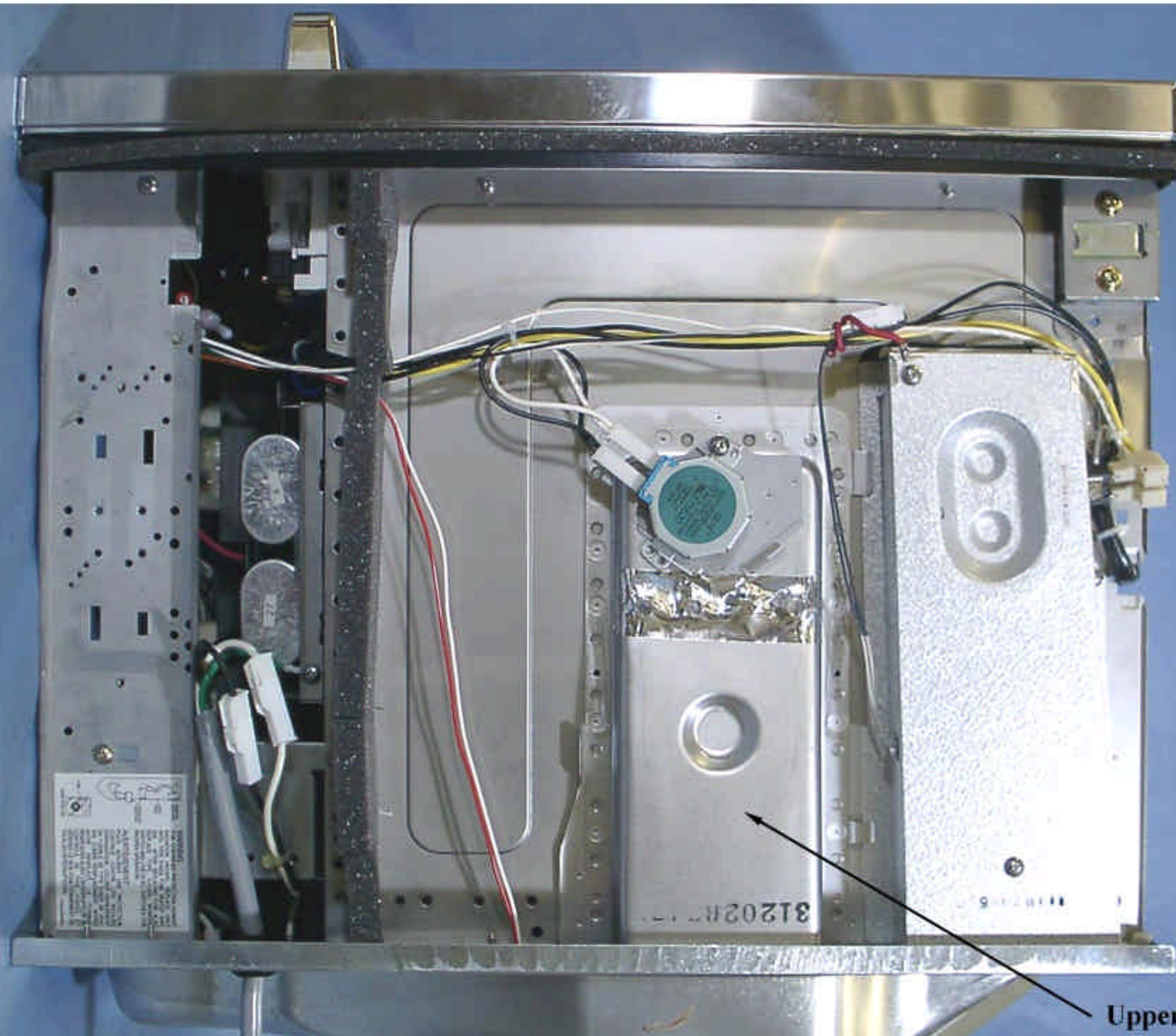
Phot.-05 APYDMR0145 Shows a top view of model R-22JT with outer enclosure removed. And shows upper waveguide location.
